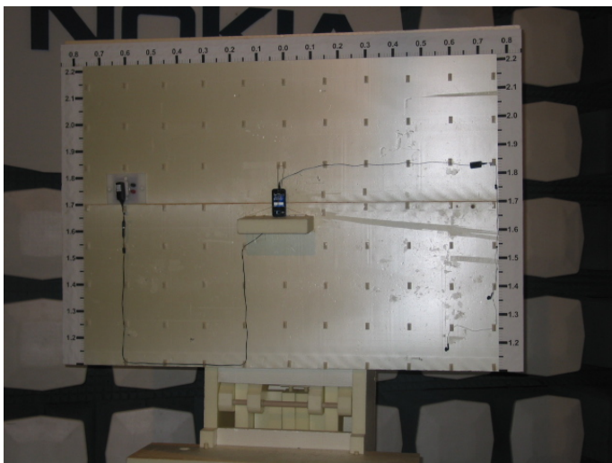
Picture 2 RF Output power measurement, Flip closed
