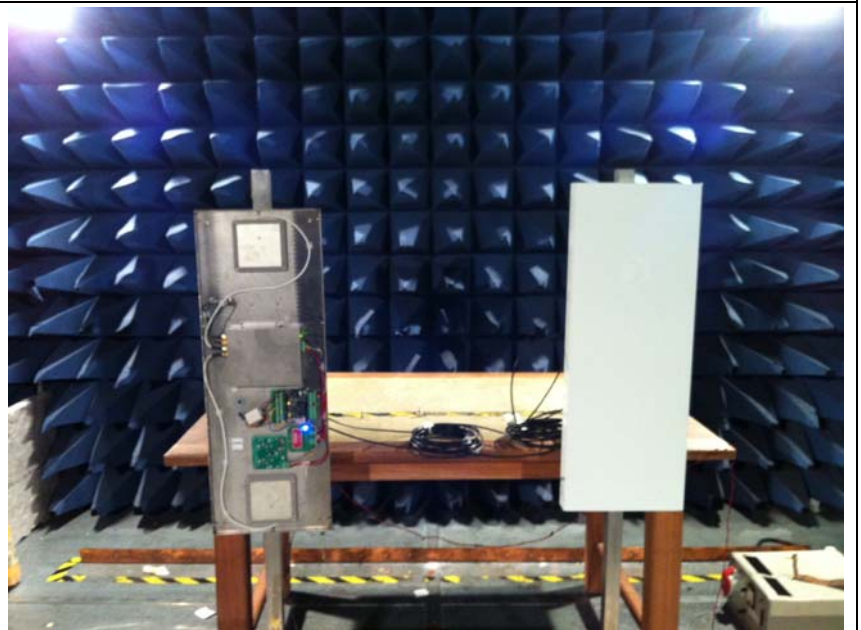
Unwanted emissions: Pre measurement (main unit + deported antennas)
