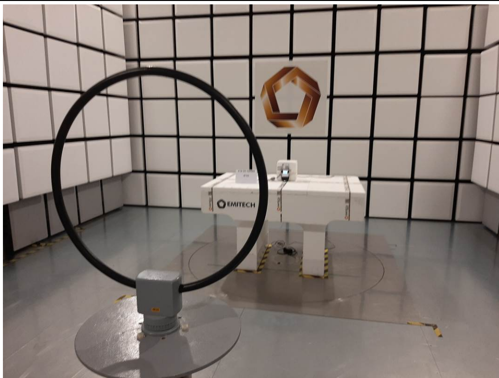
TEST SETUP PHOTO(S) RADIATED EMISSION(F<30MHZ, PRE MEASUREMENT)
