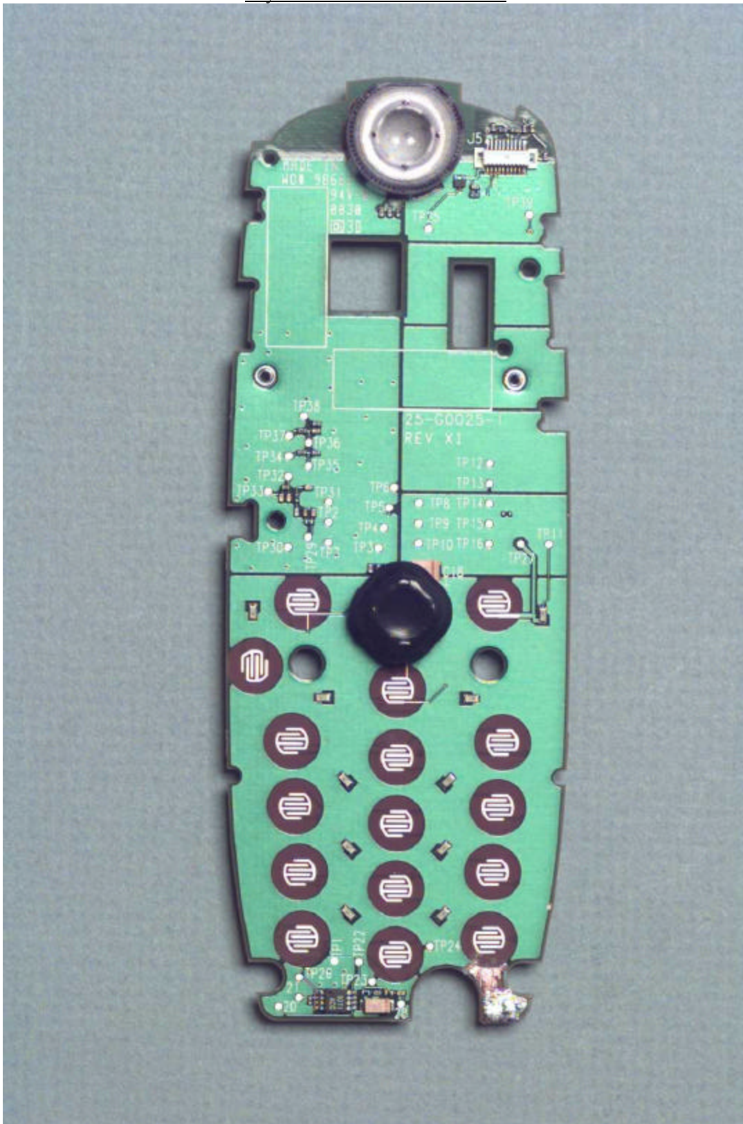
Keyboard PWB Front without LCD
