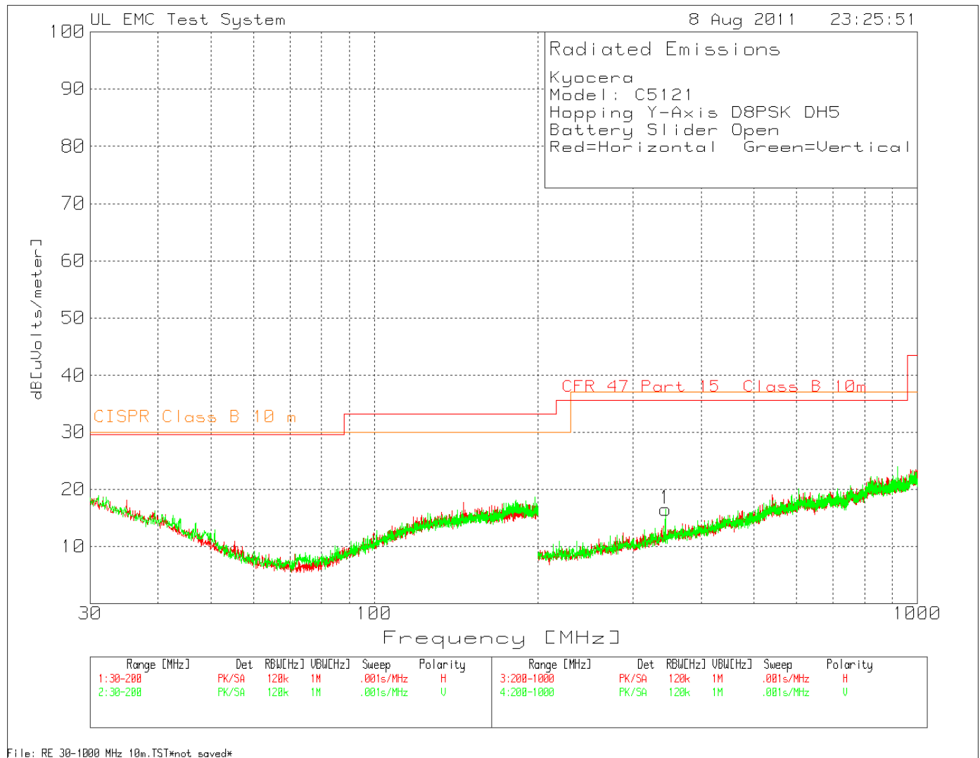
Figure 6 Radiated Emissions Graph Hopping Channel DH5 8PSK
