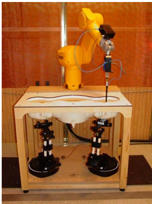
Figure 7.1 DASY 4 System
