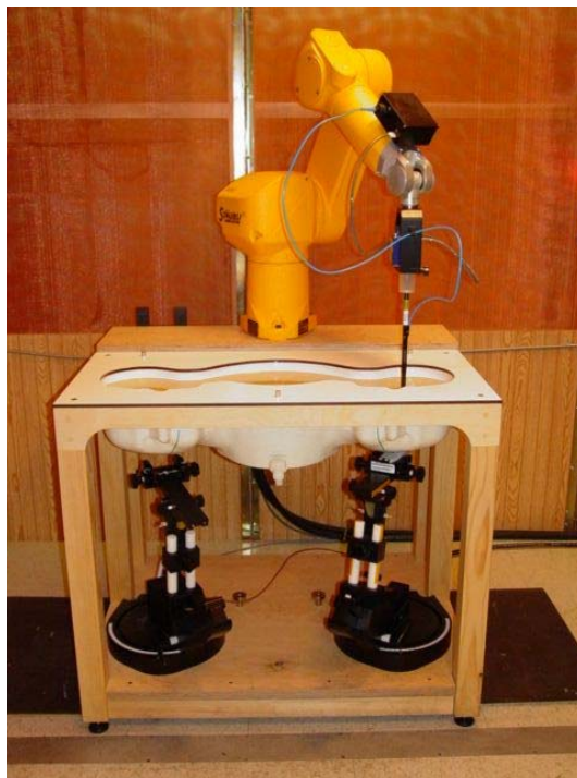
Figure 7.1 DASY 4 System
