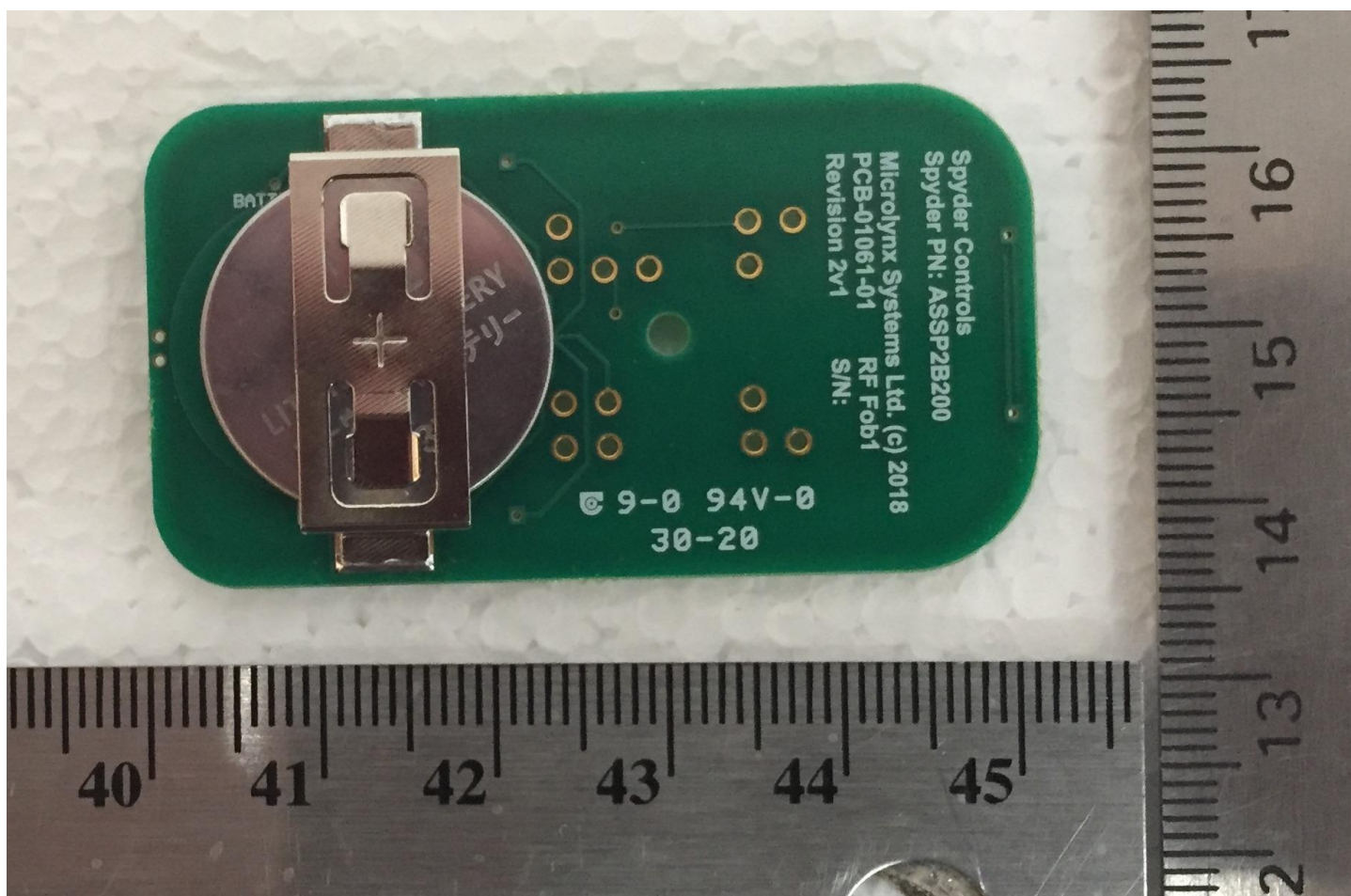
PCBA bottom view (With Battery)
