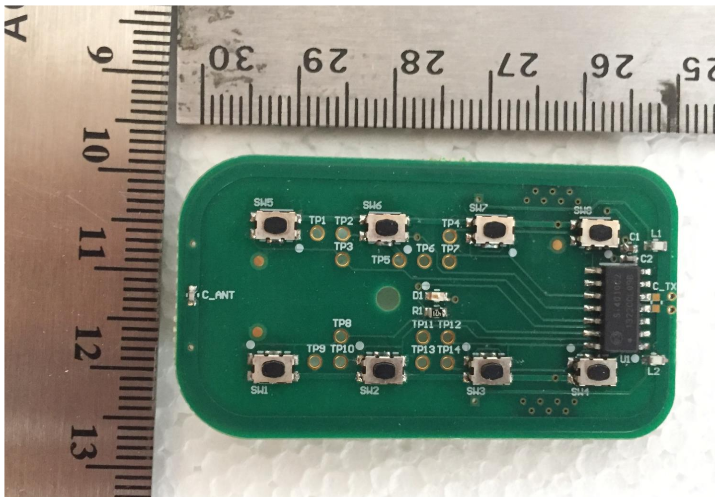
Radio PCBA top view
