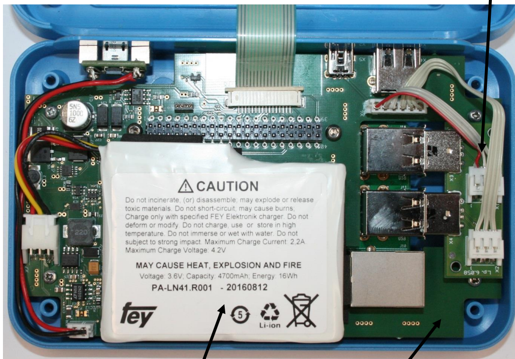
LOG PS-3 main pcb
