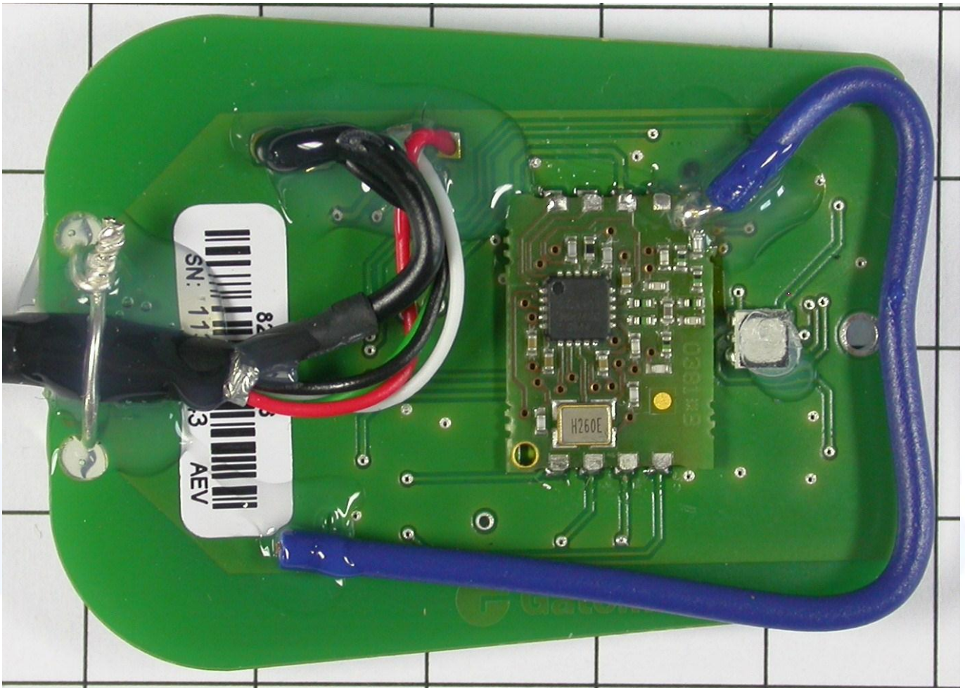
PCB top view
