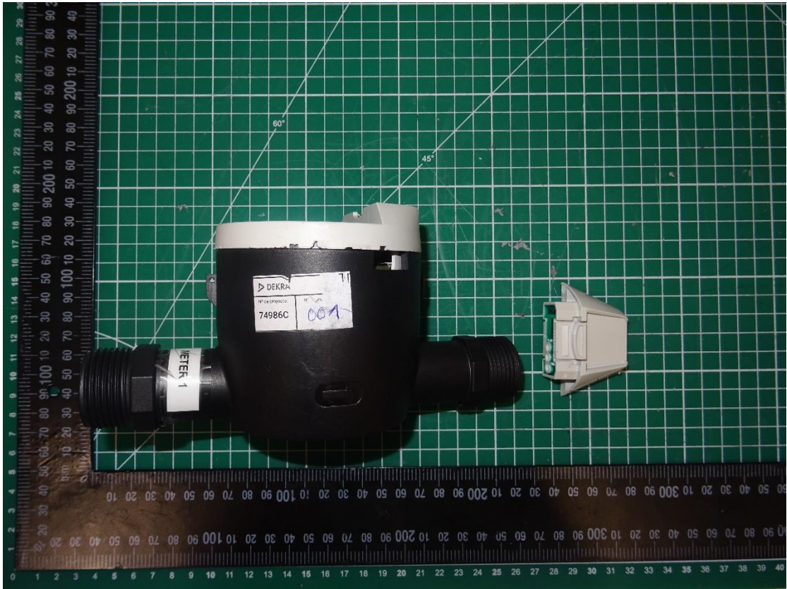
RADIATED EQUIPMENT VIEW OF CLICK ON ANTENNA
