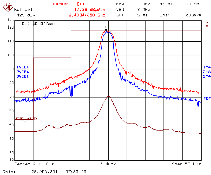
Plot 5.6.4.3. Band-Edge RF Radiated Emissions @ 3 m Low End of Frequency Band Rx Antenna Orientation: Vertical
