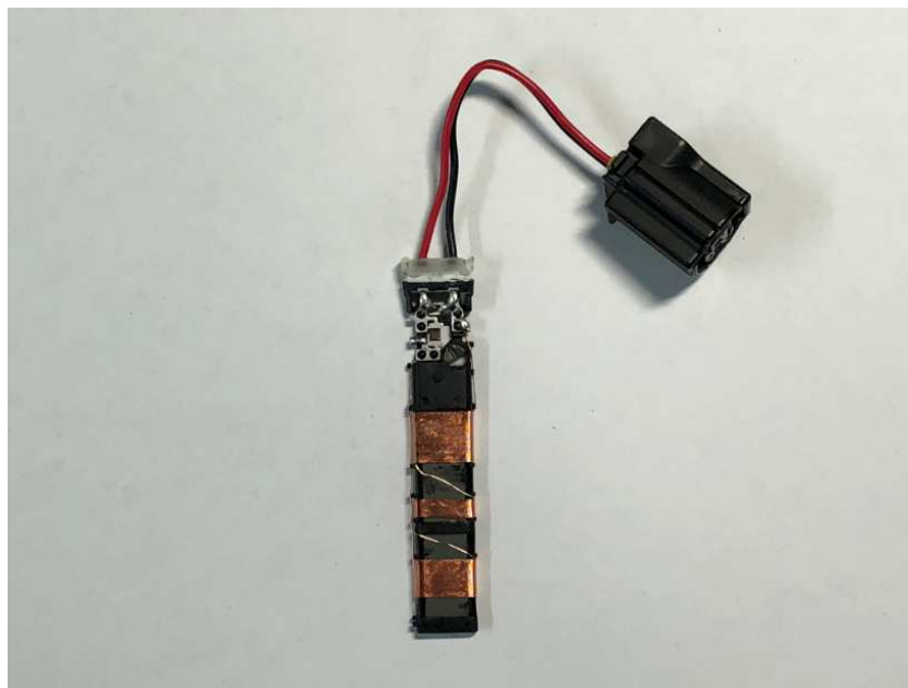
Figure 8.25 LF-antenna TG (CGF-M004-T05) internal (front view)
