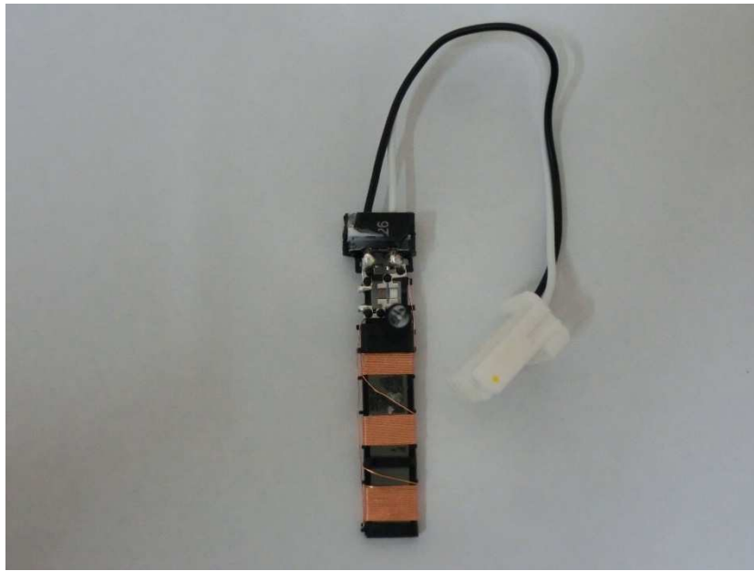
Figure 8.15 LF-antenna InF,InR (G8D-841M-ANT) internal (front view)
