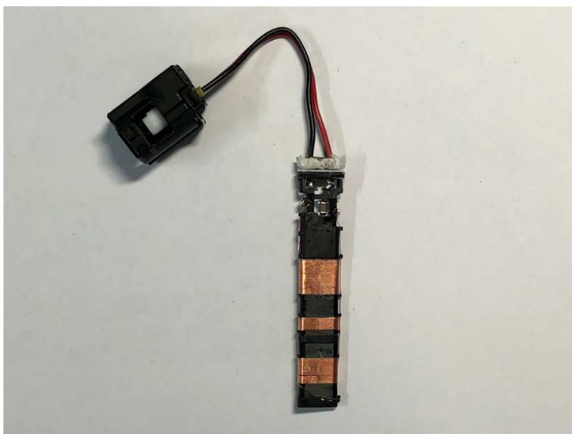
Figure 8.26 LF-antenna TG (CGF-M004-T05) internal (back view)
