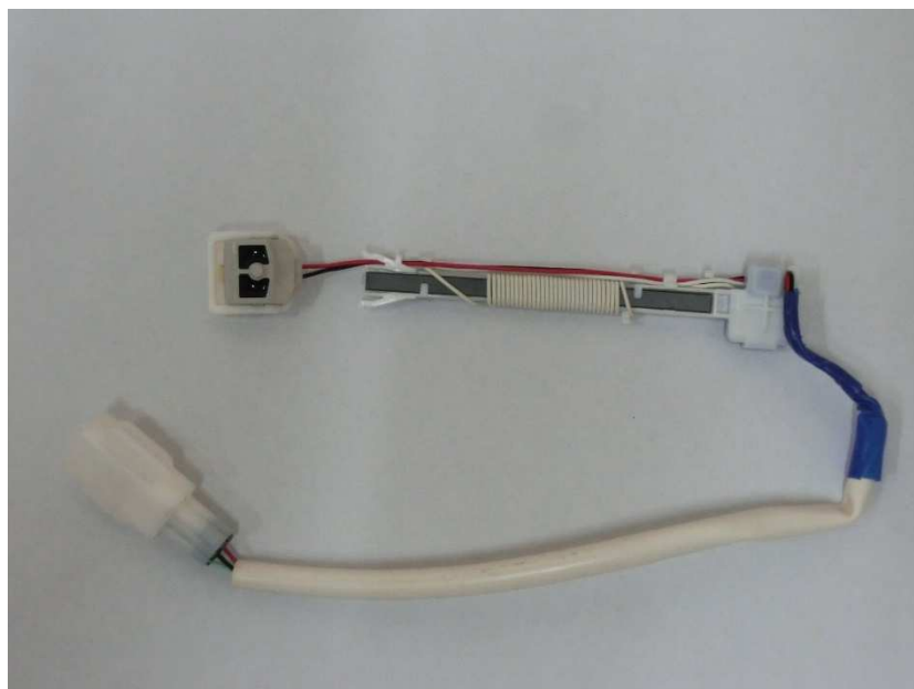
Figure 8.20 LF-antenna Dr(5716A639WB) internal (back view)
