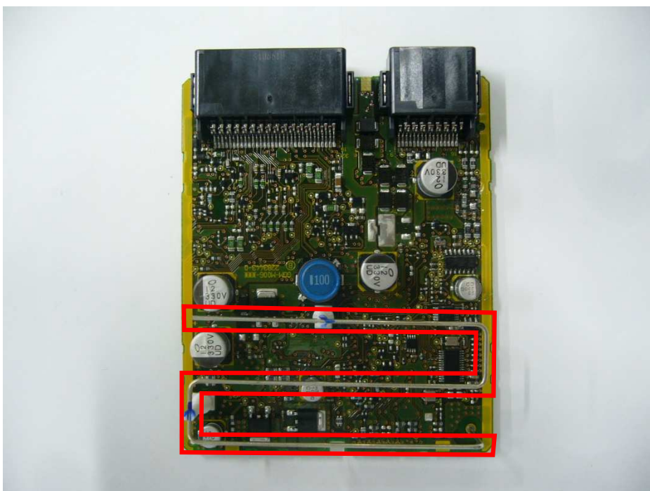
Figure 8.7.2 R706N integral antenna ( for UHF receiving ) location
