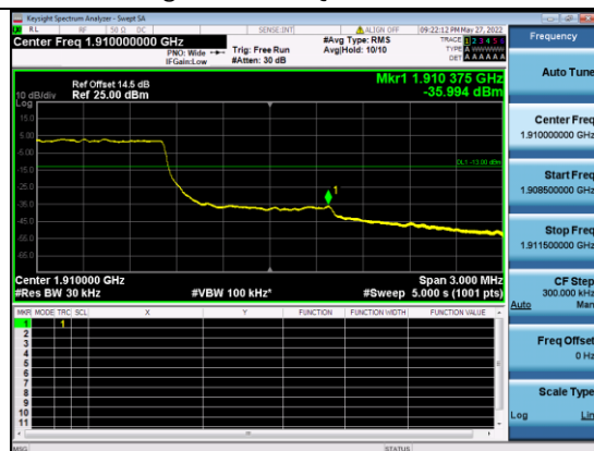
B2-10M-High CH-BE-QPSK-Full RB 0
