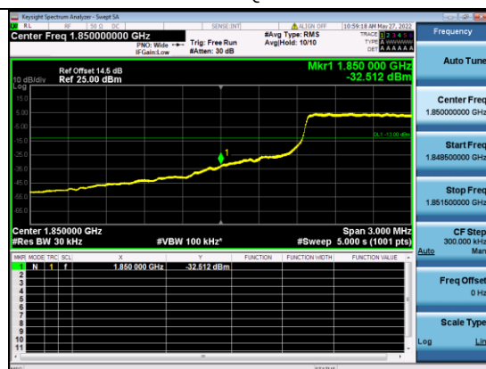
B2-10M-Low CH-BE-QPSK-Full RB 0
