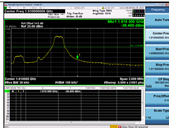
B2-3M-High CH-BE-QPSK-1 RB MAX
