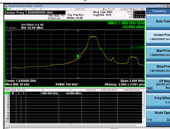
B2-5M-Low CH-BE-QPSK-1 RB 0
