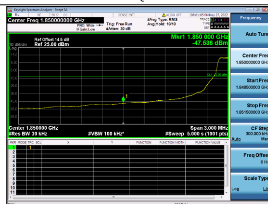
B2-20M-Low CH-BE-QPSK-1 RB 0
