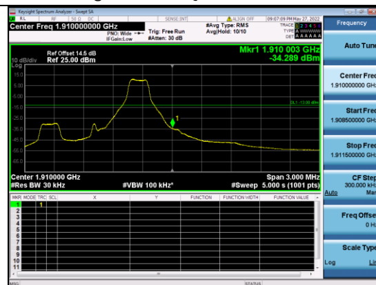
B2-5M-High CH-BE-QPSK-1 RB MAX
