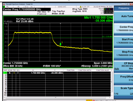
B4-5M-High CH-BE-QPSK-Full RB 0
