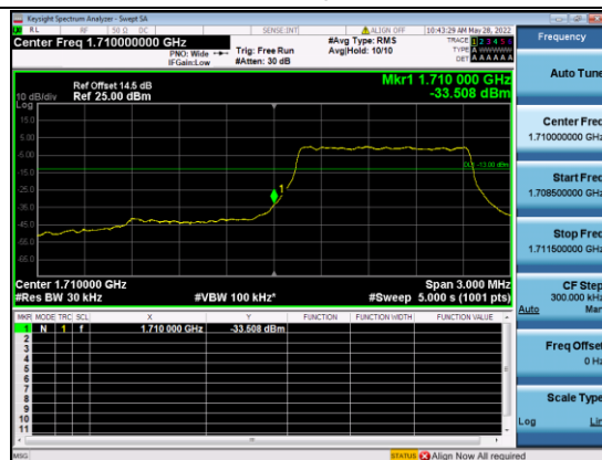
B4-1.4M-Low CH-BE-QPSK-Full RB 0
