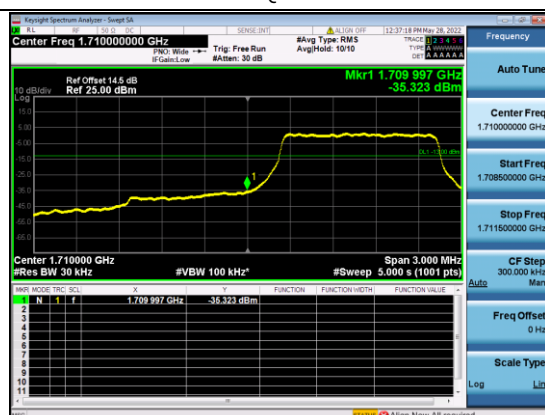
B4-5M-Low CH-BE-QPSK-Full RB 0
