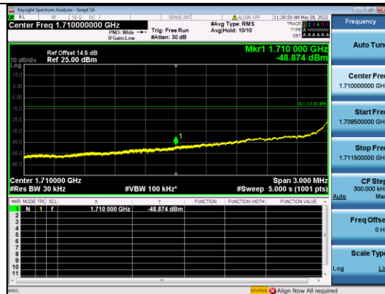
B4-3M-Low CH-BE-QPSK-Full RB 0
