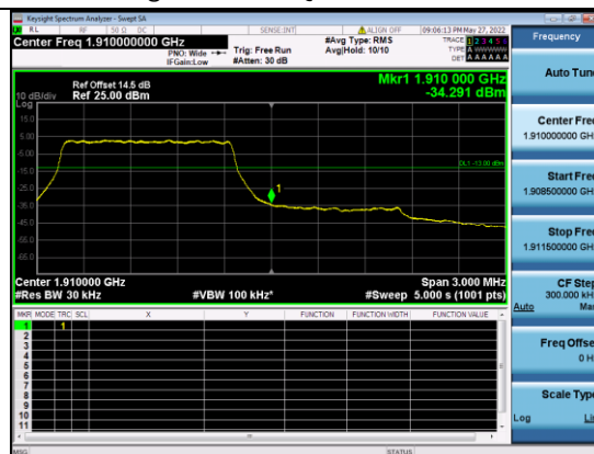
B2-5M-High CH-BE-QPSK-Full RB 0
