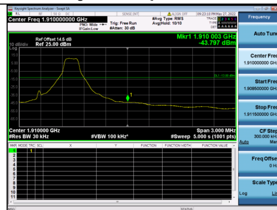
B2-10M-High CH-BE-QPSK-1 RB MAX
