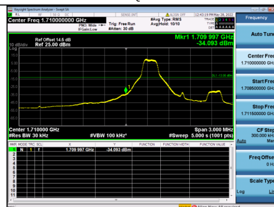
B4-5M-Low CH-BE-QPSK-1 RB 0
