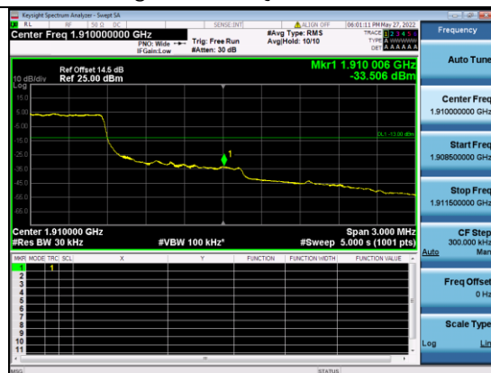
B2-15M-High CH-BE-QPSK-Full RB 0
