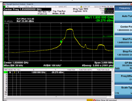
B2-1.4M-Low CH-BE-QPSK-1 RB 0
