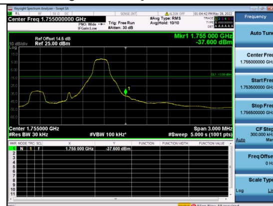
B4-5M-High CH-BE-QPSK-1 RB MAX
