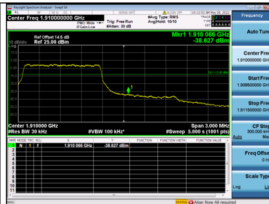
B2-3M-High CH-BE-QPSK-Full RB 0
