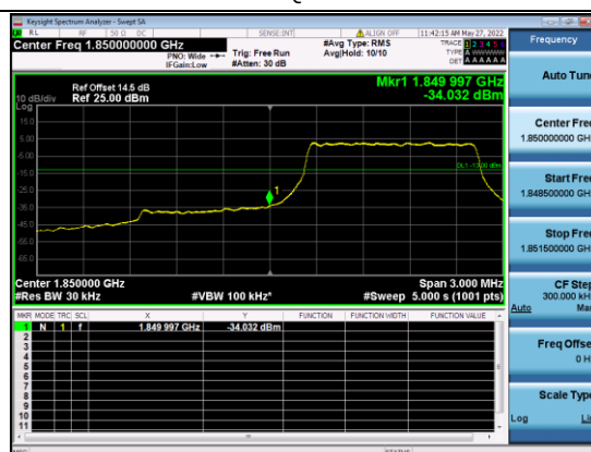
B2-5M-Low CH-BE-QPSK-Full RB 0
