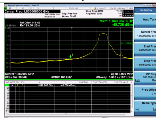
B2-10M-Low CH-BE-QPSK-1 RB 0
