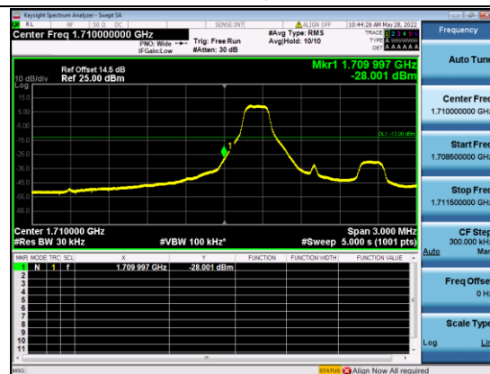
B4-1.4M-Low CH-BE-QPSK-1 RB 0
