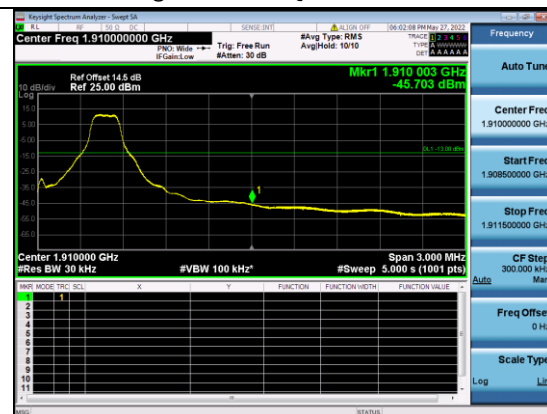
B2-15M-High CH-BE-QPSK-1 RB MAX
