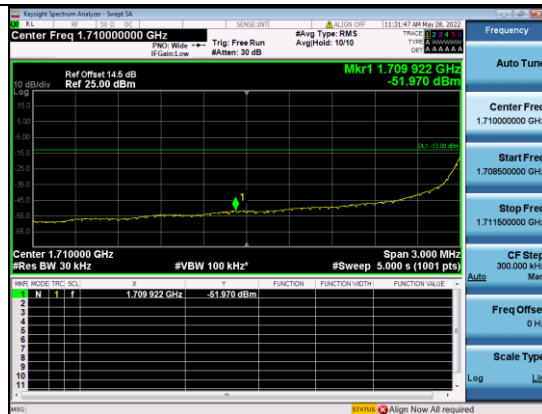
B4-3M-Low CH-BE-QPSK-1 RB 0
