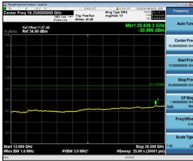
Band4-1.4MHz-16QAM-20175-1-0-Low-12000-26500--30.87-PASS
