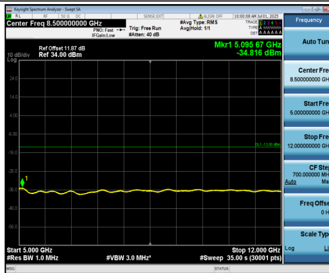
Band4-1.4MHz-QPSK-19957-1-0-Low-5000-12000--34.82-PASS
