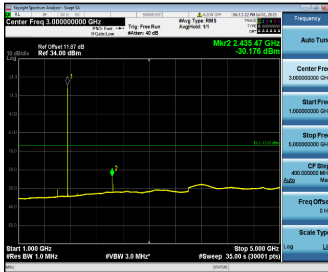
Band4-3MHz-QPSK-20385-1-0-High-1000-5000--30.18-PASS
