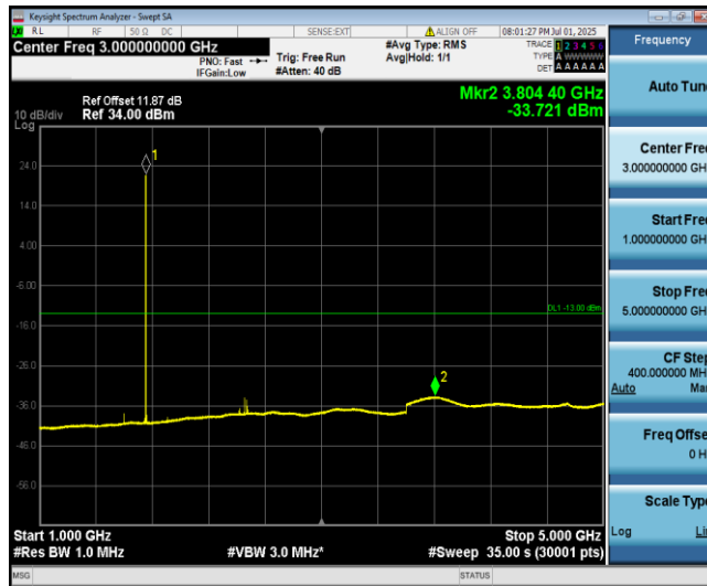
Band4-5MHz-QPSK-20375-1-0-High-1000-5000--33.72-PASS
