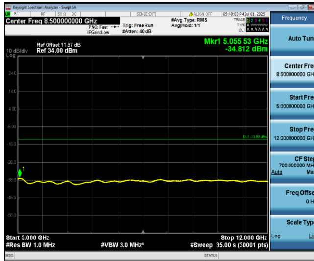
Band4-3MHz-QPSK-20175-1-0-Low-5000-12000--34.81-PASS
