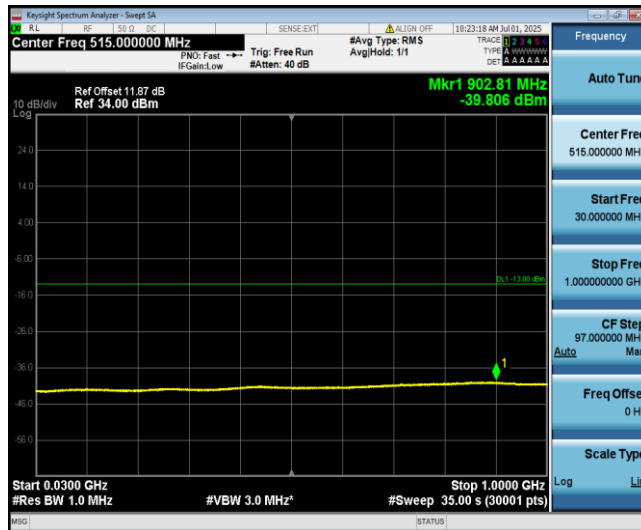
Band4-1.4MHz-16QAM-20175-1-0-Low-30-1000--39.81-PASS
