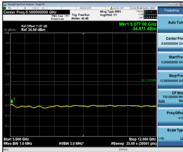
Band4-1.4MHz-QPSK-20393-1-0-High-5000-12000--34.87-PASS
