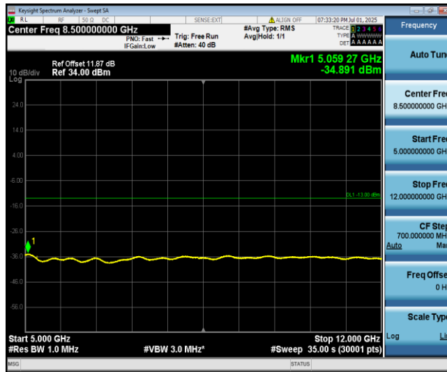
Band4-5MHz-16QAM-20175-1-0-Low-5000-12000--34.89-PASS
