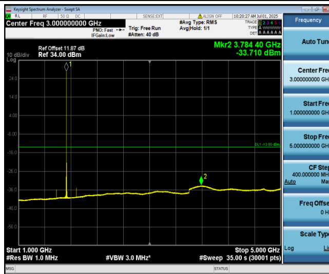
Band4-1.4MHz-QPSK-20175-1-0-Low-1000-5000--33.71-PASS
