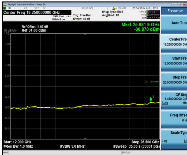
Band4-5MHz-QPSK-20175-1-0-Low-12000-26500--30.87-PASS
