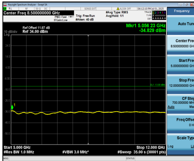
Band4-3MHz-QPSK-20385-1-0-High-5000-12000--34.83-PASS
