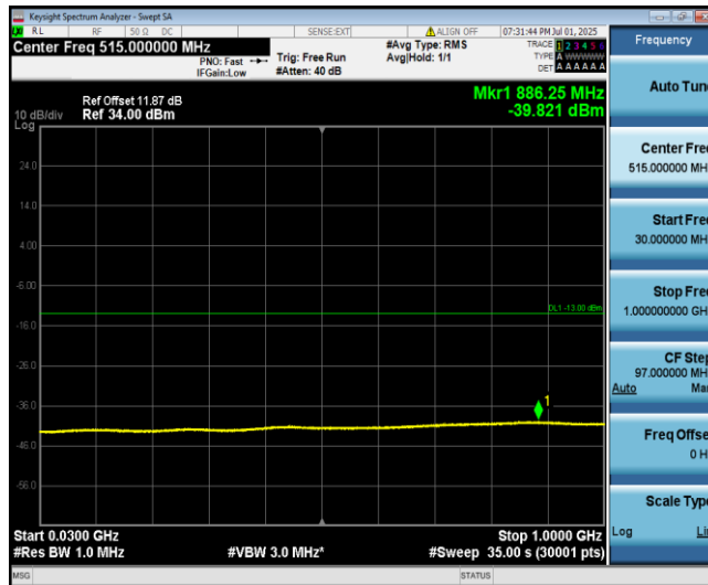
Band4-5MHz-16QAM-20175-1-0-Low-30-1000--39.82-PASS
