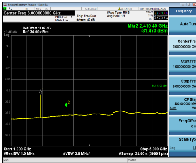
Band4-1.4MHz-QPSK-20393-1-0-High-1000-5000--31.47-PASS
