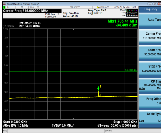
Band4-5MHz-QPSK-20175-1-0-Low-30-1000--34.49-PASS
