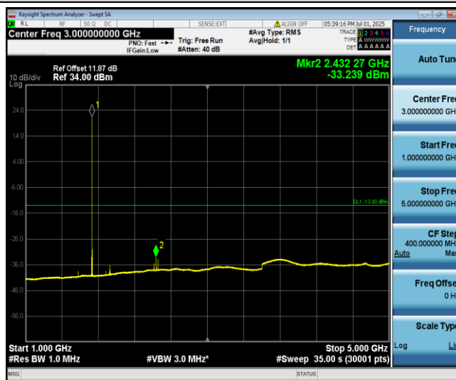
Band4-3MHz-QPSK-20175-1-0-Low-1000-5000--33.24-PASS
