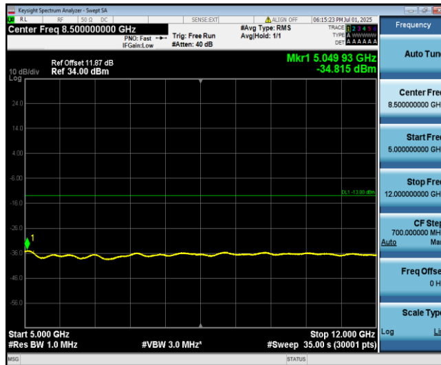
Band4-3MHz-16QAM-20385-1-0-High-5000-12000--34.82-PASS
