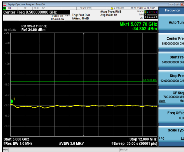
Band4-5MHz-QPSK-20375-1-0-High-5000-12000--34.85-PASS
