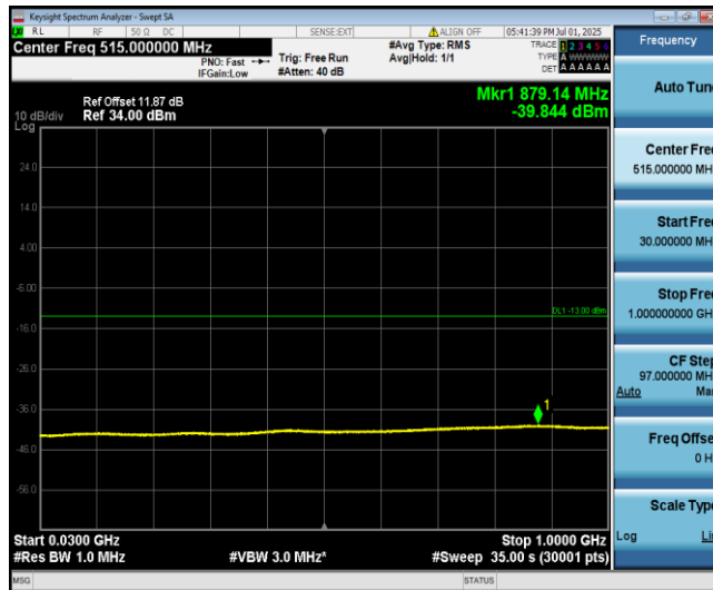
Band4-3MHz-16QAM-20175-1-0-Low-30-1000--39.84-PASS
