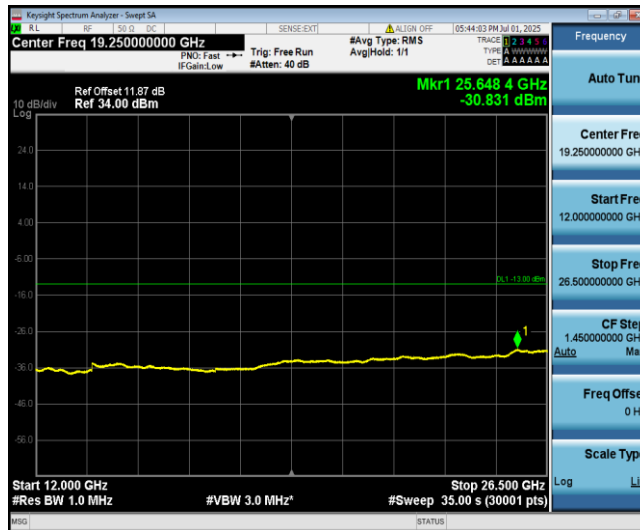
Band4-3MHz-16QAM-20175-1-0-Low-12000-26500--30.83-PASS
