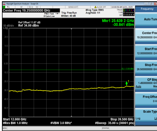
Band4-1.4MHz-QPSK-19957-1-0-Low-12000-26500--30.84-PASS
