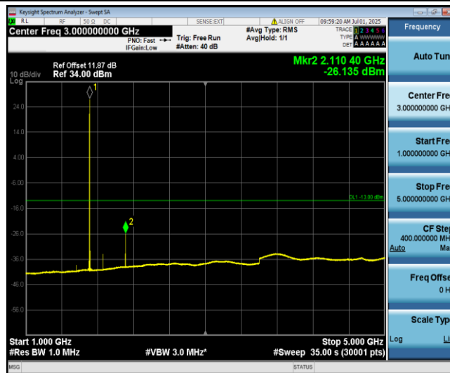
Band4-1.4MHz-QPSK-19957-1-0-Low-1000-5000--26.14-PASS
