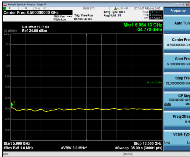
Band4-5MHz-QPSK-20175-1-0-Low-5000-12000--34.77-PASS
