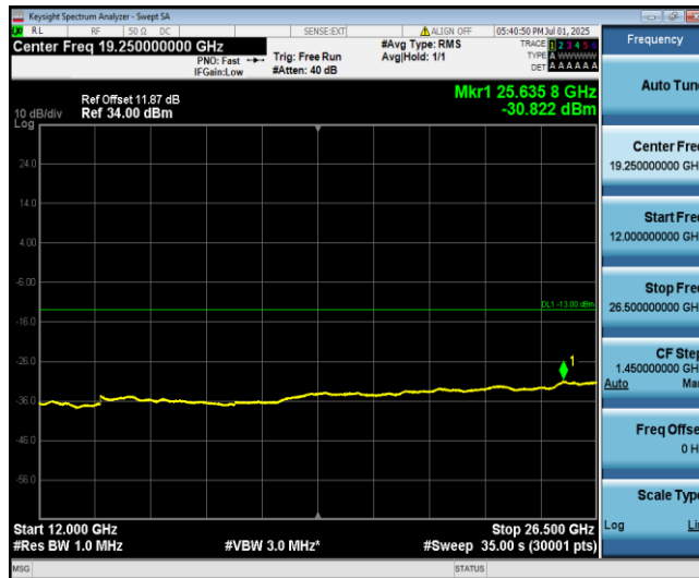
Band4-3MHz-QPSK-20175-1-0-Low-12000-26500--30.82-PASS
