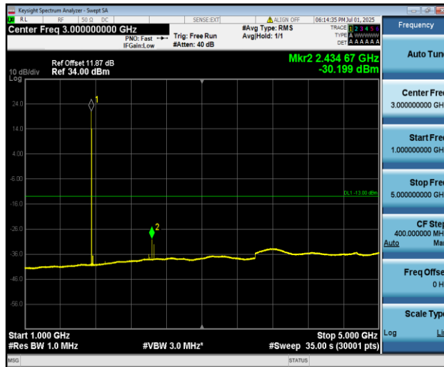
Band4-3MHz-16QAM-20385-1-0-High-1000-5000--30.2-PASS
