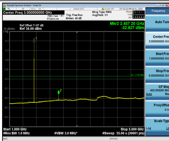
Band4-5MHz-16QAM-20175-1-0-Low-1000-5000--32.63-PASS
