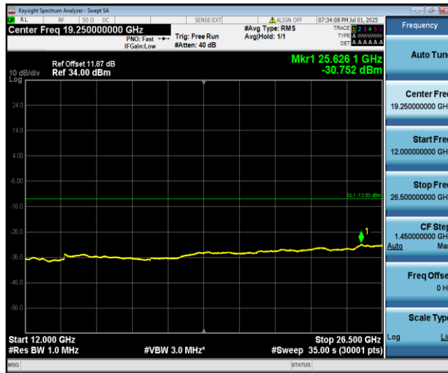
Band4-5MHz-16QAM-20175-1-0-Low-12000-26500--30.75-PASS
