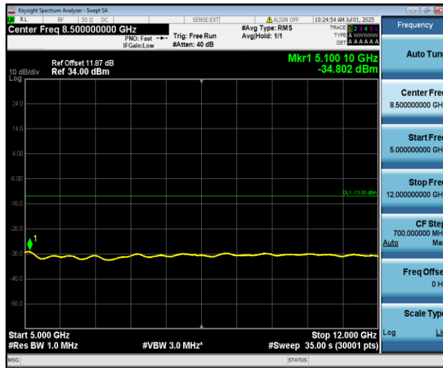
Band4-1.4MHz-16QAM-20175-1-0-Low-5000-12000--34.8-PASS
