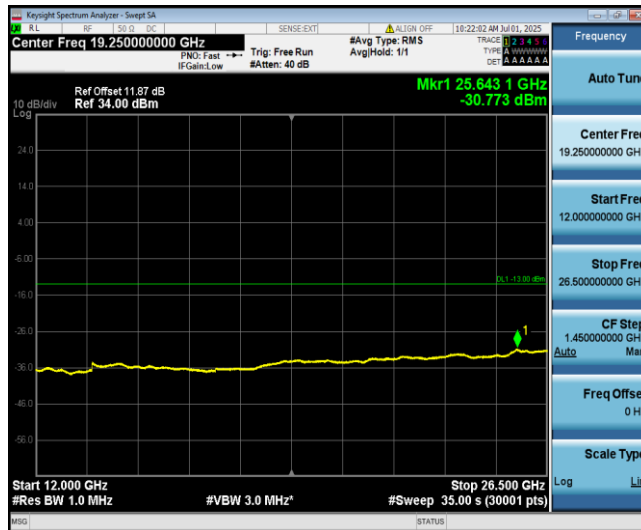
Band4-1.4MHz-QPSK-20175-1-0-Low-12000-26500--30.77-PASS
