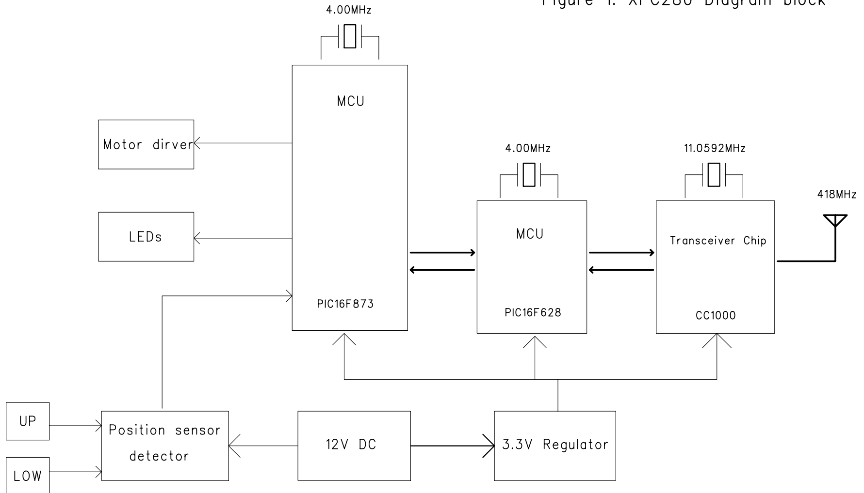
Figure 1. XPC280 Diagram block
