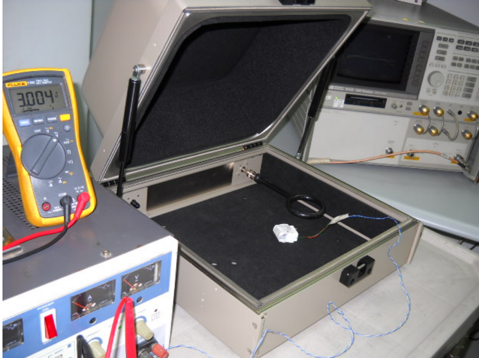
Photograph No.4 Setup for occupied bandwidth measurements
