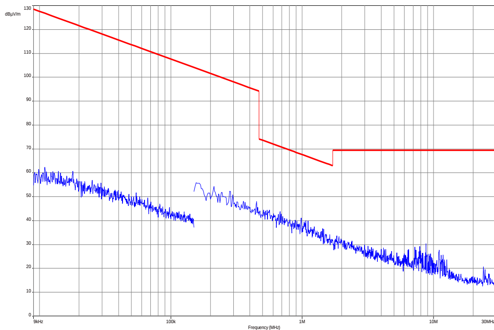
Plot 2: 9 kHz to 30 MHz, QPSK
