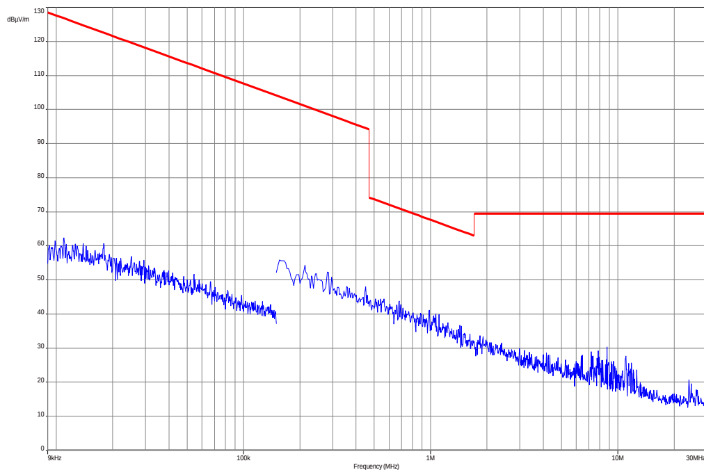
Plot 1: 9 kHz to 30 MHz, BPSK
