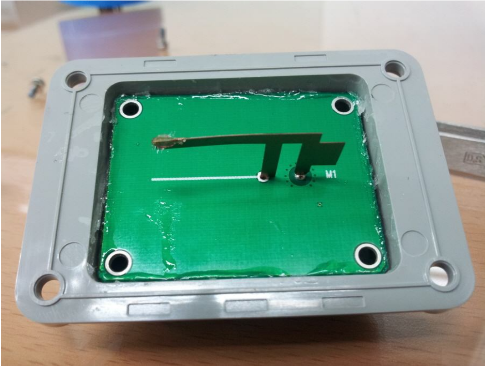
Antenna Board
