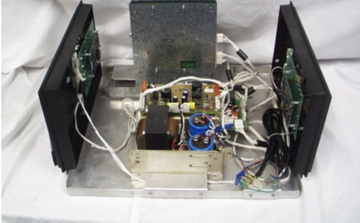
Wayne Dresser 13.56 MHz Reader (Shell Easy Pay), Side View
