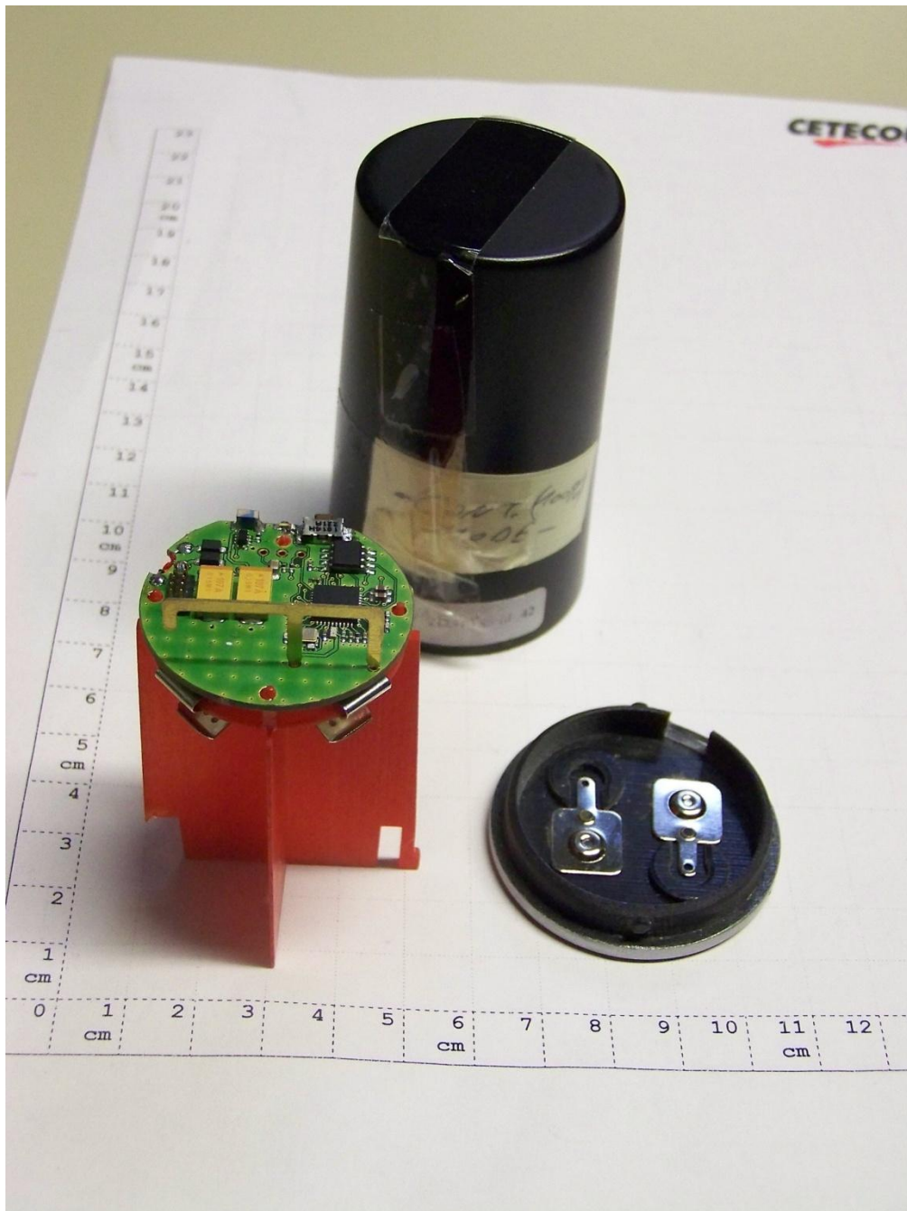
PCB with battery taper shank removed of EUT A
