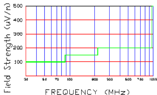
Figure 11. Spurious Radiated Limits at 3 meters
