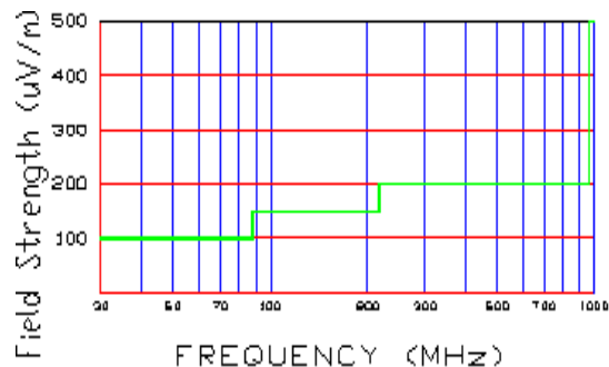
Figure 12. Spurious Radiated Limits at 3 meters
