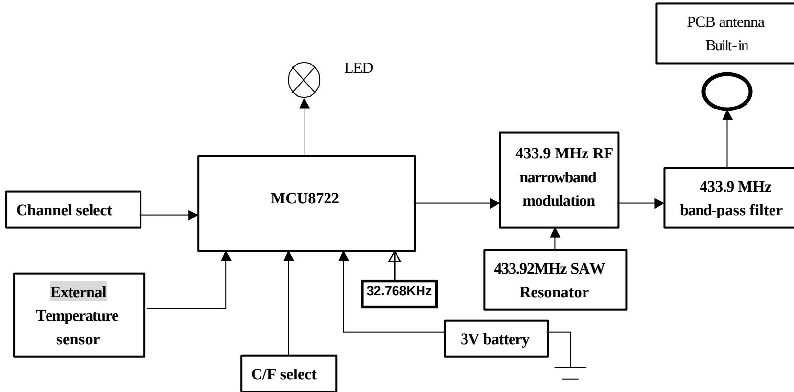
Figure 1 C8203FCC Block diagram
