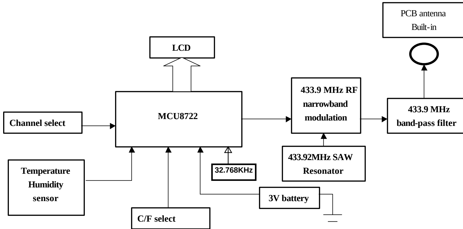
Figure 1 C8202FCC Block diagram
