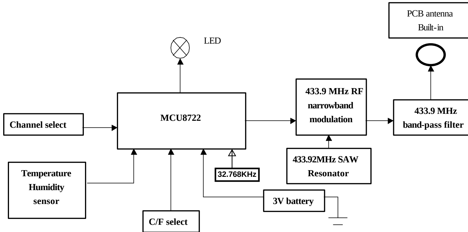
Figure 1 C8201FCC Block diagram
