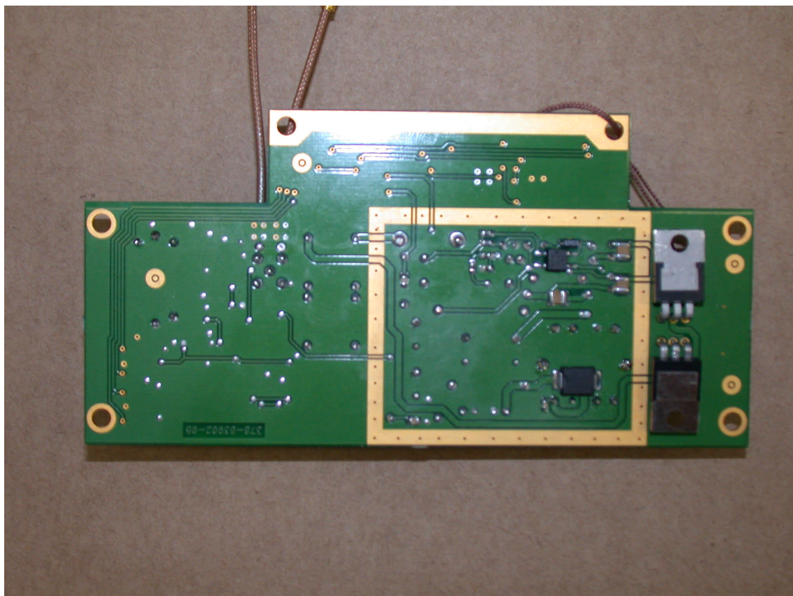
PSU/TCXO Bottom Assembly without Screening Can
