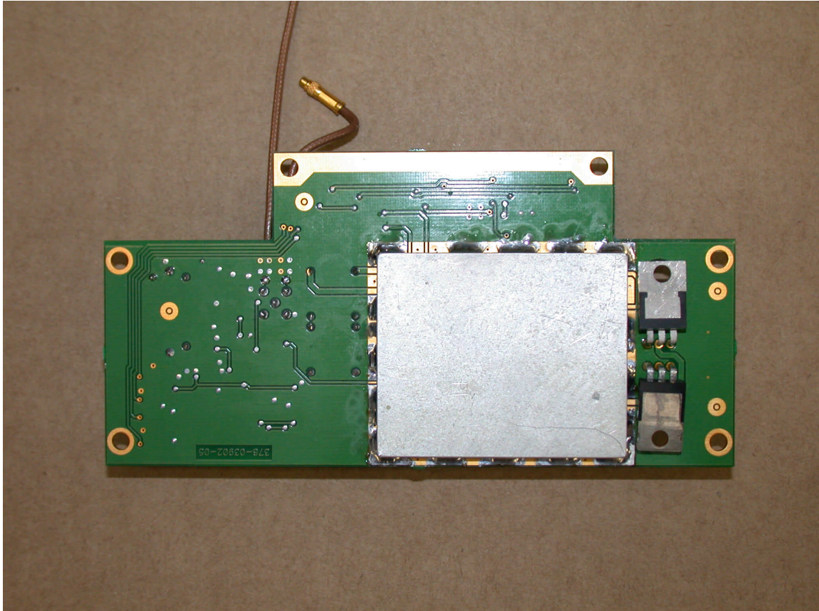
PSU/TCXO Bottom Assembly with Screening Can
