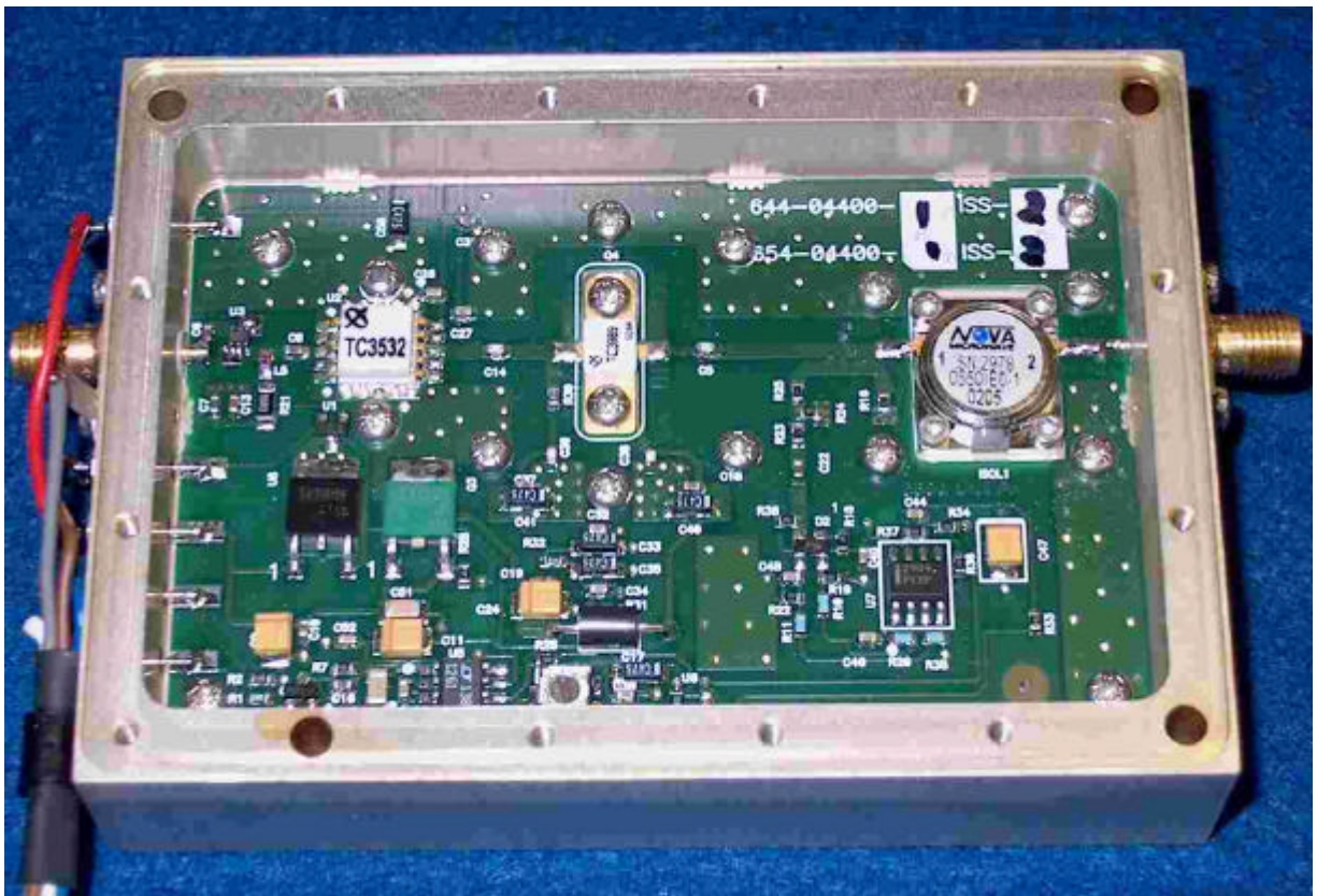
Power Amplifier with Lid Removed
