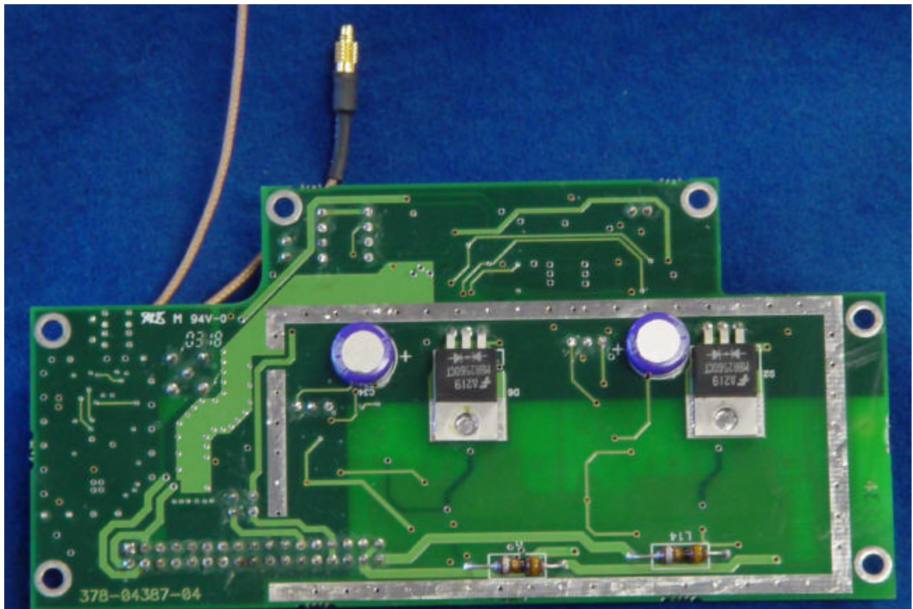
PSU/TCXO Bottom cans removed
