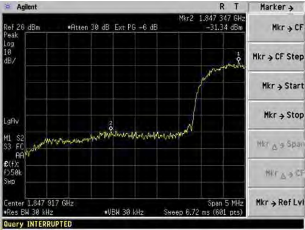
Low Band Edge UMTS BAND II CH 9262
