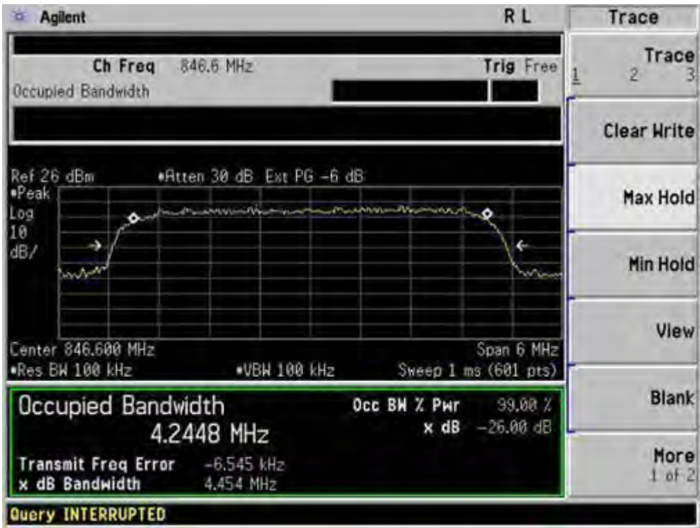
Occupied Bandwidth (99%) UMTS BAND V CH 4233
