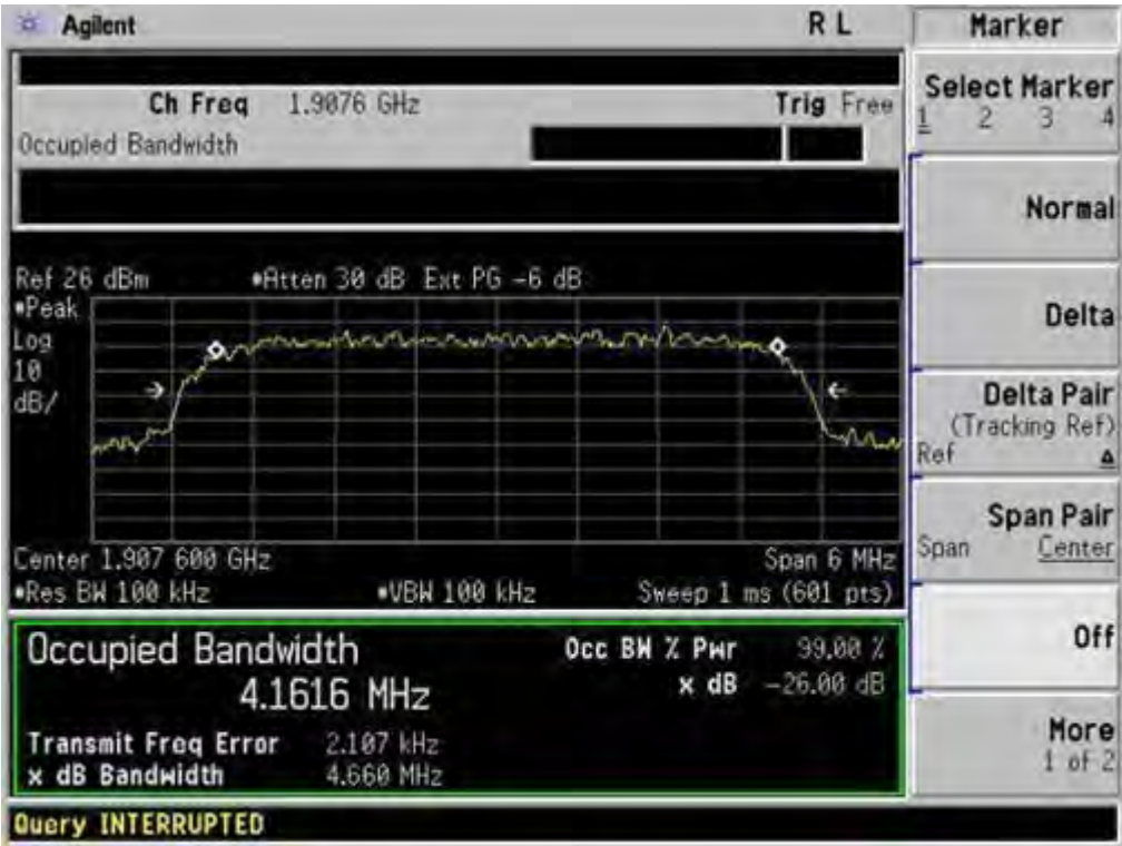
Occupied Bandwidth (99%) UMTS band II CH 9538
