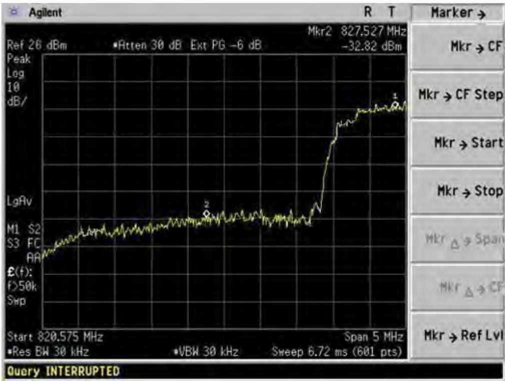
Low Band Edge UMTS BAND V CH 4132
