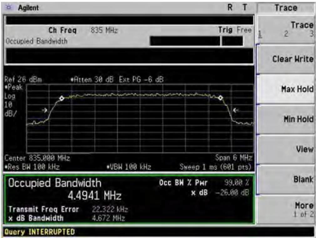
Occupied Bandwidth (99%) UMTS BAND V CH 4175
