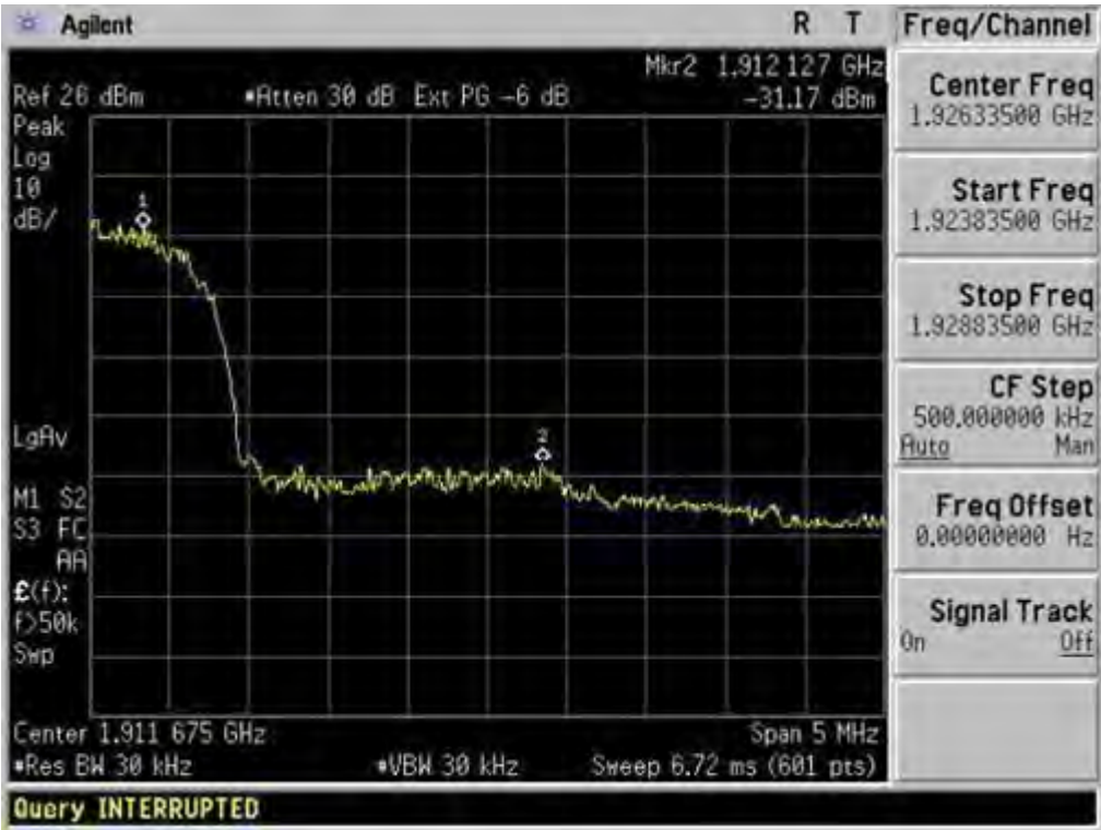
High Band Edge UMTS BAND II CH 9538
