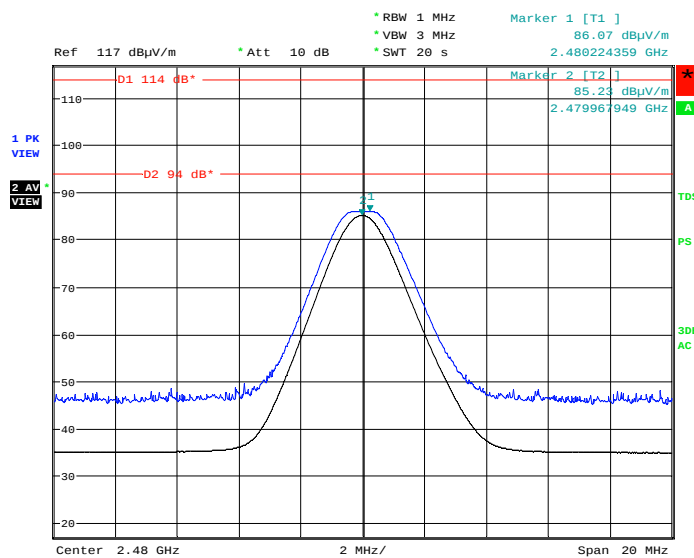
Figure 13: Field Strength of Fundamental, Spectral Diagram, Mode C (2480MHz)
