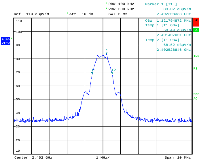
Figure 8: 99% Bandwidth, Mode A (2402MHz)
