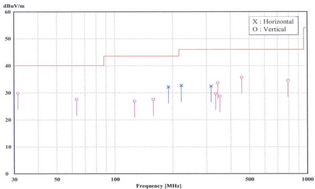
< Fig 6-1. Radiated emission result >
