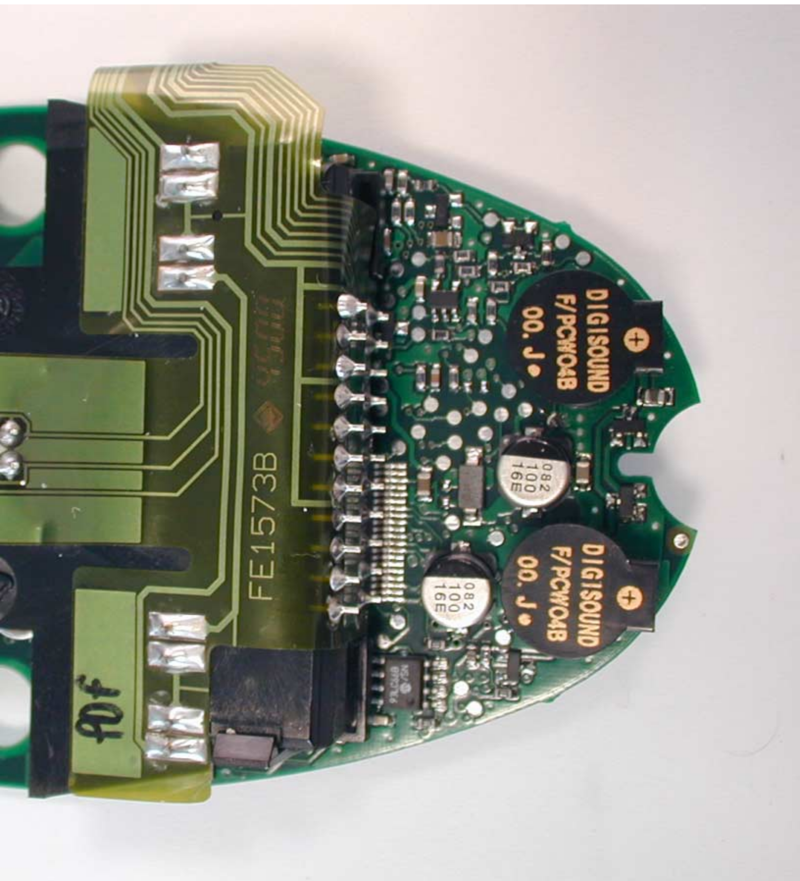
MOTHER BOARD AND CCD UPPER VIEW
