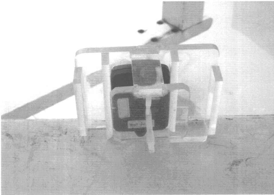
Figure 3.3 Radiated Test Setup ( Axis-Z )
