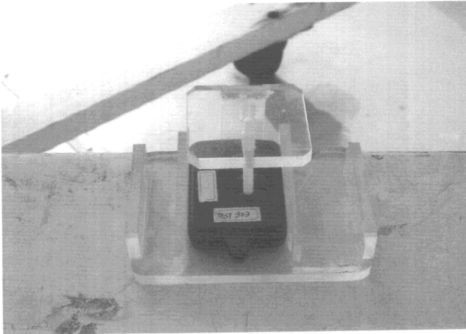
Figure 3.1 Radiated Test Setup ( Axis-X )
