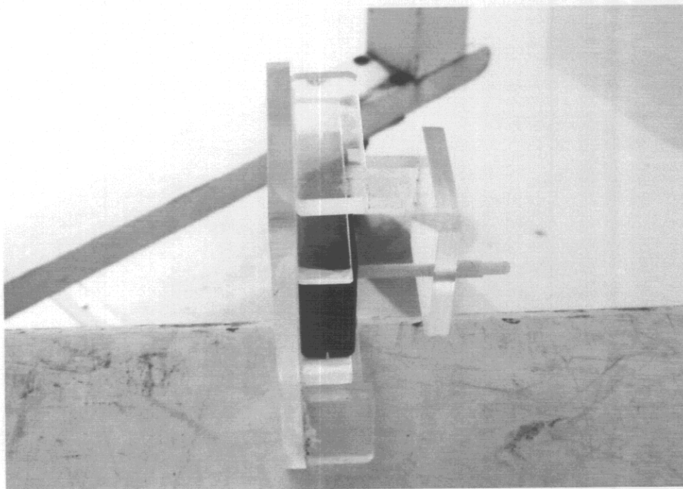
Figure 3.2 Radiated Test Setup ( Axis-Y )
