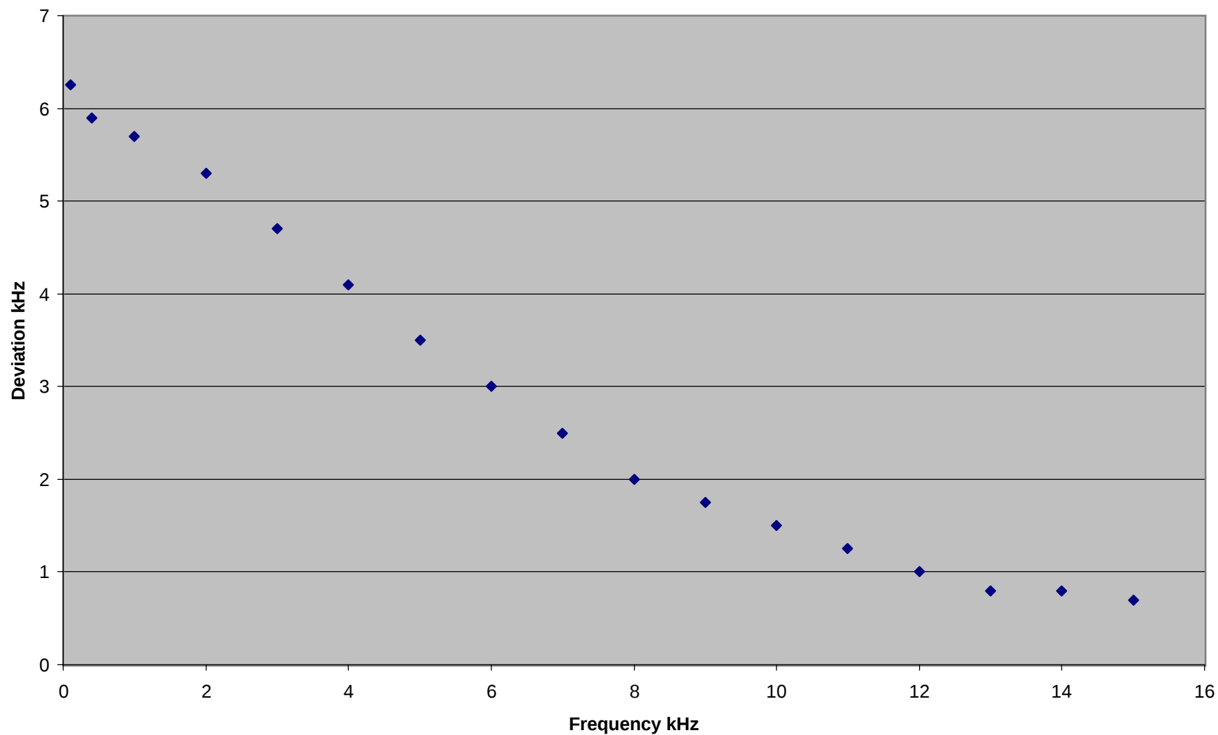
LT700 Frequency Response Ch. 1K
