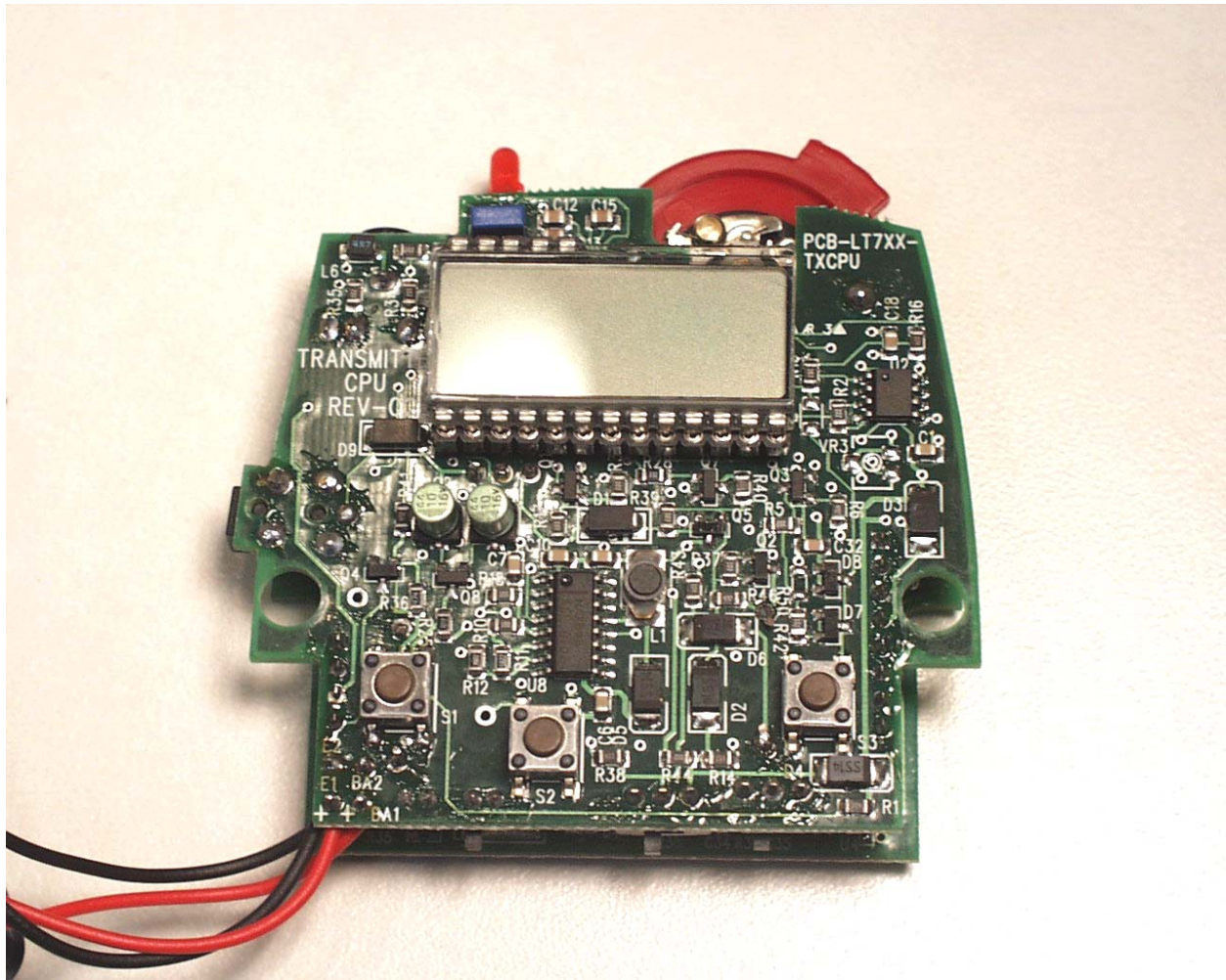
Photograph 10 - Front View of the Control PCB
