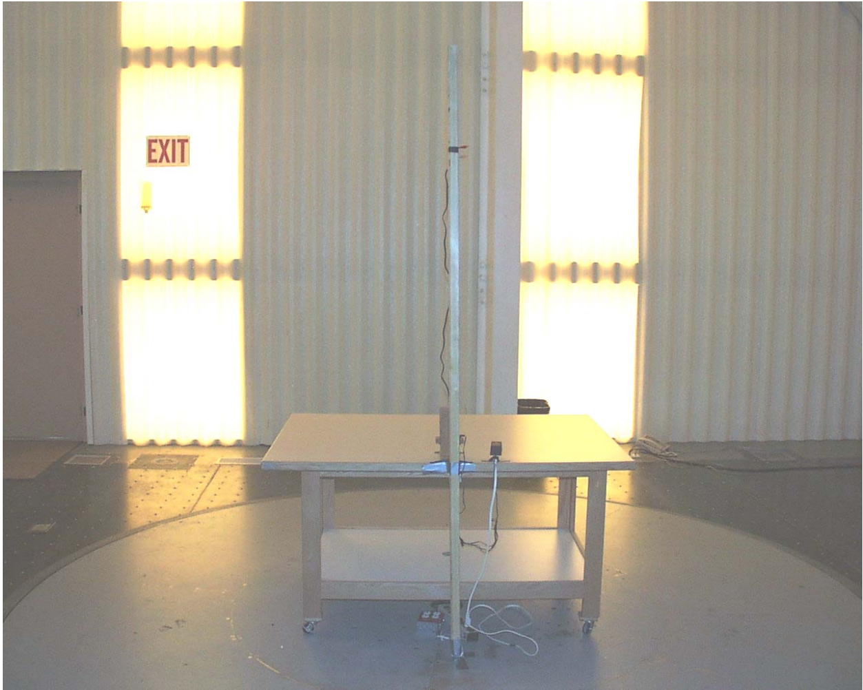
Photograph 2 - Rear View Radiated Emission Configuration (Vertical Orientation)
