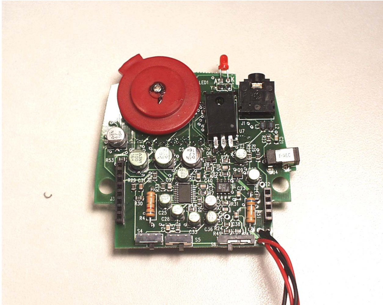
Photograph 11 - Rear Side of the Control PCB
