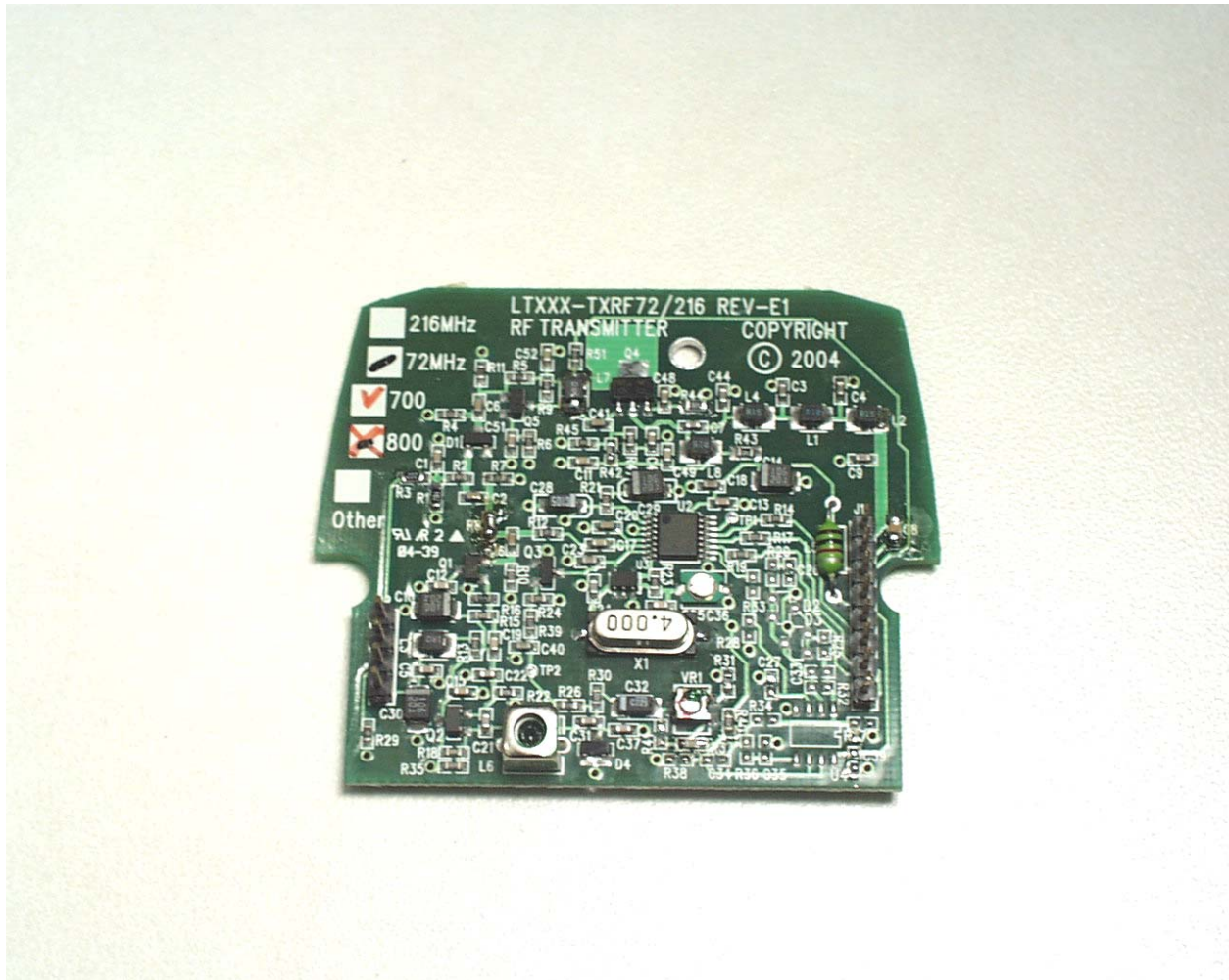
Photograph 12 - Component Side of the Transmitter PCB
