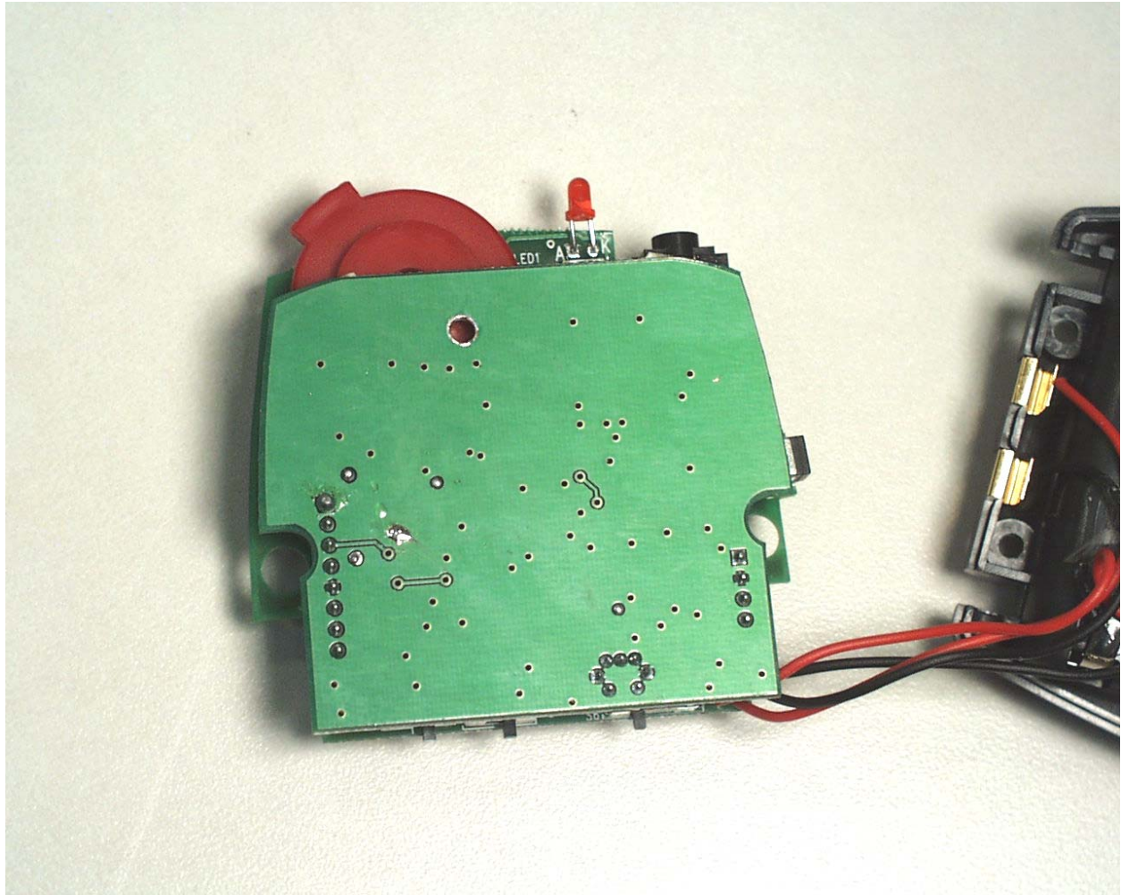
Photograph 13 - Trace Side of the Transmitter PCB While Connected to the Control Card
