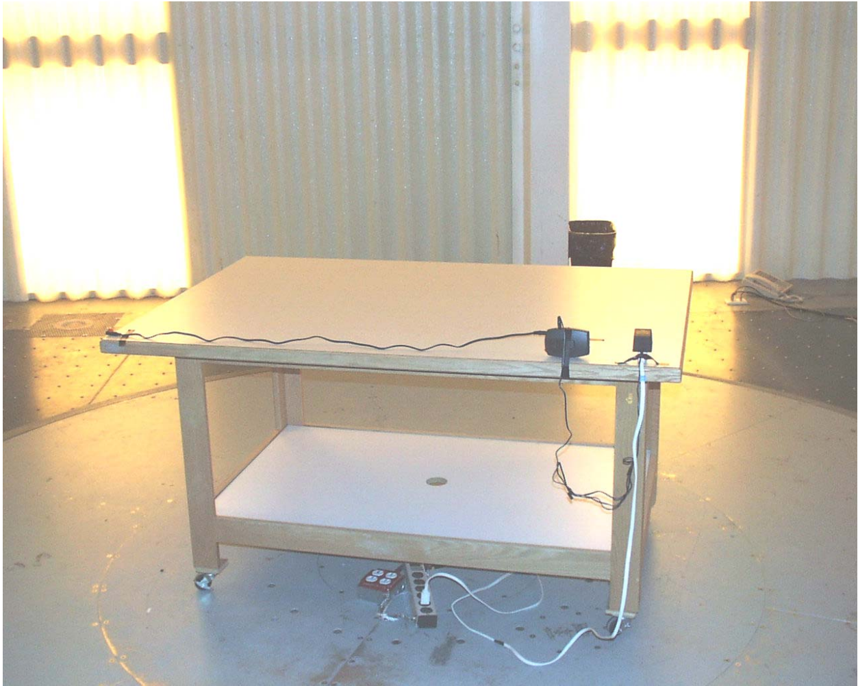
Photograph 4 - Rear View Radiated Emission Configuration (Horizontal Orientation)
