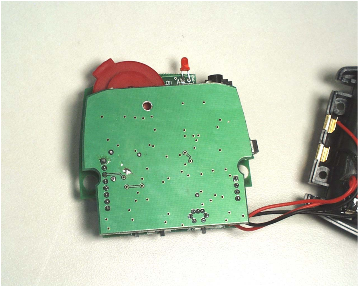
Trace Side of the Transmitter PCB While Connected to the Control Card
