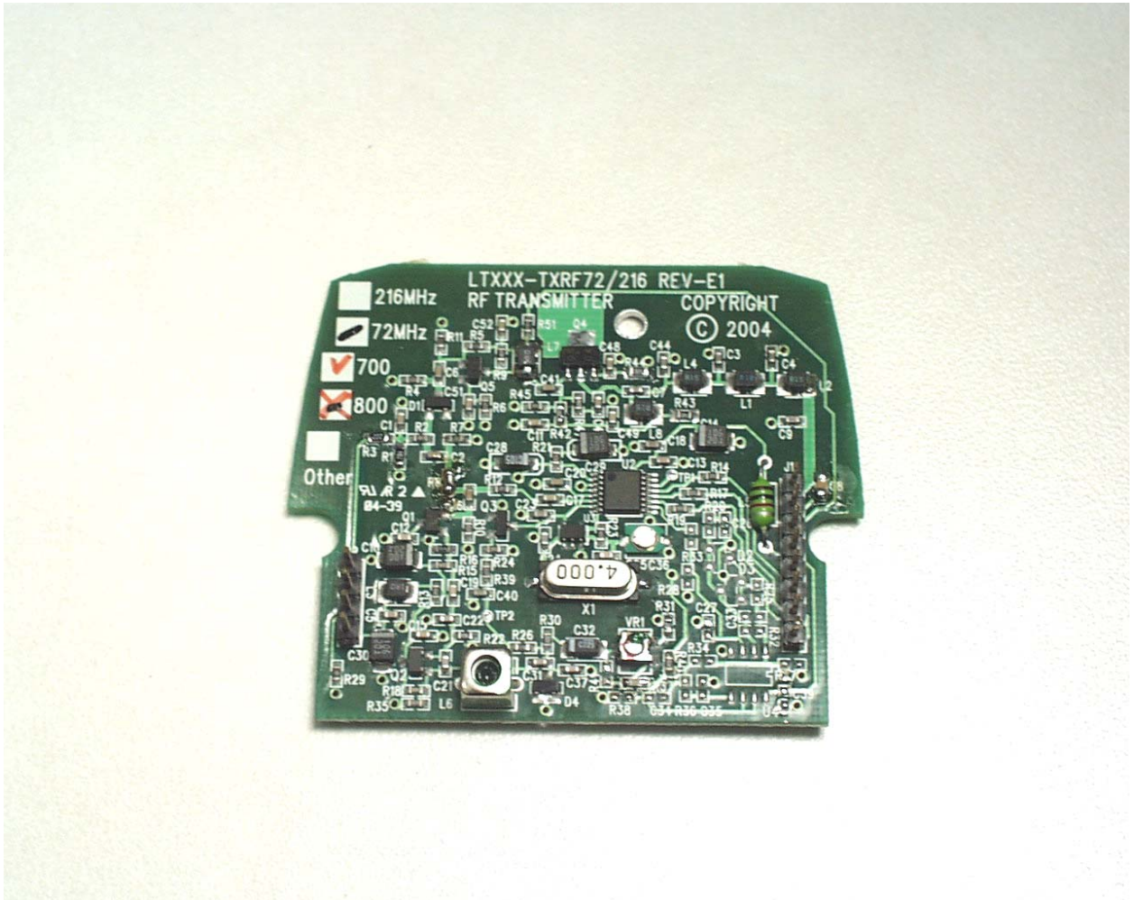
Component Side of the Transmitter PCB
