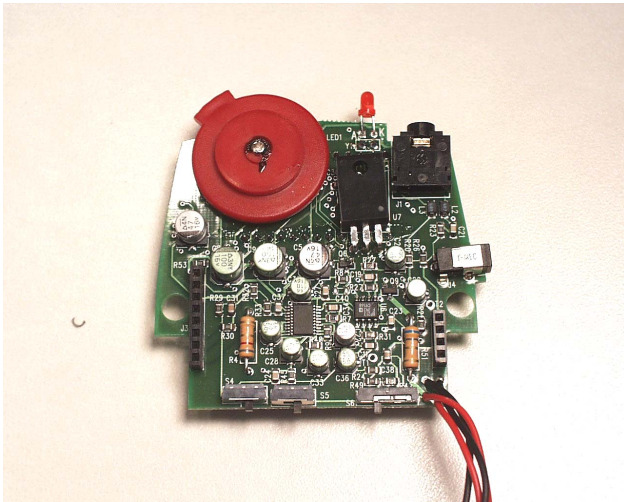
Rear Side of the Control PCB
