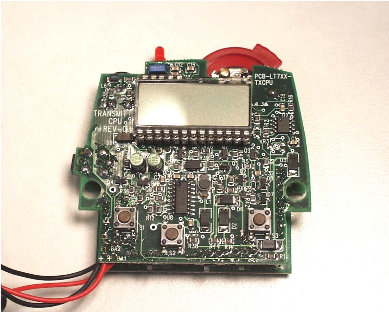
Front View of the Control PCB
