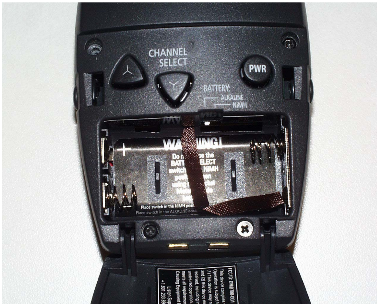
Front Cover Opened Showing Battery Compartment
