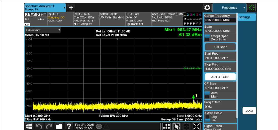
11B-Ant2-2437-30~1000-PASS
