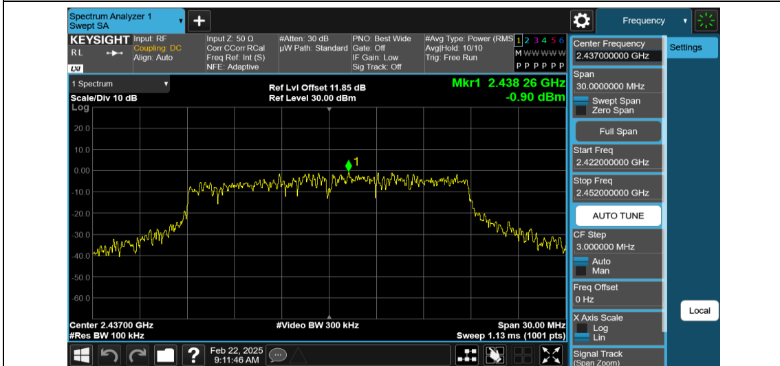
11N20MIMO-Ant2-2437-0~Reference-PASS
