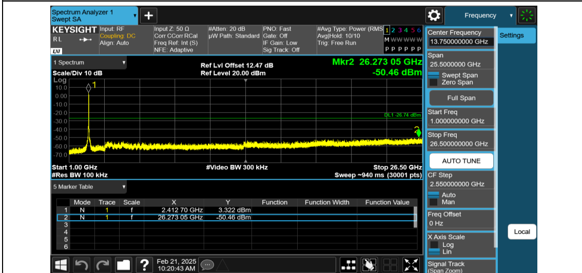
11N20MIMO-Ant1-2412-1000~26500-PASS
