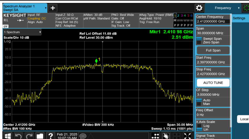
11G-Ant2-2412-0~Reference-PASS
