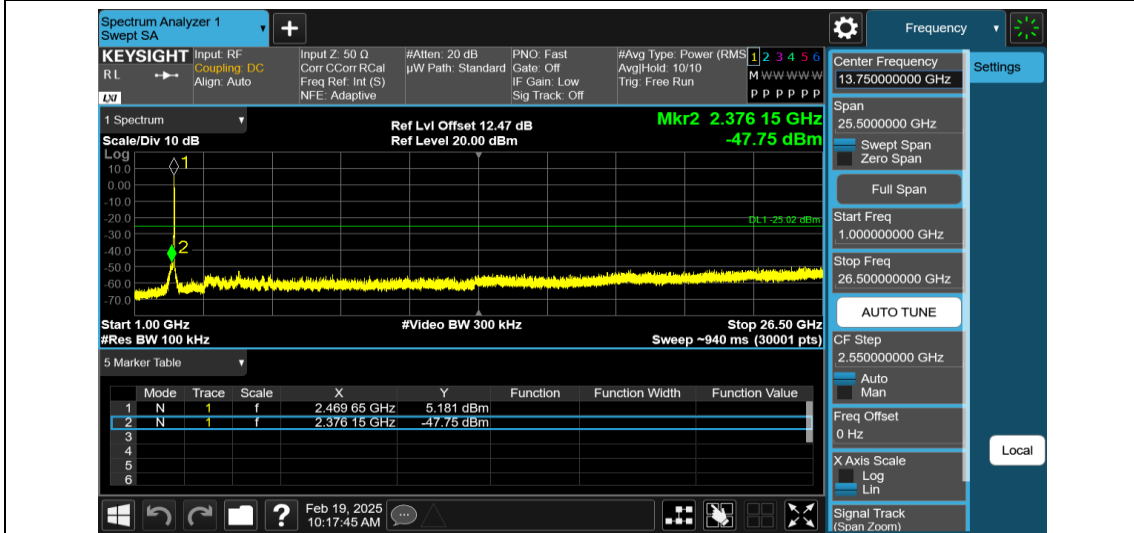
11G-Ant1-2462-1000~26500-PASS
