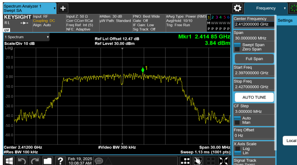
11G-Ant1-2412-0~Reference-PASS
