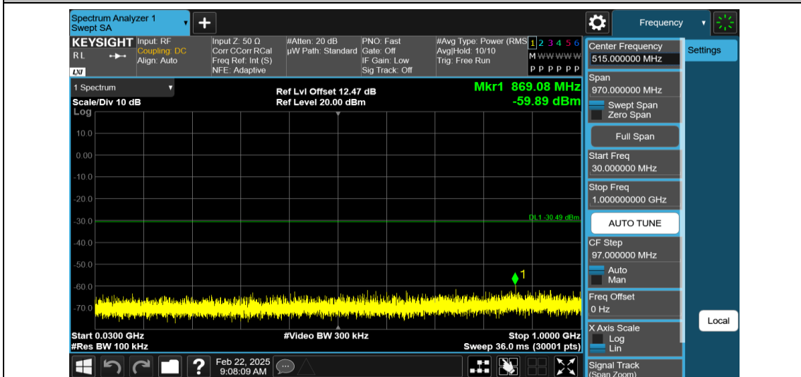
11N20MIMO-Ant1-2437-30~1000-PASS
