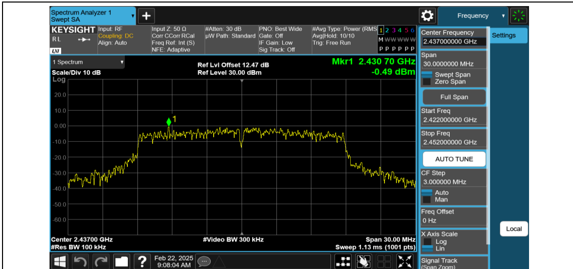
11N20MIMO-Ant1-2437-0~Reference-PASS
