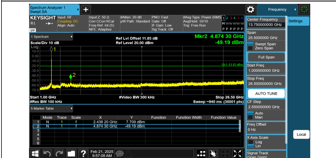
11B-Ant2-2437-1000~26500-PASS
