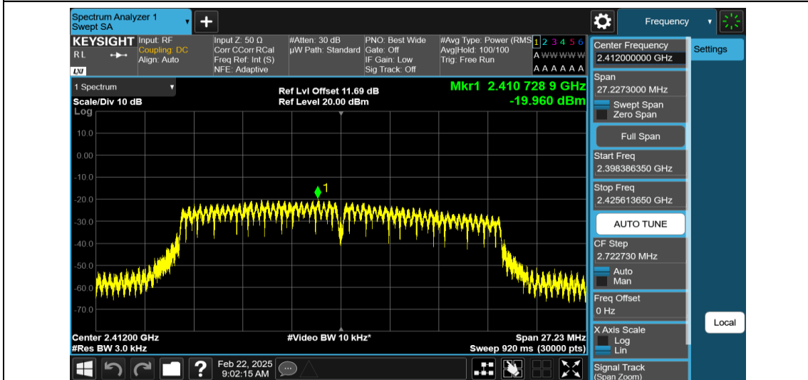
11N20MIMO-Ant2-2412-PASS
