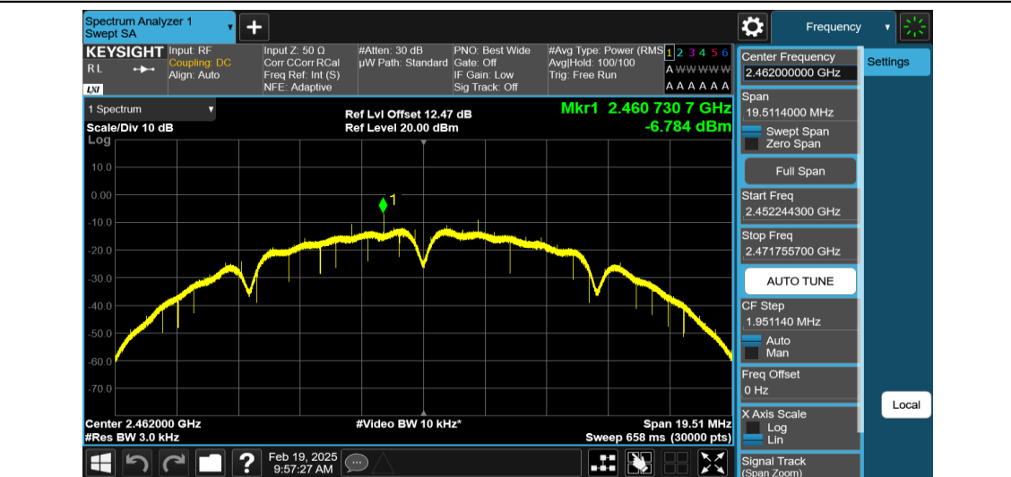
11B-Ant1-2462-PASS
