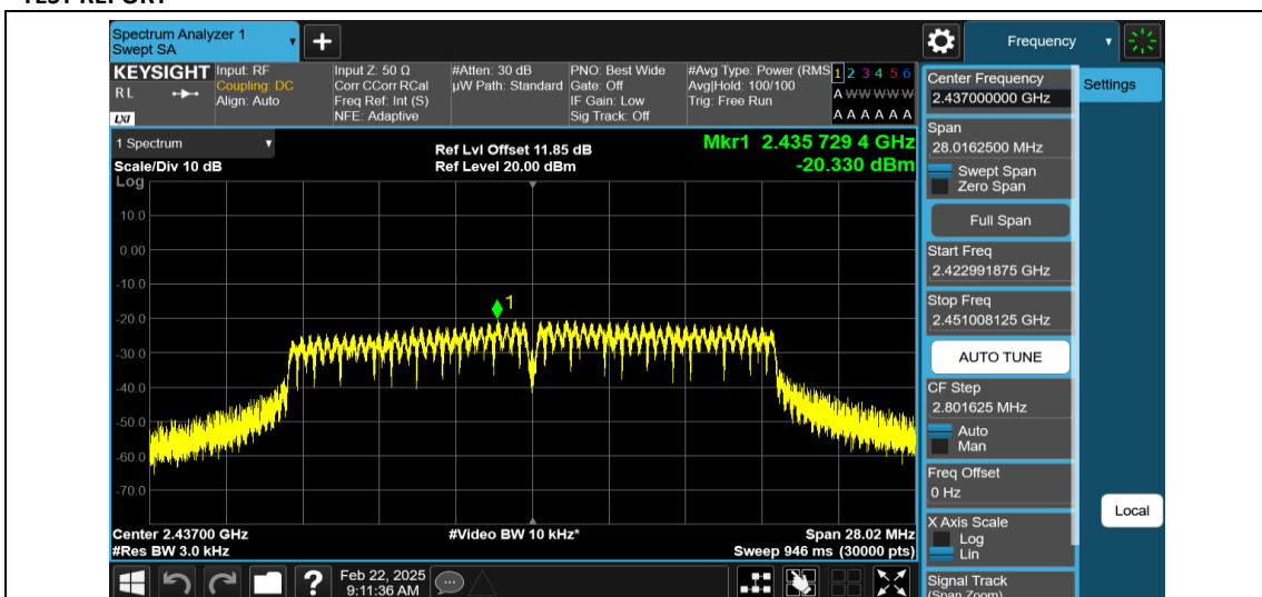
11N20MIMO-Ant2-2437-PASS
