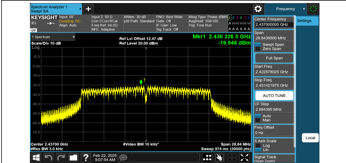
11N20MIMO-Ant1-2437-PASS
