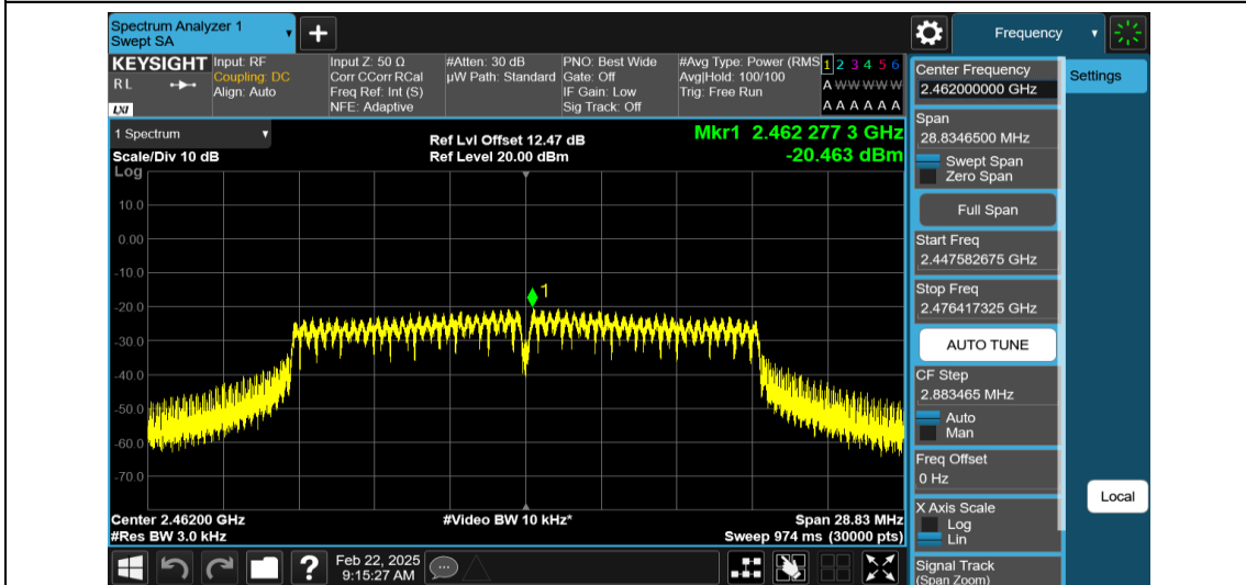
11N20MIMO-Ant1-2462-PASS
