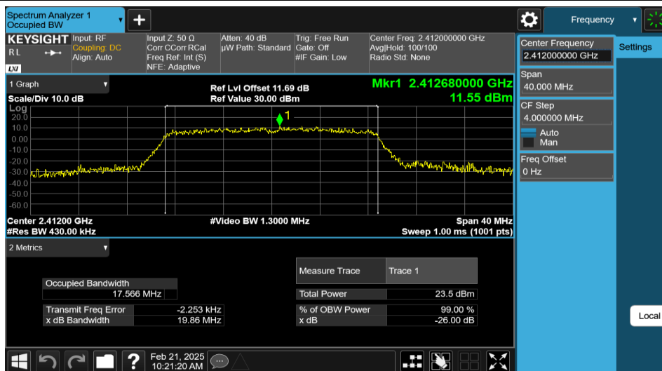
11N20MIMO-Ant2-2412
