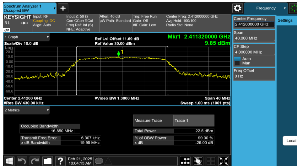
11G-Ant2-2412
