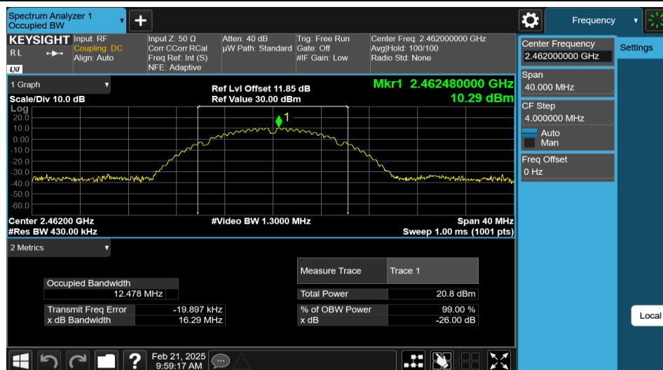
11B-Ant2-2462
