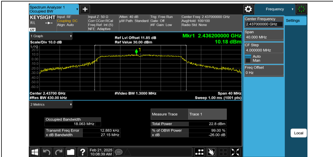
11G-Ant2-2437
