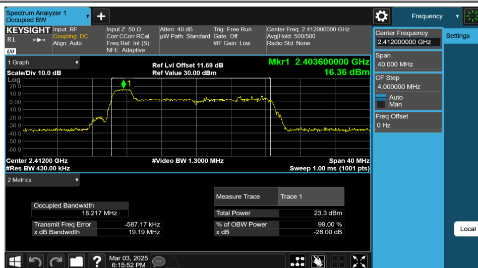
11AX20MIMO-Ant2-2412-26Tone-RU0
