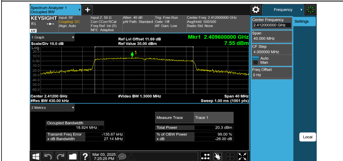
11AX20MIMO-Ant2-2412-242Tone-RU61
