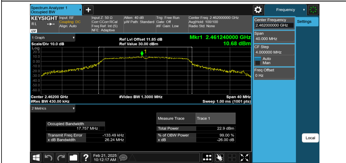
11G-Ant2-2462
