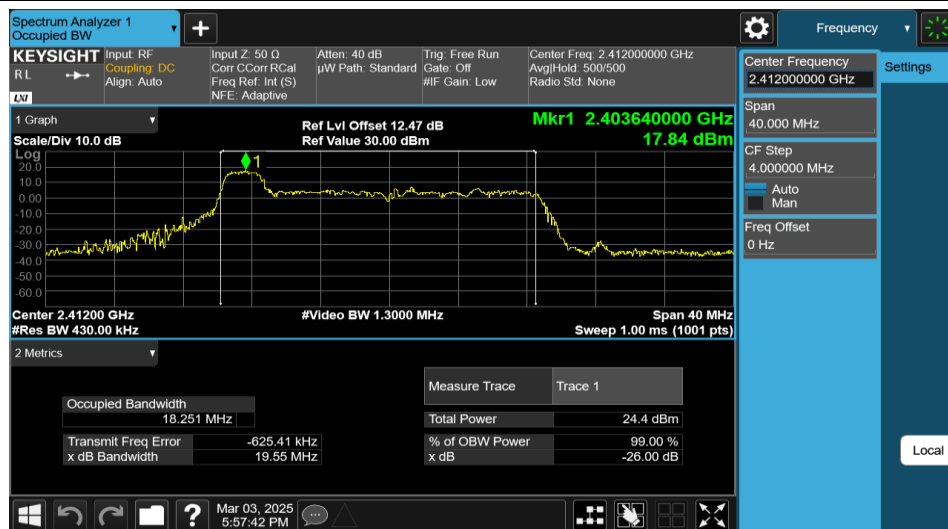
11AX20MIMO-Ant1-2412-26Tone-RU0
