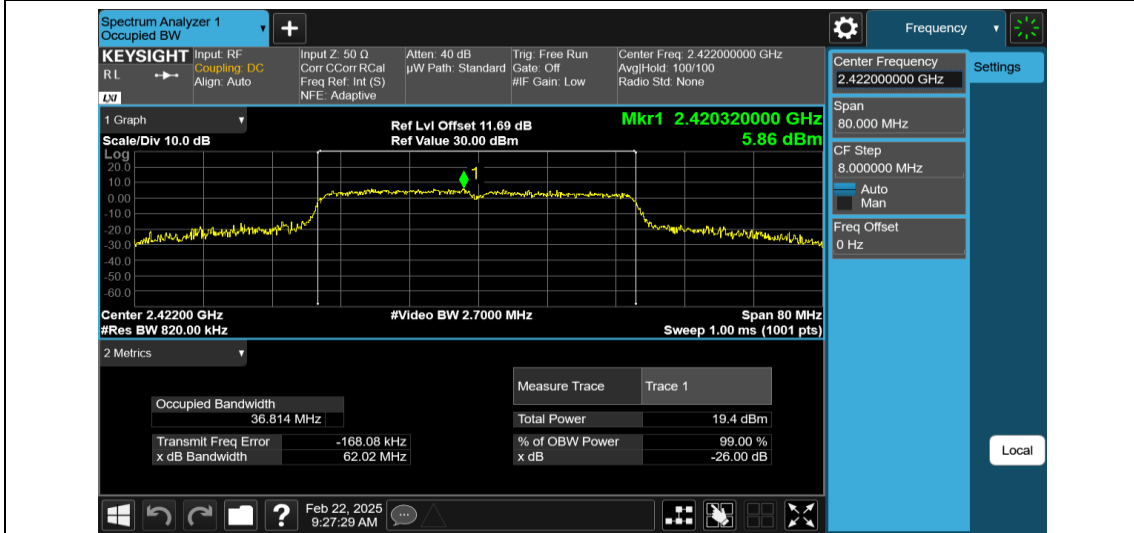
11N40MIMO-Ant2-2422
