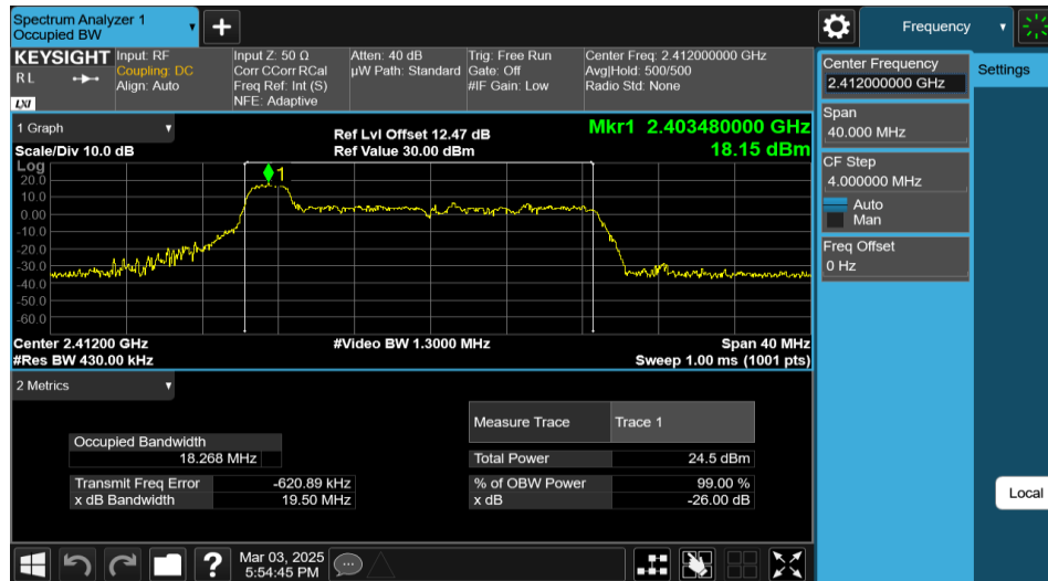
11AX20ISO-Ant1-2412-26Tone-RU0
