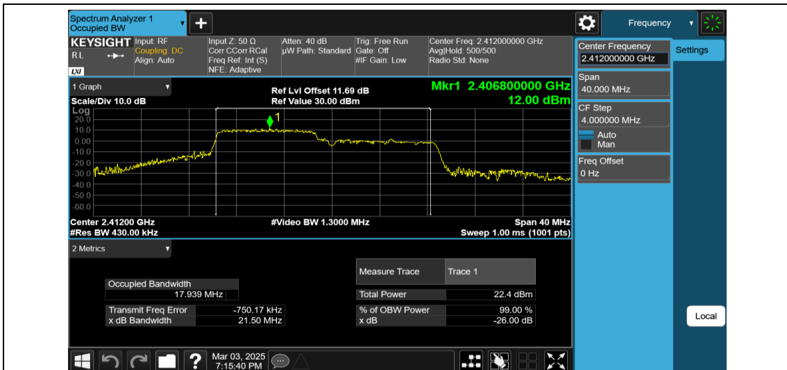
11AX20MIMO-Ant2-2412-106Tone-RU53
