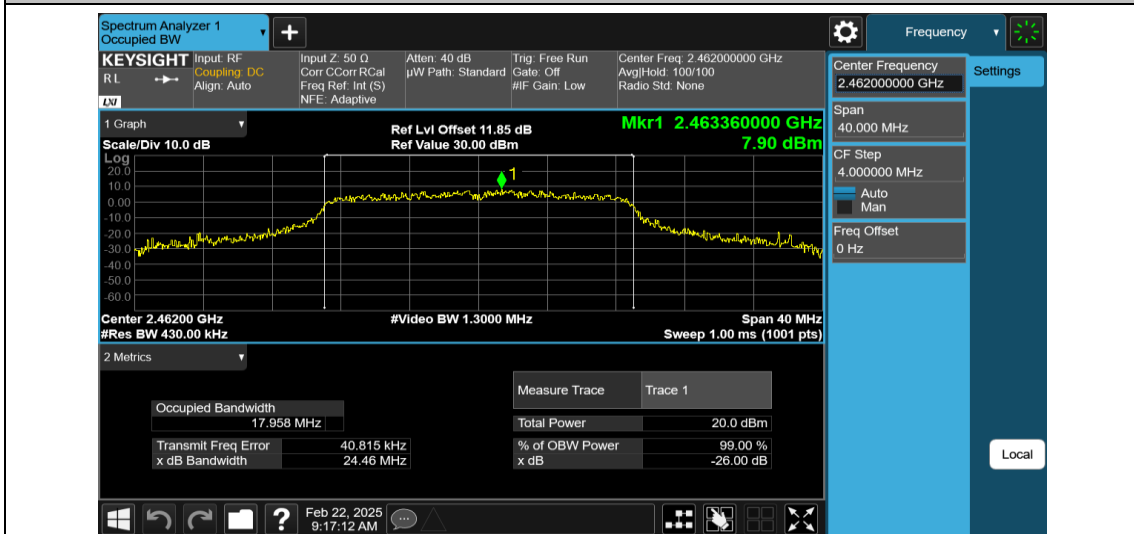
11N20MIMO-Ant2-2462
