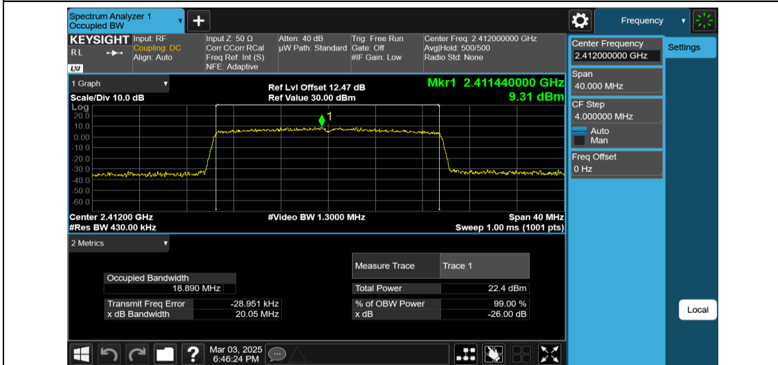
11AX20MIMO-Ant1-2412-242Tone-RU61
