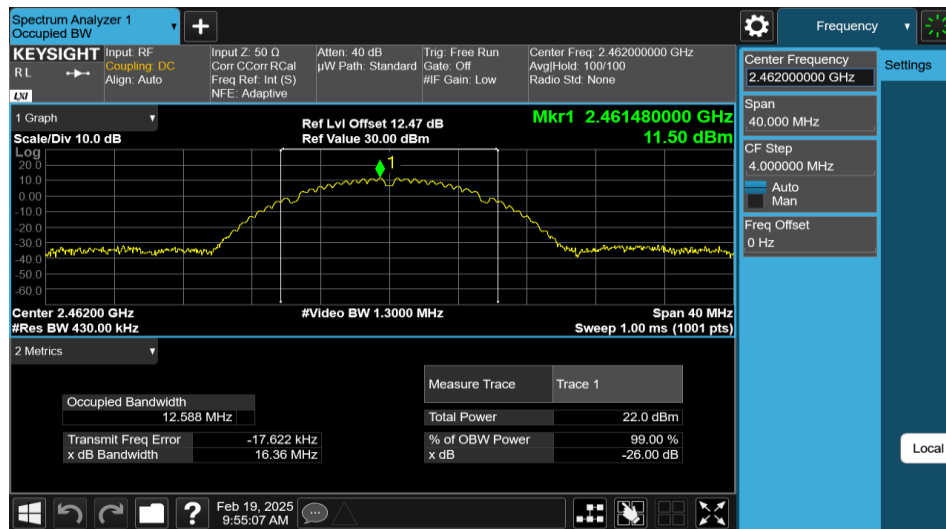
11B-Ant1-2462
