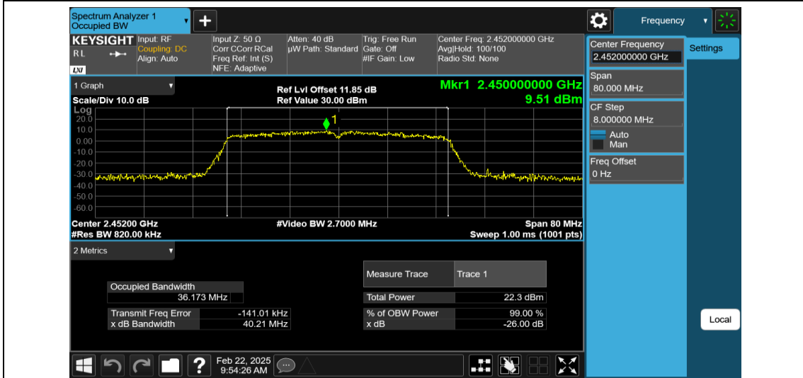
11N40MIMO-Ant2-2452
