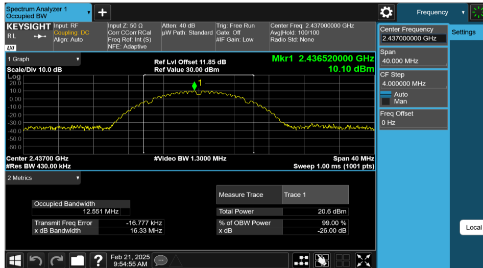
11B-Ant2-2437
