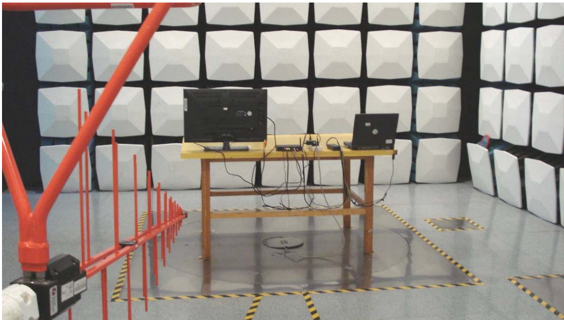
Spurious Emissions Test Setup - Rear View (Below 1GHz)
