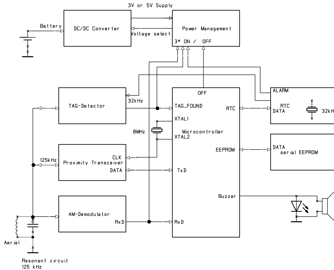
Block Diagram ProxiPen
