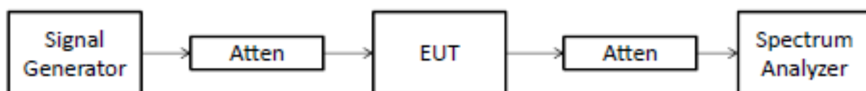
Figure 7.4.1 Out-of-band rejection test setup
