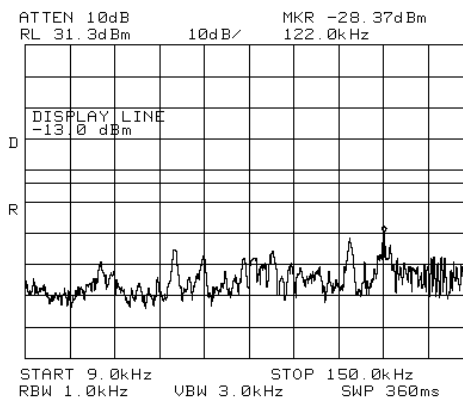
Figure 161.— 2112.50 MHz W-CDMA
