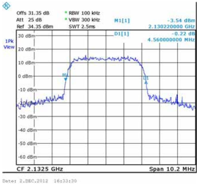
Figure 108.— W-CDMA (2132.5 MHz) OUT
