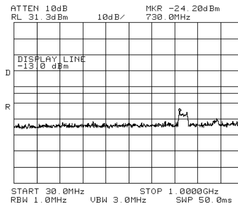
Figure 143.— 2132.50 MHz LTE
