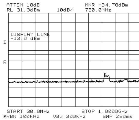
Figure 157.— 2112.50 MHz W-CDMA
