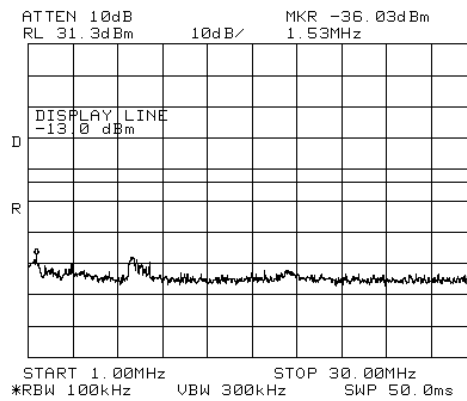
Figure 149.— 2150.00 MHz LTE
