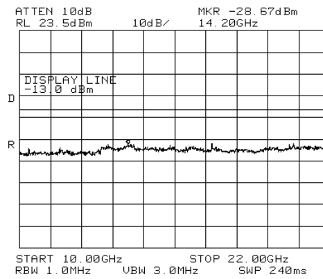
Figure 194 Intermodulation
