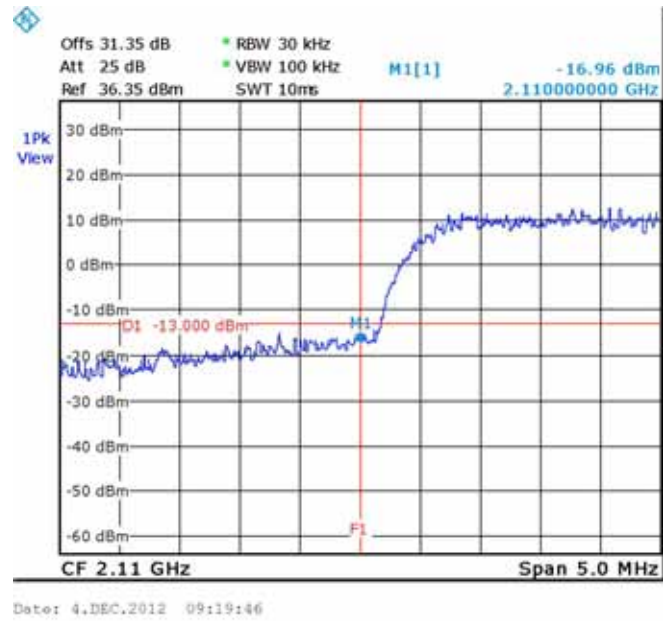
Figure 186.— W-CDMA 2112.50 MHz
