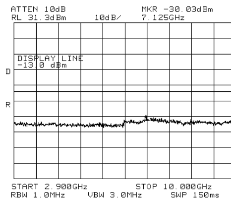
Figure 159.— 2112.50 MHz W-CDMA
