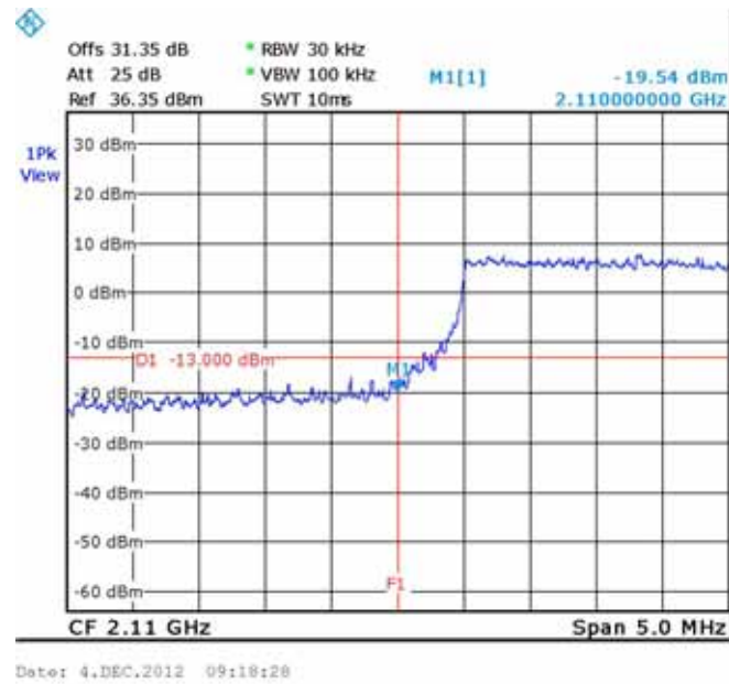
Figure 180.— LTE 64QAM 2115.00 MHz
