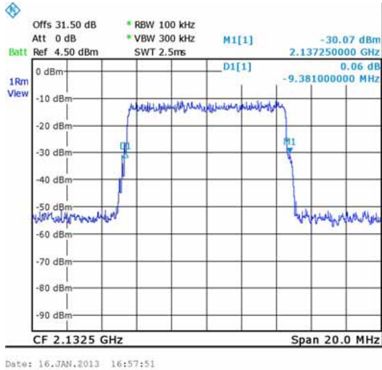
Figure 101.— LTE QPSK (2132.5 MHz) IN
