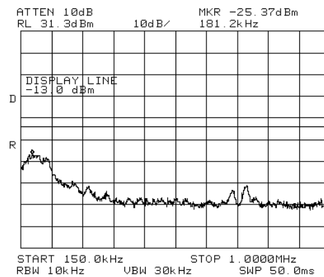
Figure 155.— 2112.50 MHz W-CDMA
