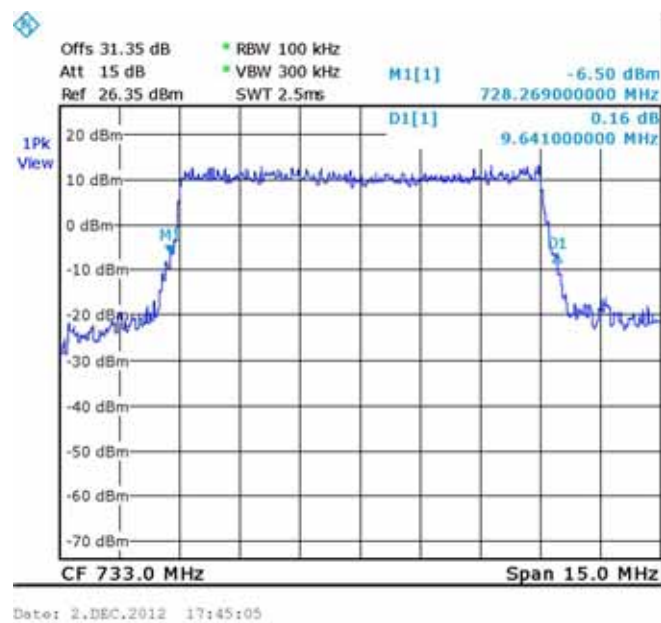
Figure 16.— 64QAM 733 MHz IN
