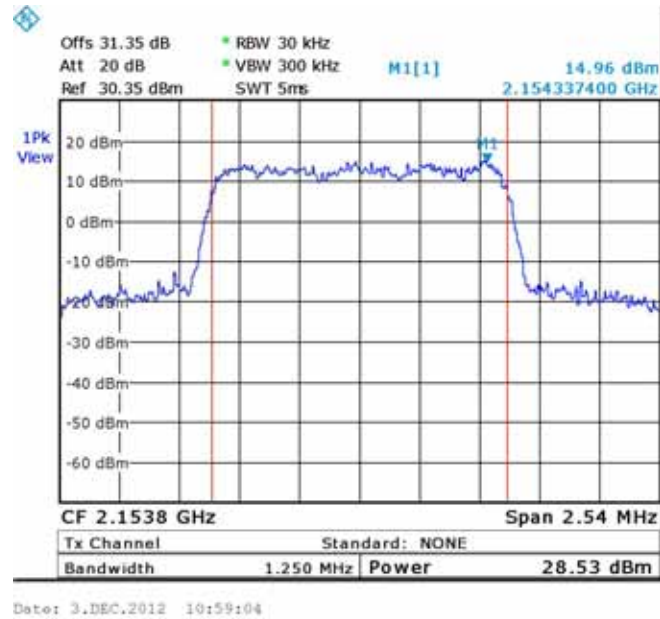
Figure 66.— CDMA (2153.8 MHz)
