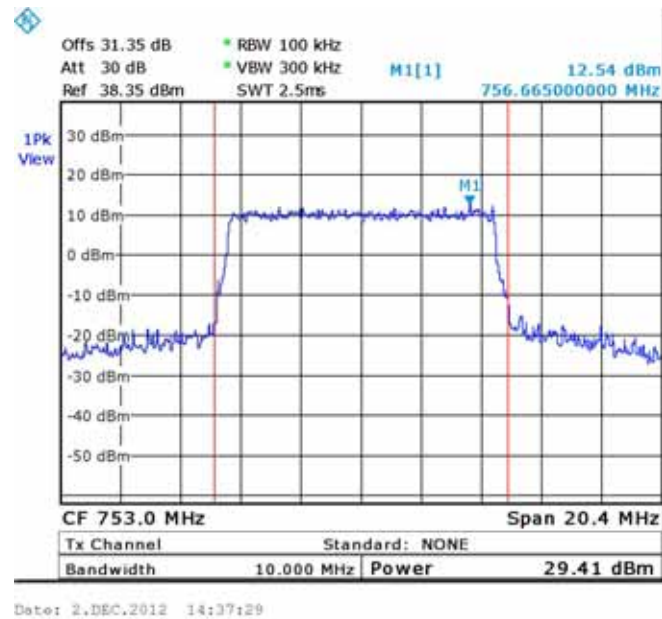
Figure 7.— 64QAM 753 MHz
