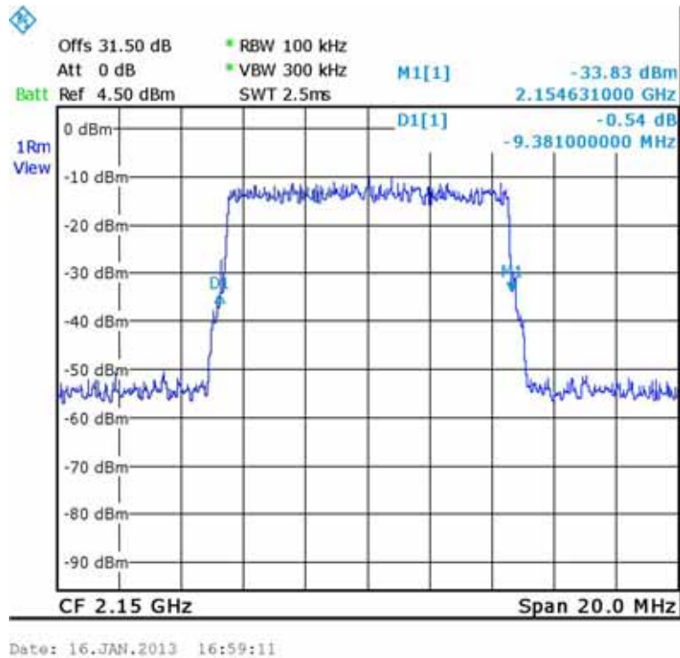
Figure 103.— LTE QPSK (2150.0 MHz) IN
