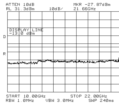
Figure 139.— 2115.00 MHz LTE
