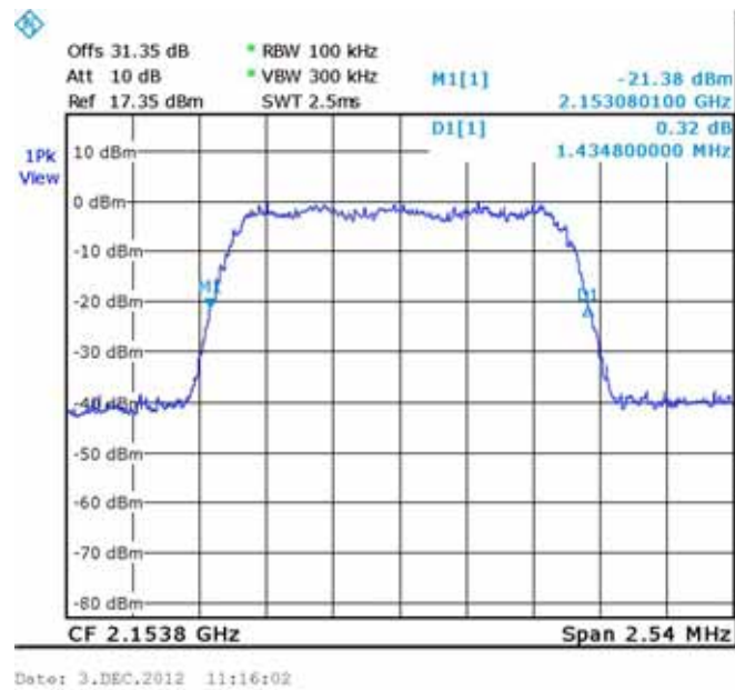
Figure 85.— CDMA (2153.8 MHz) IN
