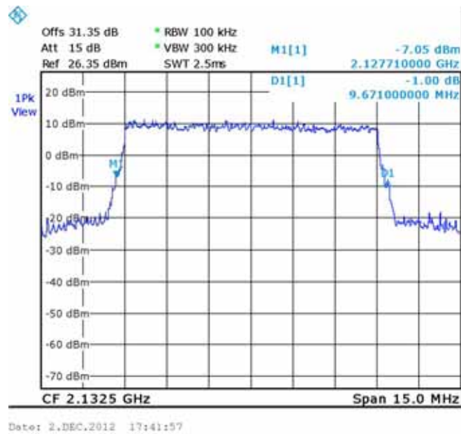
Figure 90.— LTE 64QAM (2132.5 MHz) OUT
