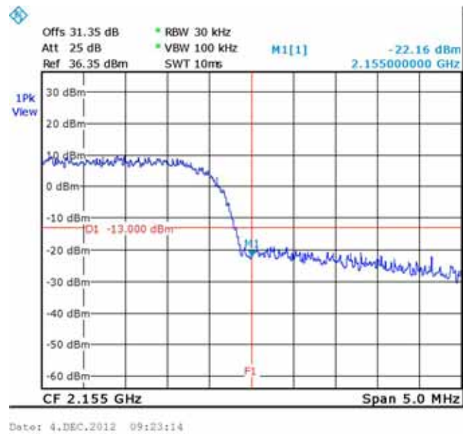
Figure 187.— W-CDMA 2152.50 MHz
