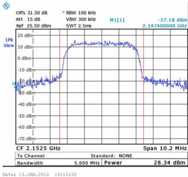
Figure 78.— W-CDMA (2152.5 MHz)
