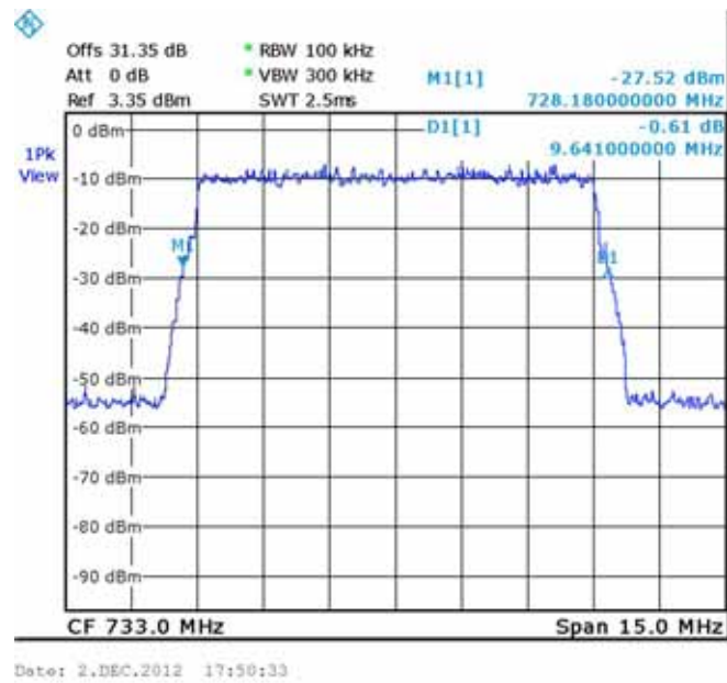
Figure 16.— 64QAM 733 MHz IN
