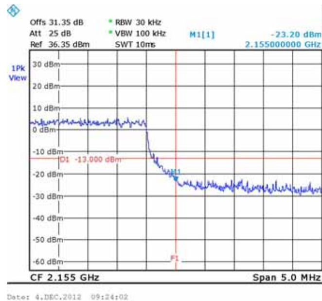
Figure 181.— LTE 64QAM 2150.00 MHz
