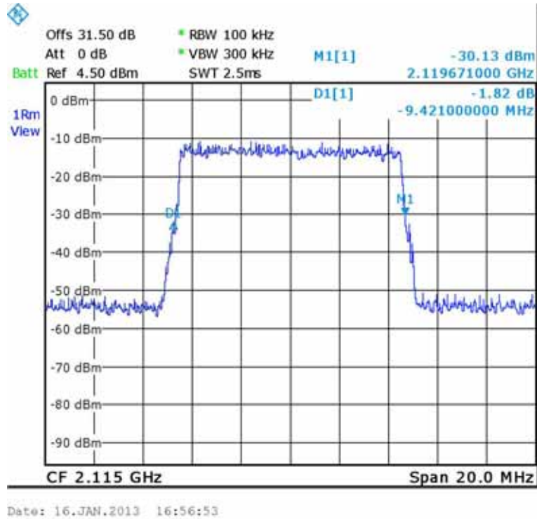
Figure 93.— LTE 16QAM (2115.0 MHz) IN
