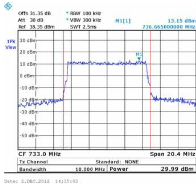
Figure 5.— 64QAM, 733 MHz
