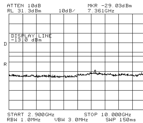
Figure 131.— 2153.80 MHz CDMA
