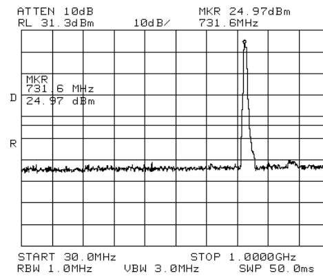
Figure 38.— 733 MHz
