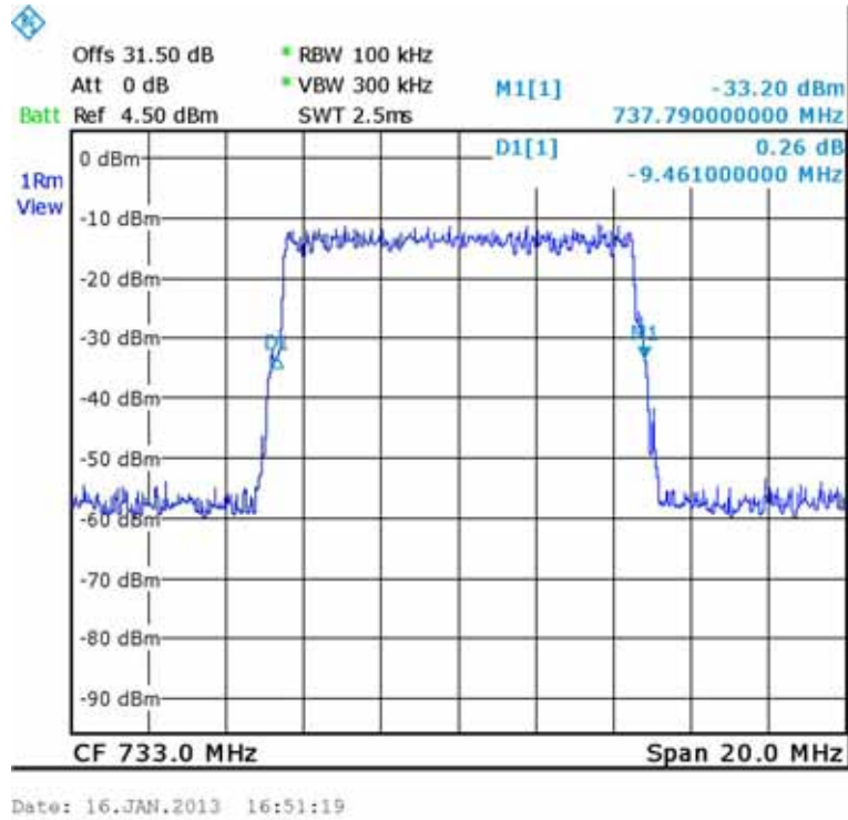
Figure 28.— QPSK 733 MHz IN
