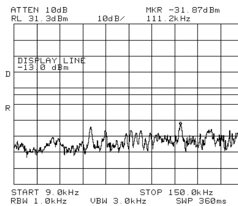
Figure 147.— 2132.50 MHz LTE
