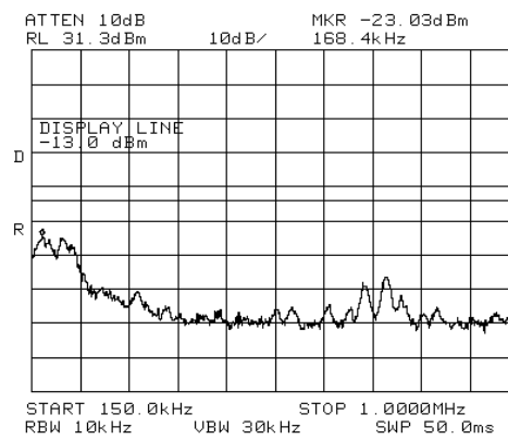
Figure 141.— 2132.50 MHz LTE
