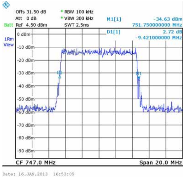
Figure 24.— 16QAM 747 MHz IN
