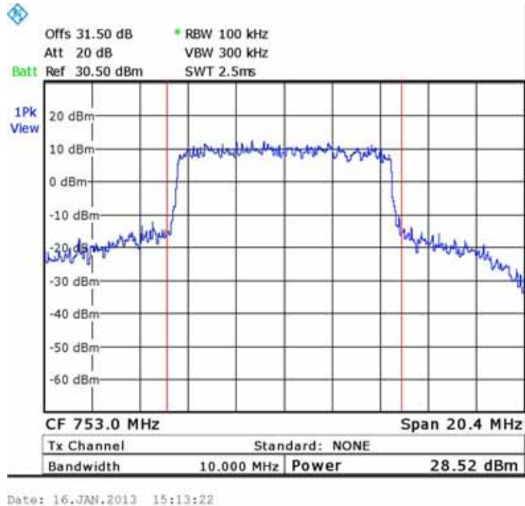
Figure 13.— QPSK 753 MHz
