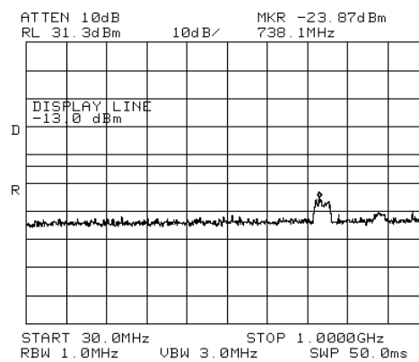
Figure 171.— 2152.50 MHz W-CDMA
