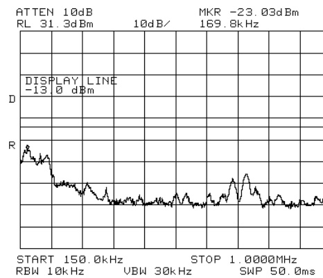
Figure 169.— 2152.50 MHz W-CDMA
