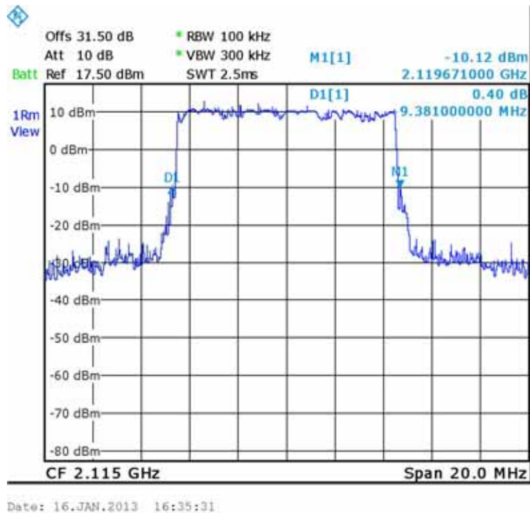
Figure 94.— LTE 16QAM (2115.0 MHz) OUT
