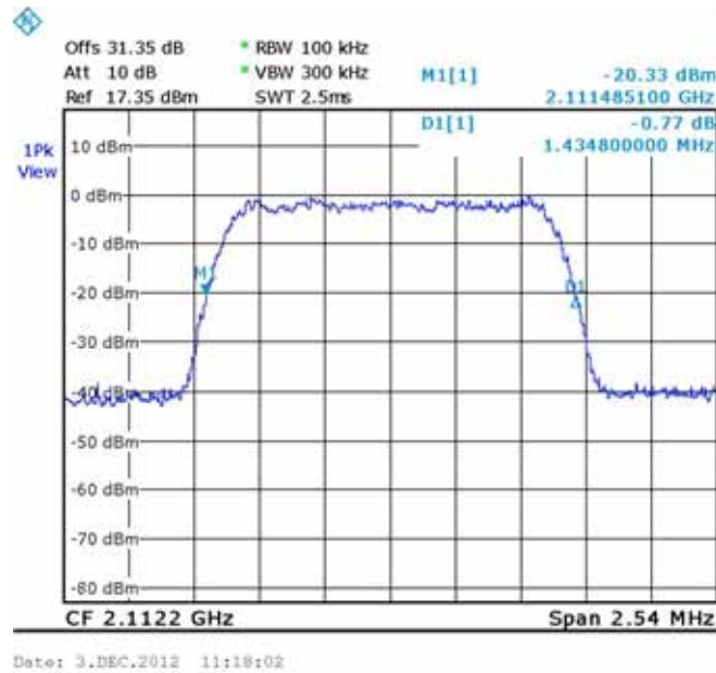
Figure 81.— CDMA (2112.2 MHz) IN
