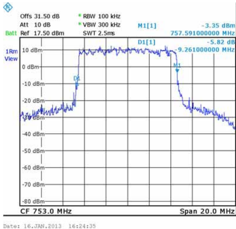
Figure 32.— QPSK 753 MHz IN
