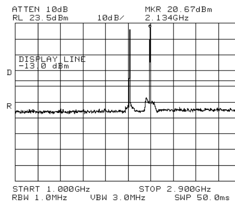
Figure 192 Intermodulation
