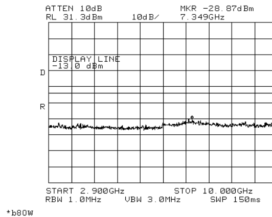
Figure 173.— 2152.50 MHz W-CDMA
