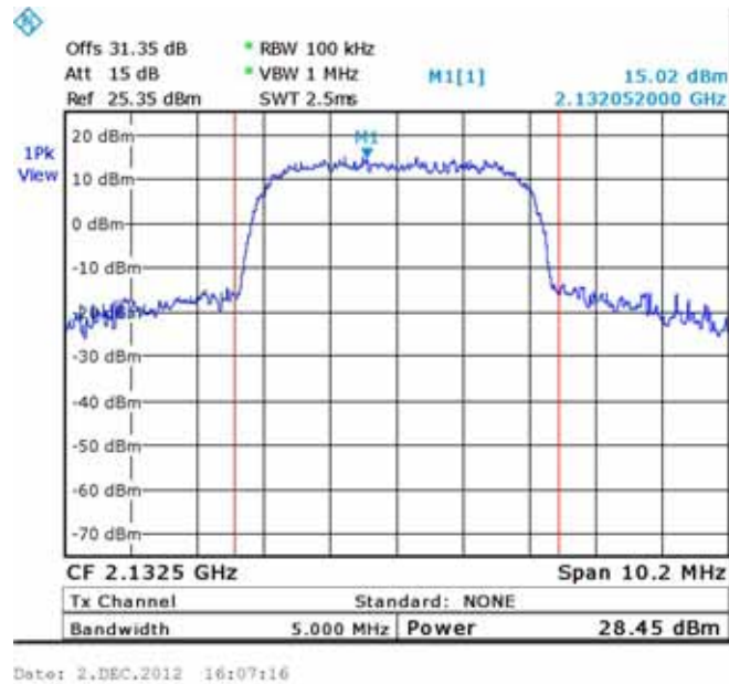
Figure 77.— W-CDMA (2132.5 MHz)
