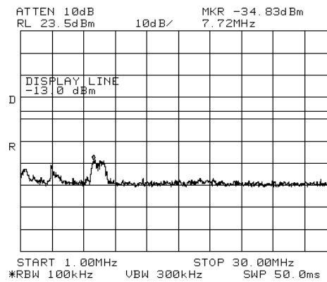
Figure 190 Intermodulation
