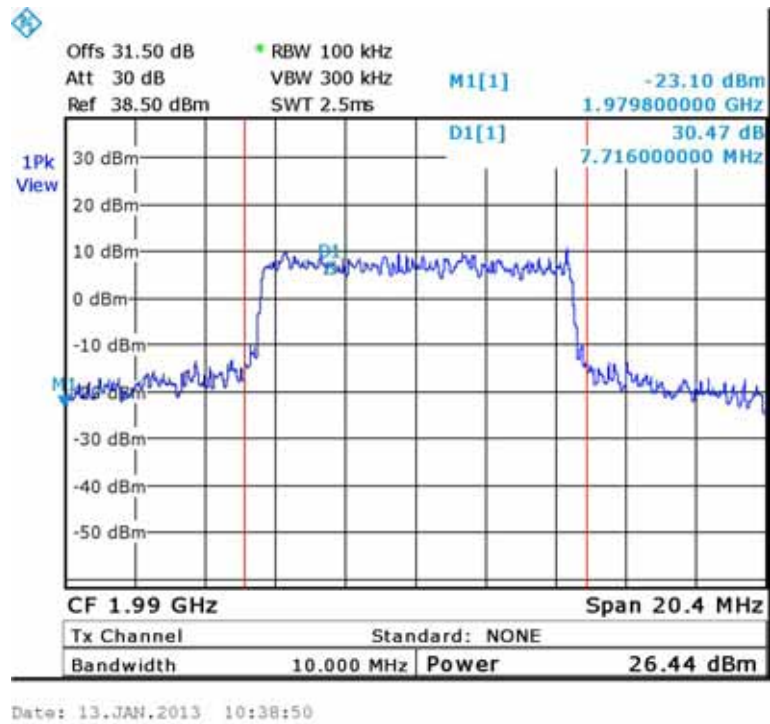
Figure 126.— 64QAM 1990.00 MHz
