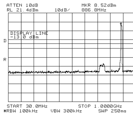
Figure 68.— 889.00 MHz
