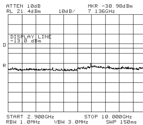
Figure 70.— 889.00 MHz
