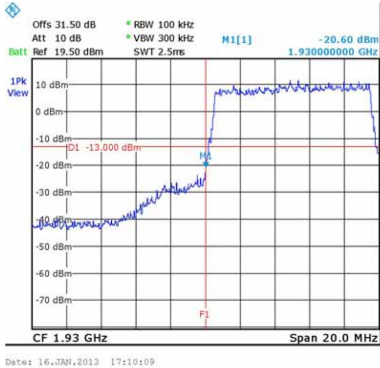
Figure 242.— QPSK 1935.00 MHz
