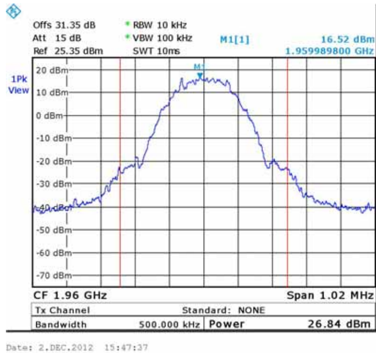
Figure 134.— 1960.00 MHz
