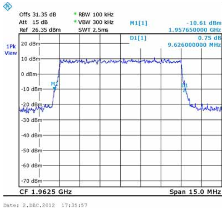
Figure 144.— 64QAM Output 1962.50 MHz
