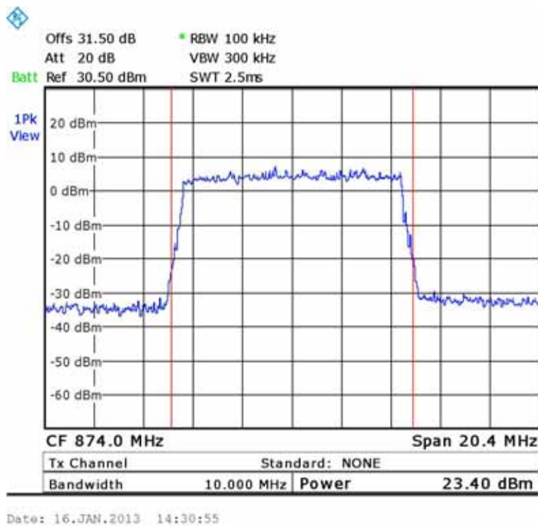
Figure 8.— 874.00 MHz
