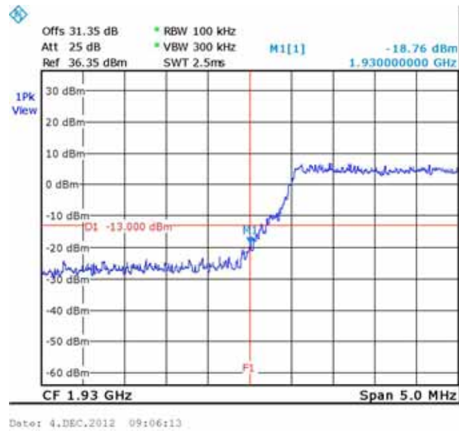
Figure 238.— 64QAM 1935.00 MHz
