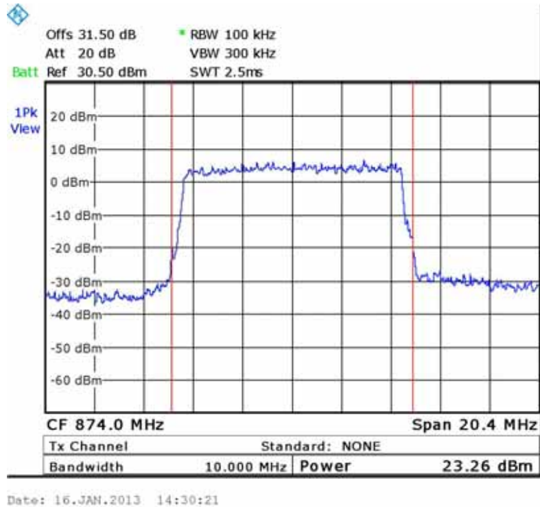
Figure 5.— 874.00 MHz
