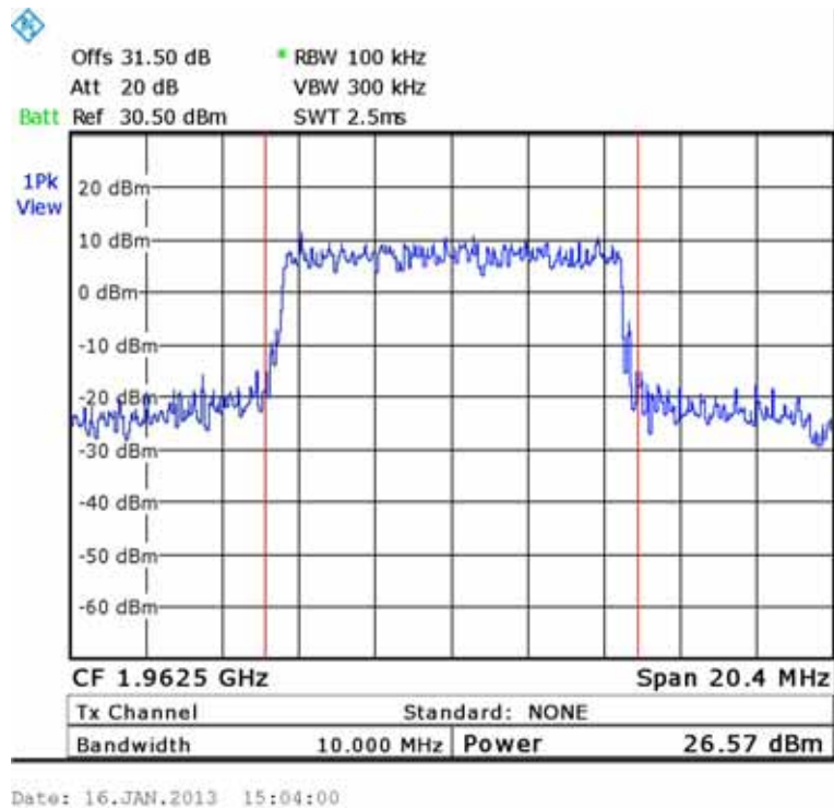
Figure 131.— QPSK 1962.50 MHz
