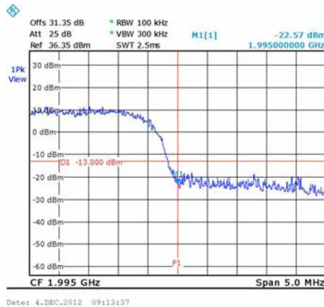
Figure 247.— 1992.50 MHz
