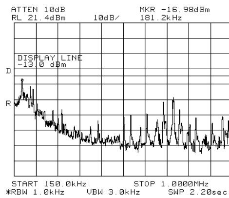
Figure 78.— 881.00 MHz
