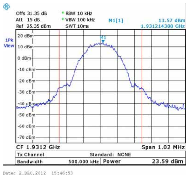
Figure 133.— 1931.20 MHz
