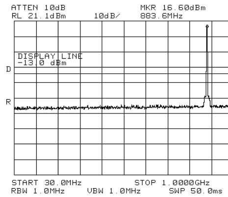
Figure 252 Intermodulation
