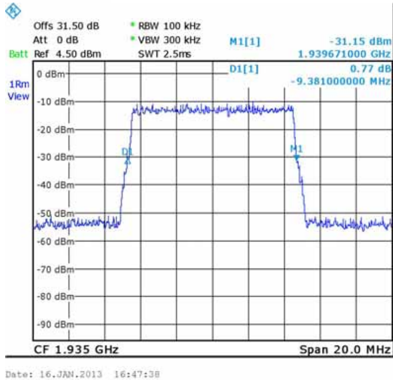
Figure 147.— 16QAM Input 1935.00 MHz
