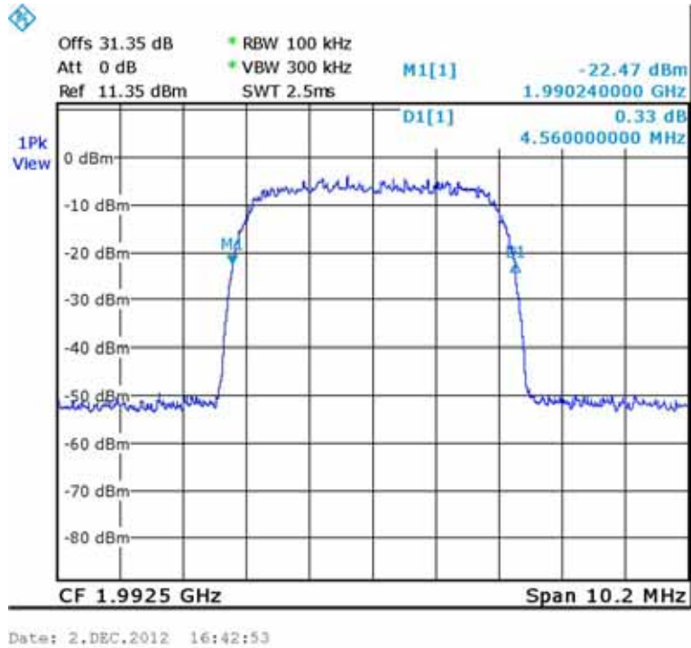
Figure 169.— Input 1992.50 MHz
