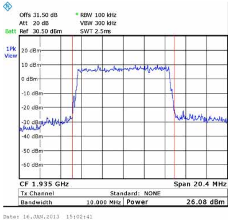
Figure 130.— QPSK 1935.00 MHz
