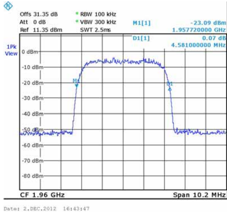
Figure 167.— Input 1960.00 MHz
