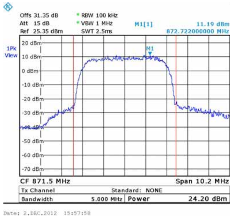
Figure 17.— 871.50 MHz
