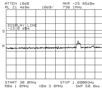
Figure 231.— 1992.50 MHz
