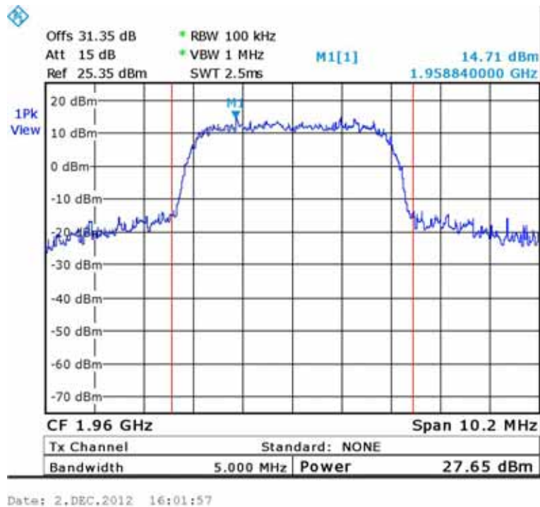
Figure 137.— 1960.00 MHz
