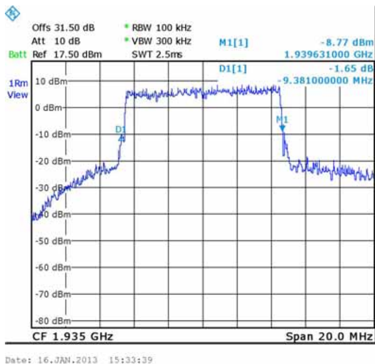
Figure 153.— QPSK Input 1935.00 MHz
