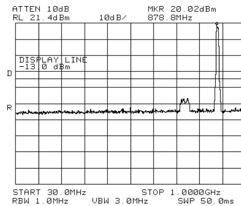
Figure 62.— 881.00 MHz
