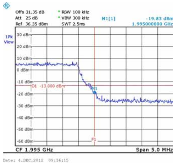
Figure 239.— 64QAM 1990.00 MHz
