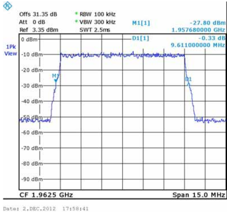
Figure 143.— 64QAM Input 1962.50 MHz
