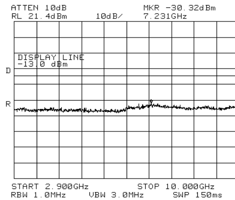
Figure 108.— 891.50 MHz
