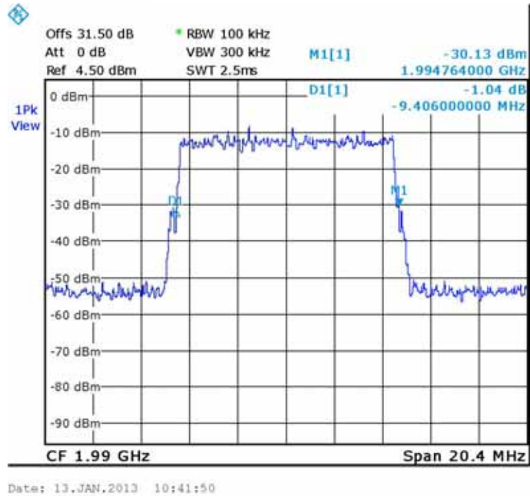
Figure 145.— 64QAM Input 1990.00 MHz
