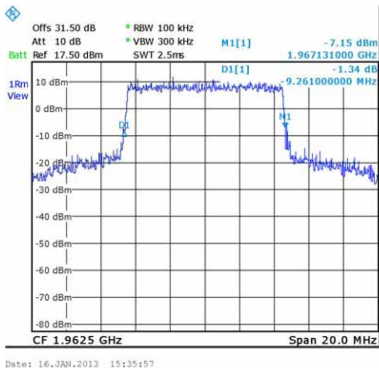
Figure 149.— 16QAM Input 1962.50 MHz
