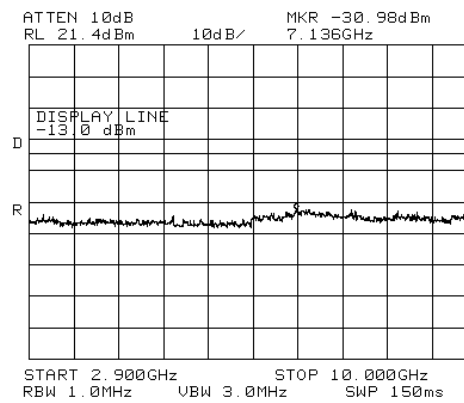
Figure 70.— 890.00 MHz
