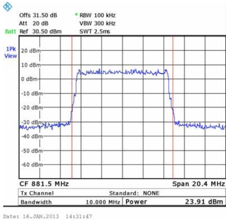
Figure 9.— 881.5 MHz
