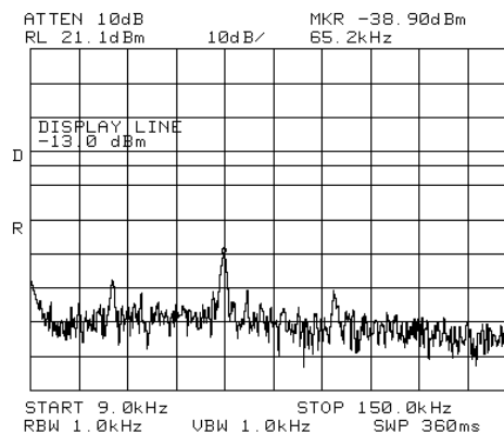
Figure 249 Intermodulation
