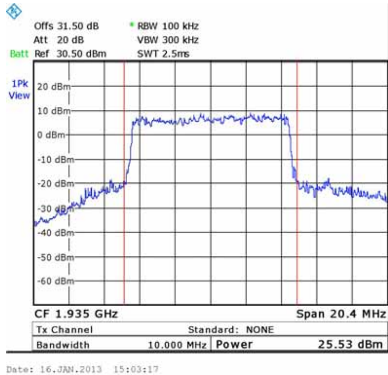
Figure 127.— 16QAM 1935.00 MHz
