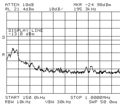
Figure 187.— 1990.00 MHz
