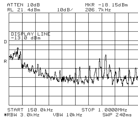
Figure 60.— 881.00 MHz
