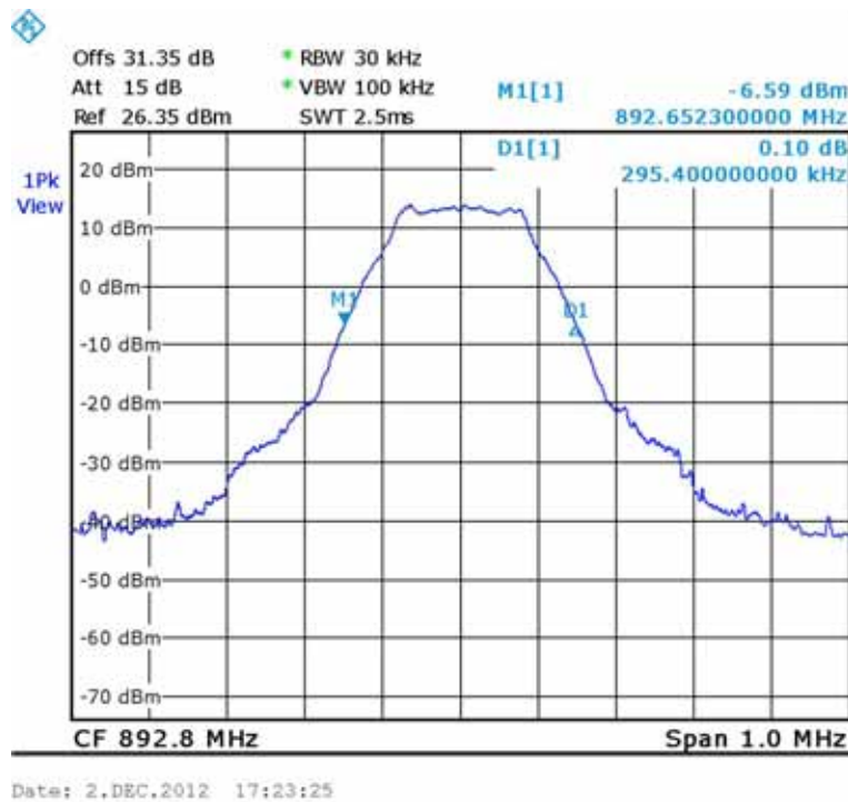
Figure 45.— Output 892.8 MHz.
