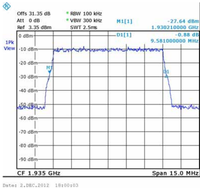
Figure 141.— 64QAM Input 1935.00 MHz
