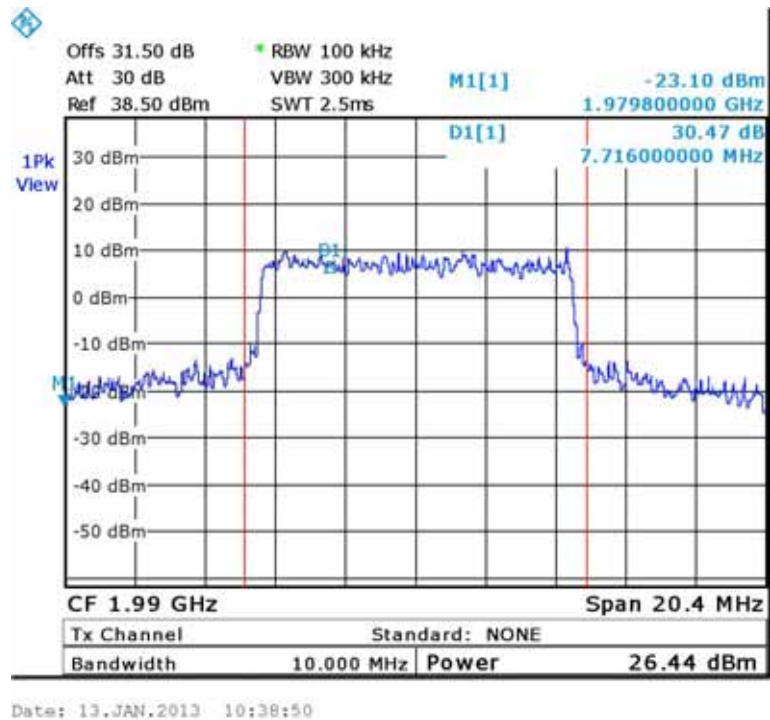
Figure 126.— 64QAM 1990.00 MHz
