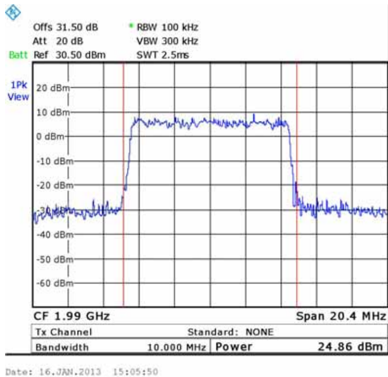
Figure 129.— 16QAM 1990.00 MHz
