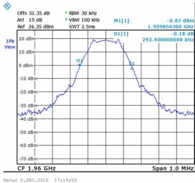
Figure 162.— Output 1960.00 MHz
