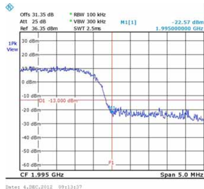
Figure 247.— 1992.50 MHz
