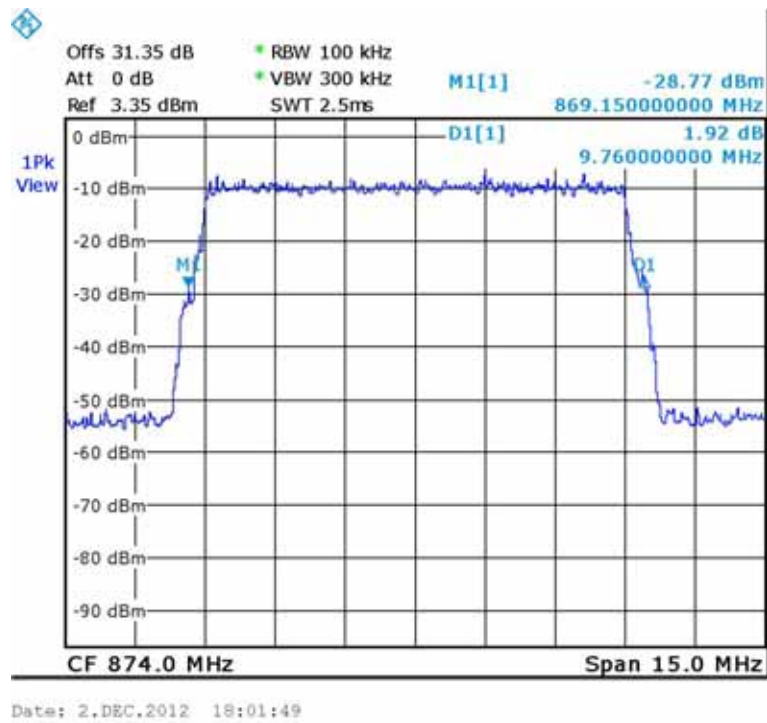
Figure 22.— 64QAM Input 874.00
