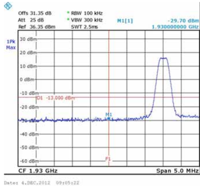
Figure 244.— 1931.20 MHz
