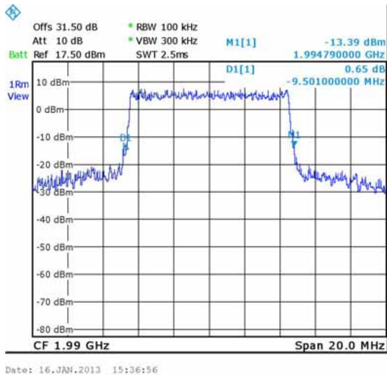
Figure 157.— QPSK Input 1990.00 MHz
