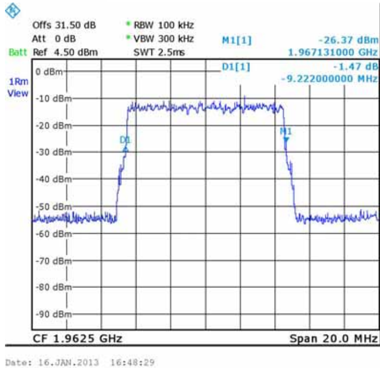
Figure 155.— QPSK Input 1962.50 MHz
