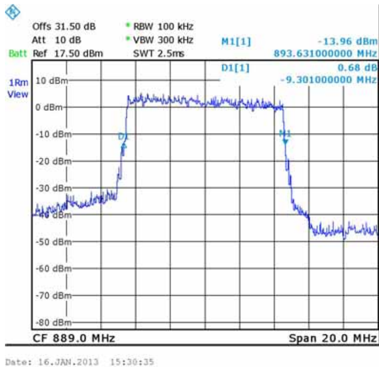
Figure 39.— QPSK Output 889.00 MHz.
