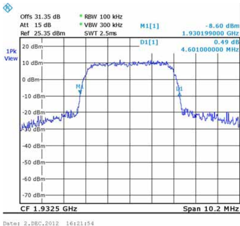
Figure 165.— Input 1932.50 MHz
