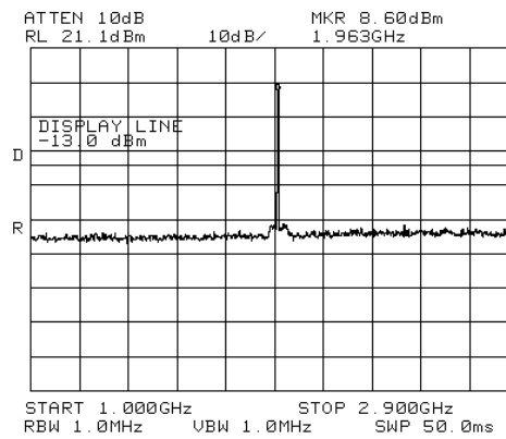
Figure 253 Intermodulation
