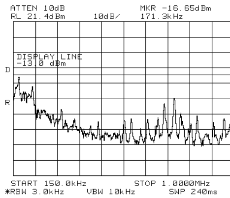
Figure 90.— 871.50 MHz
