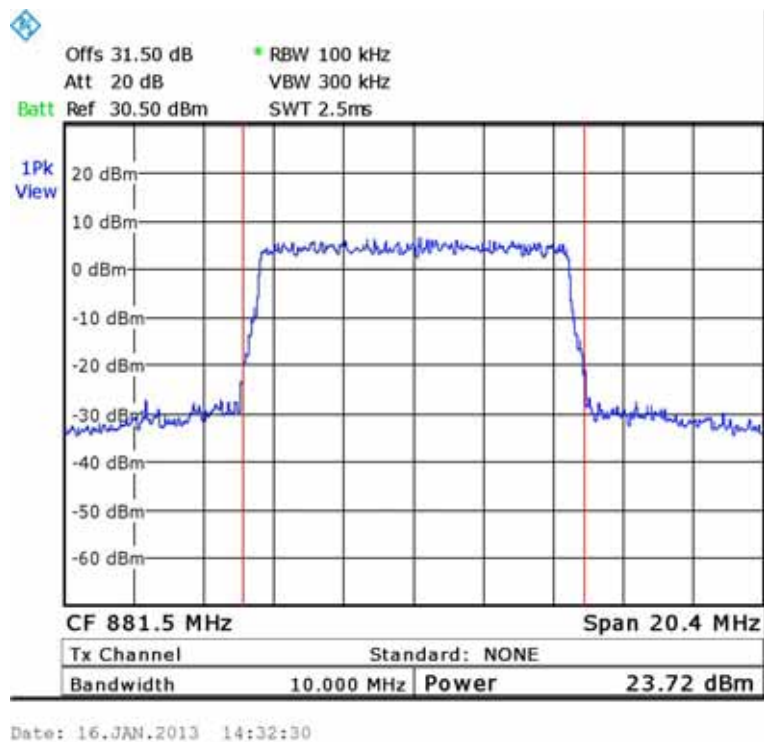
Figure 6.— 881.50 MHz
