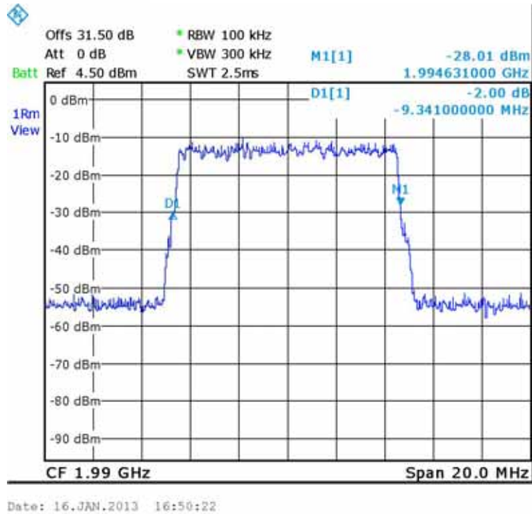
Figure 151.— 16QAM Input 1990.00 MHz
