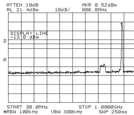
Figure 68.— 890.00 MHz
