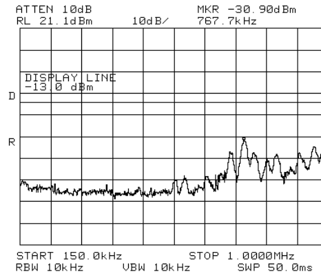
Figure 250 Intermodulation
