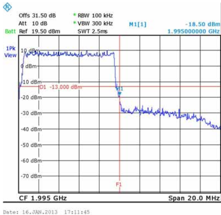
Figure 241.— 16QAM 1990.00 MHz
