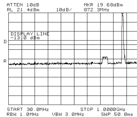
Figure 56.— 874.00 MHz
