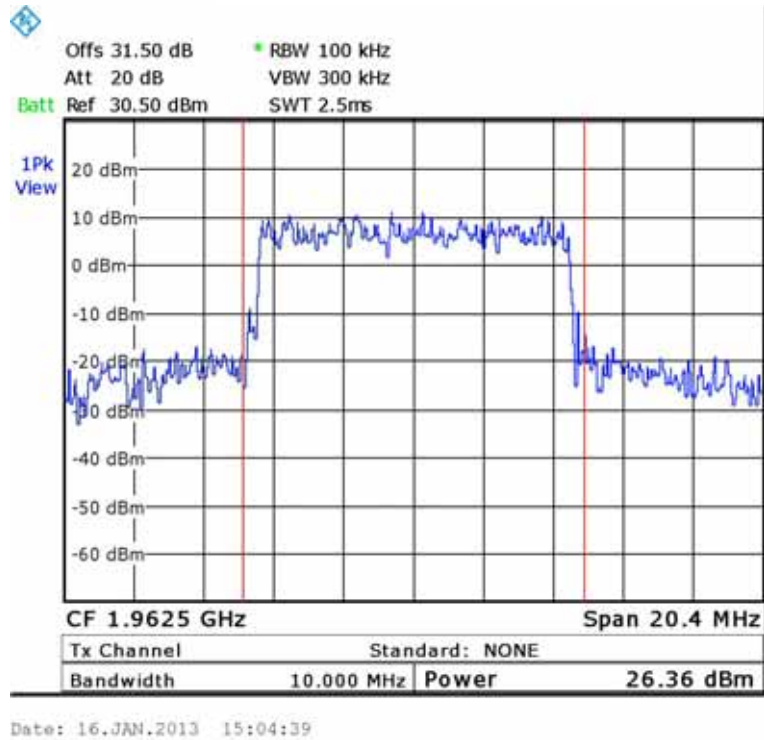
Figure 128.— 16QAM 1962.50 MHz
