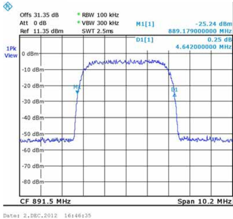
Figure 50.— Input 891.50 MHz.
