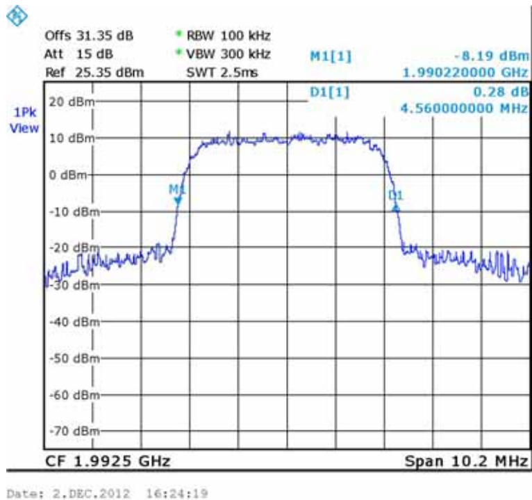
Figure 170.— Output 1992.50 MHz
