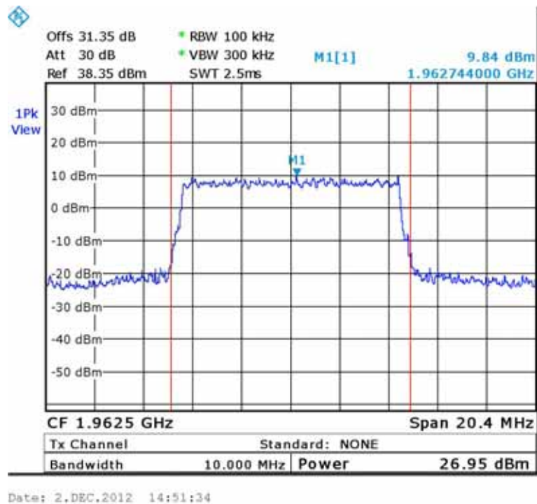
Figure 125.— 64QAM 1962.50 MHz
