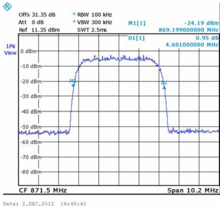
Figure 46.— Input 871.50
