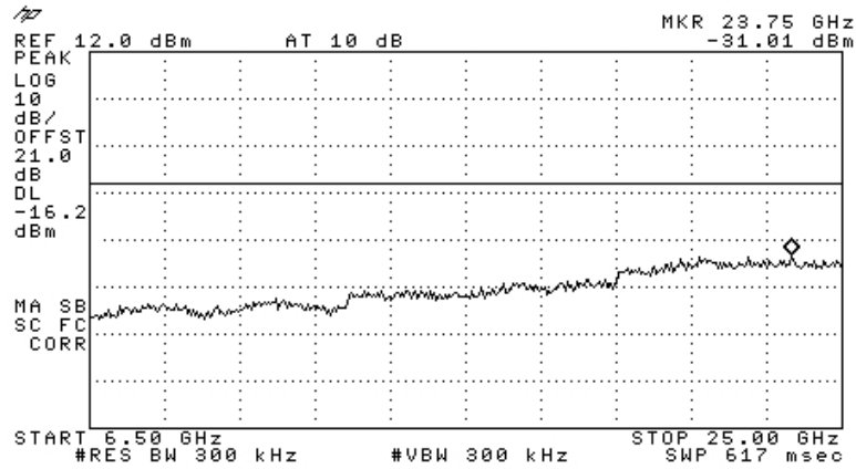
Figure 72 —2437 MHz DBPSK
