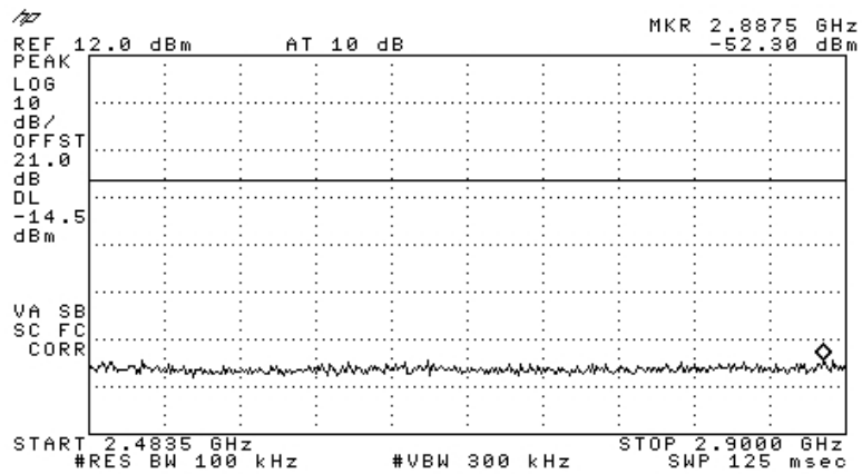
Figure 42 —2412 MHz DBPSK
