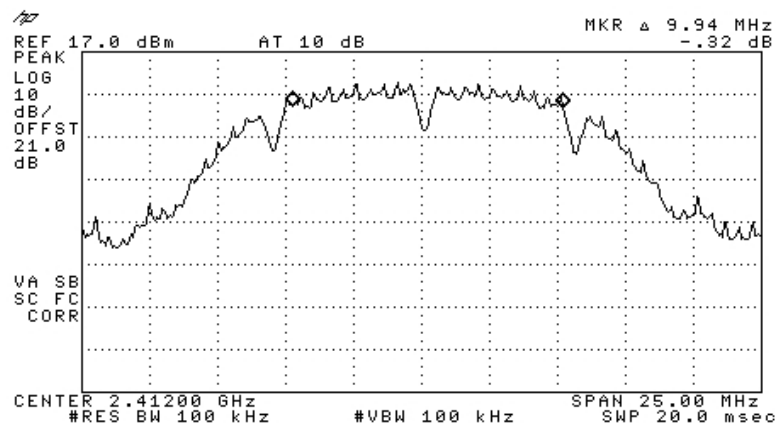
Figure 125 —2412 MHz DBPSK
