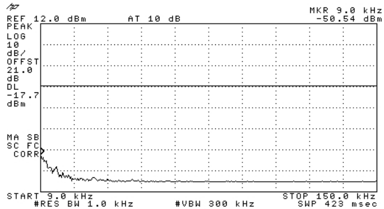
Figure 60 —2412 MHz 64QAM
