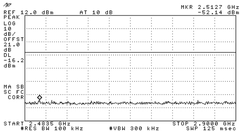
Figure 70 —2437 MHz DBPSK
