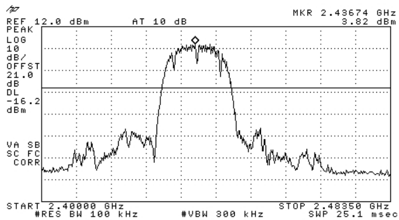
Figure 67 —2437 MHz DBPSK
