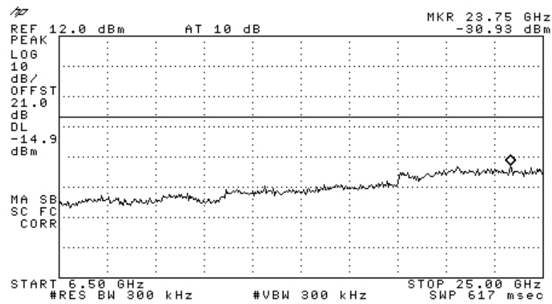
Figure 58 —2412 MHz CCK
