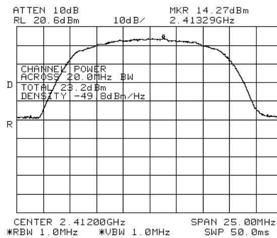
Figure 26 2412 MHz BPSK
