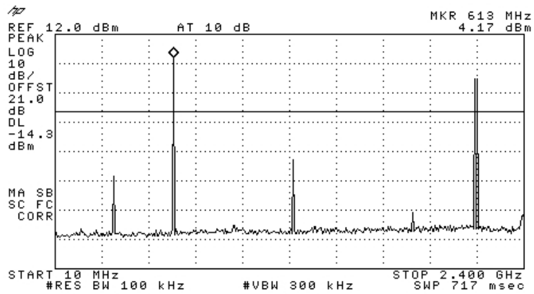
Figure 118 —2462 MHz 64QAM
