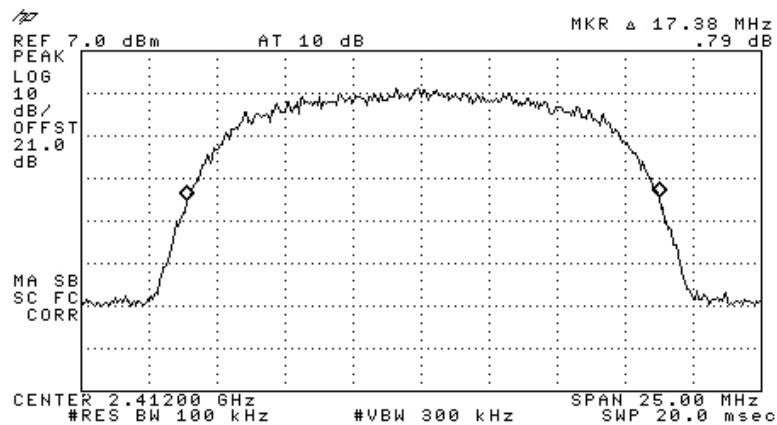
Figure 13 —2412 MHz BPSK
