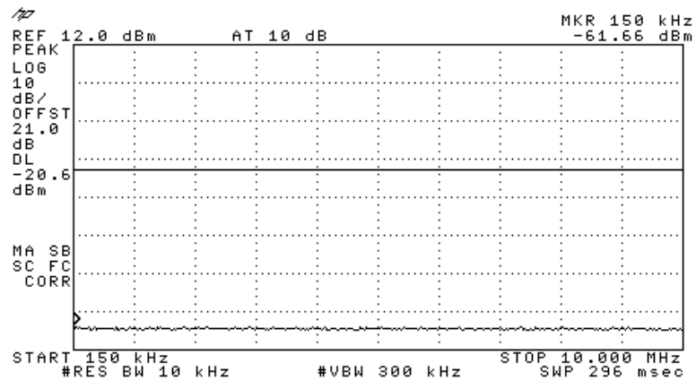
Figure 110 —2462 MHz CCK
