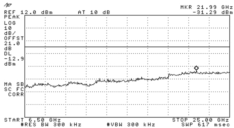
Figure 86 —2437 MHz CCK
