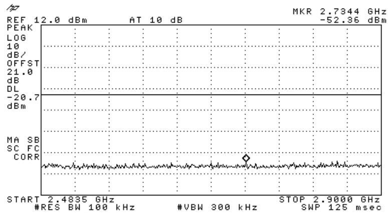
Figure 98 —2462 MHz DBPSK
