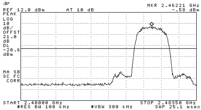
Figure 108 —2462 MHz BPSK
