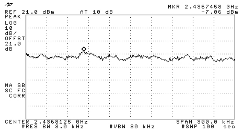
Figure 155 —2437 MHz CCK
