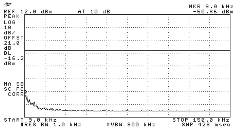
Figure 75 —2437 MHz BPSK
