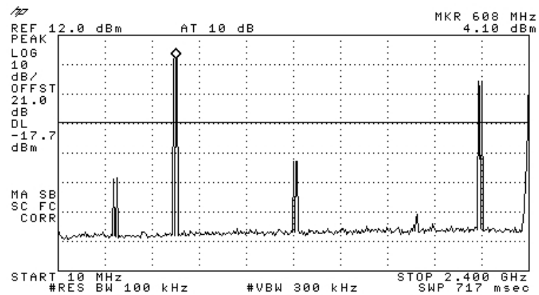
Figure 62 —2412 MHz 64QAM
