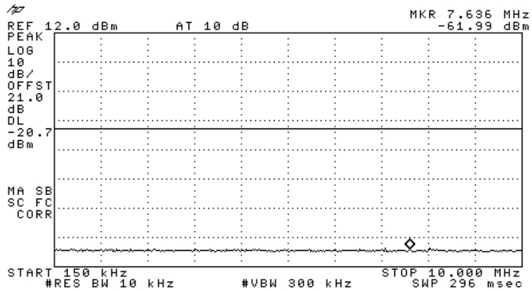
Figure 96 —2462 MHz DBPSK
