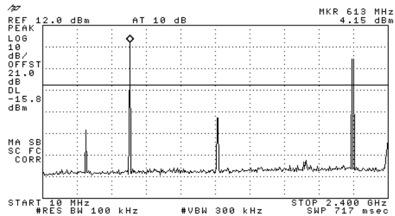
Figure 90 —2437 MHz 64QAM
