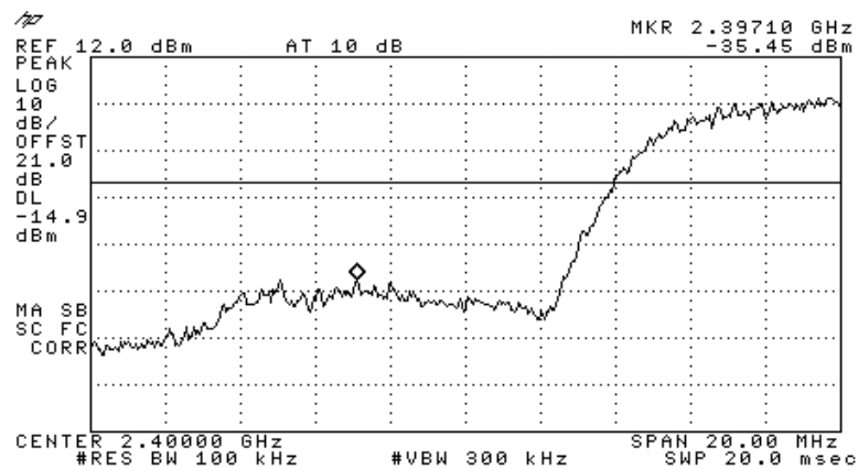
Figure 140 —2412 MHz BPSK
