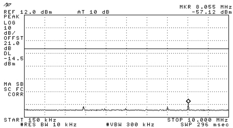
Figure 40 —2412 MHz DBPSK
