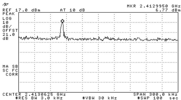
Figure 149 —2412 MHz DBPSK
