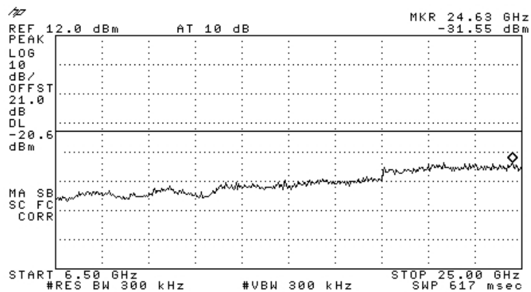
Figure 114 —2462 MHz CCK
