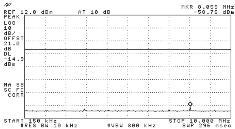
Figure 54 —2412 MHz CCK
