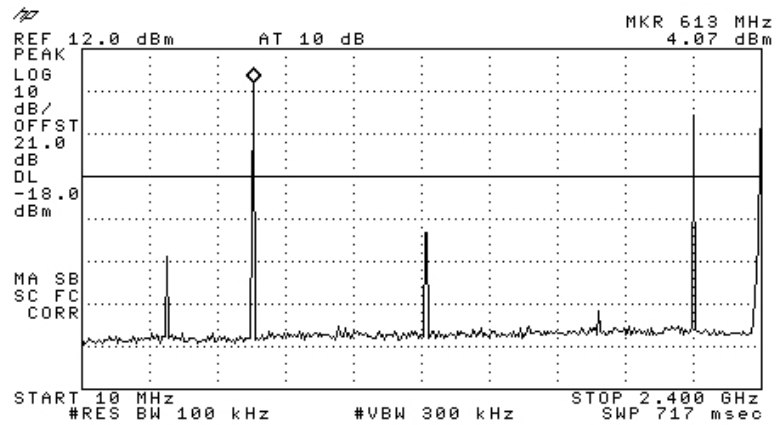
Figure 48 —2412 MHz BPSK
