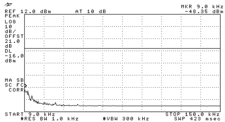
Figure 102 —2462 MHz BPSK
