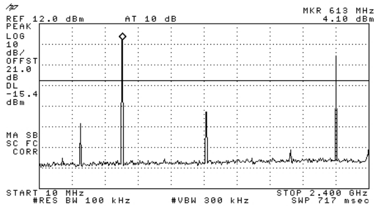
Figure 76 —2437 MHz BPSK
