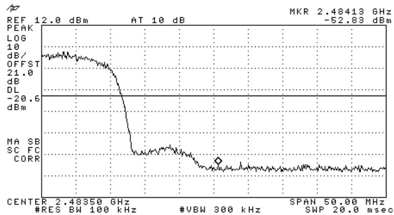
Figure 144 —2462 MHz BPSK
