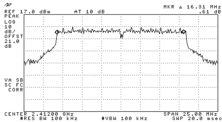
Figure 128 —2412 MHz 64QAM
