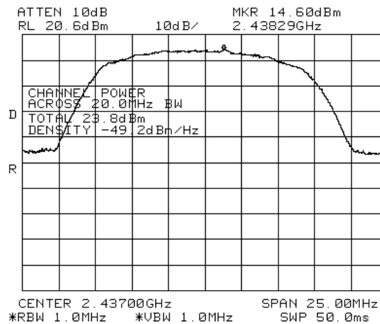
Figure 30 2437 MHz BPSK
