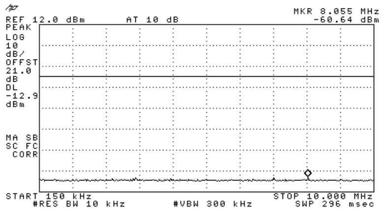
Figure 82 —2437 MHz CCK
