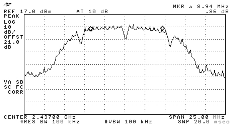
Figure 129 —2437 MHz DBPSK
