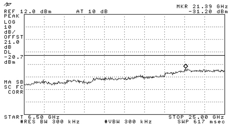
Figure 100 —2462 MHz DBPSK
