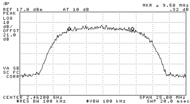
Figure 134 —2462 MHz BPSK
