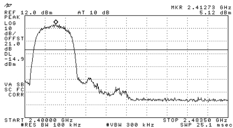
Figure 52 —2412 MHz BPSK
