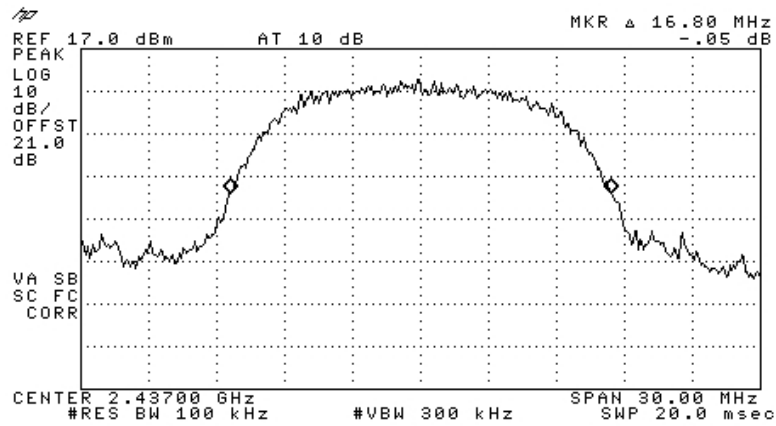
Figure 17 —2437 MHz BPSK
