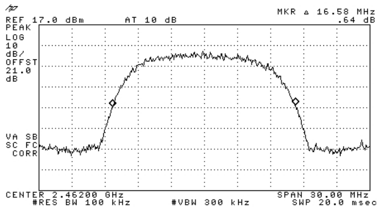
Figure 21 —2462 MHz BPSK
