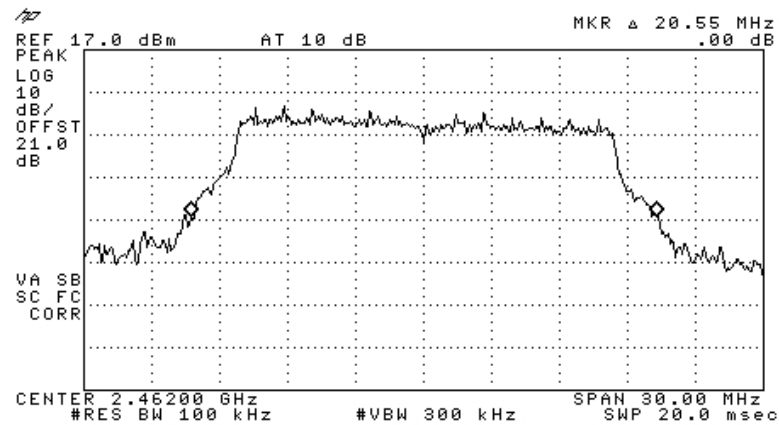
Figure 21 —2462 MHz BPSK
