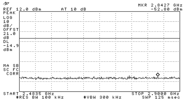
Figure 56 —2412 MHz CCK
