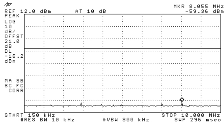
Figure 68 —2437 MHz DBPSK
