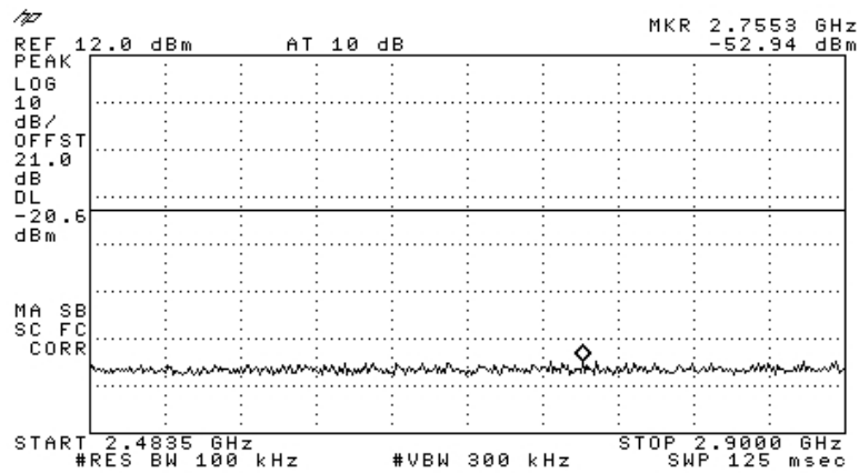
Figure 112 —2462 MHz CCK
