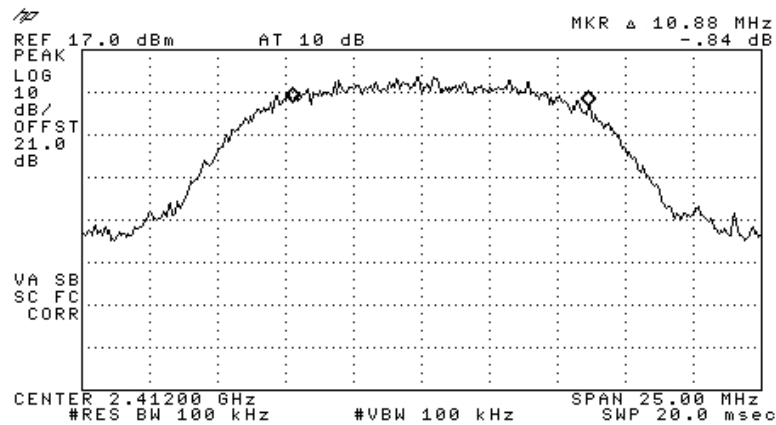
Figure 126 —2412 MHz BPSK
