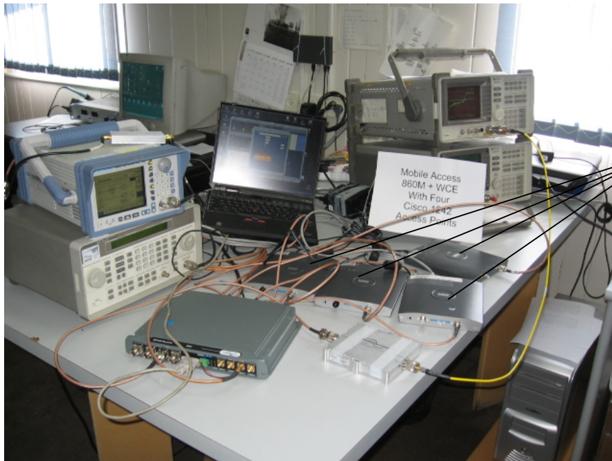
Conducted Tests on Antenna Ports Setup
