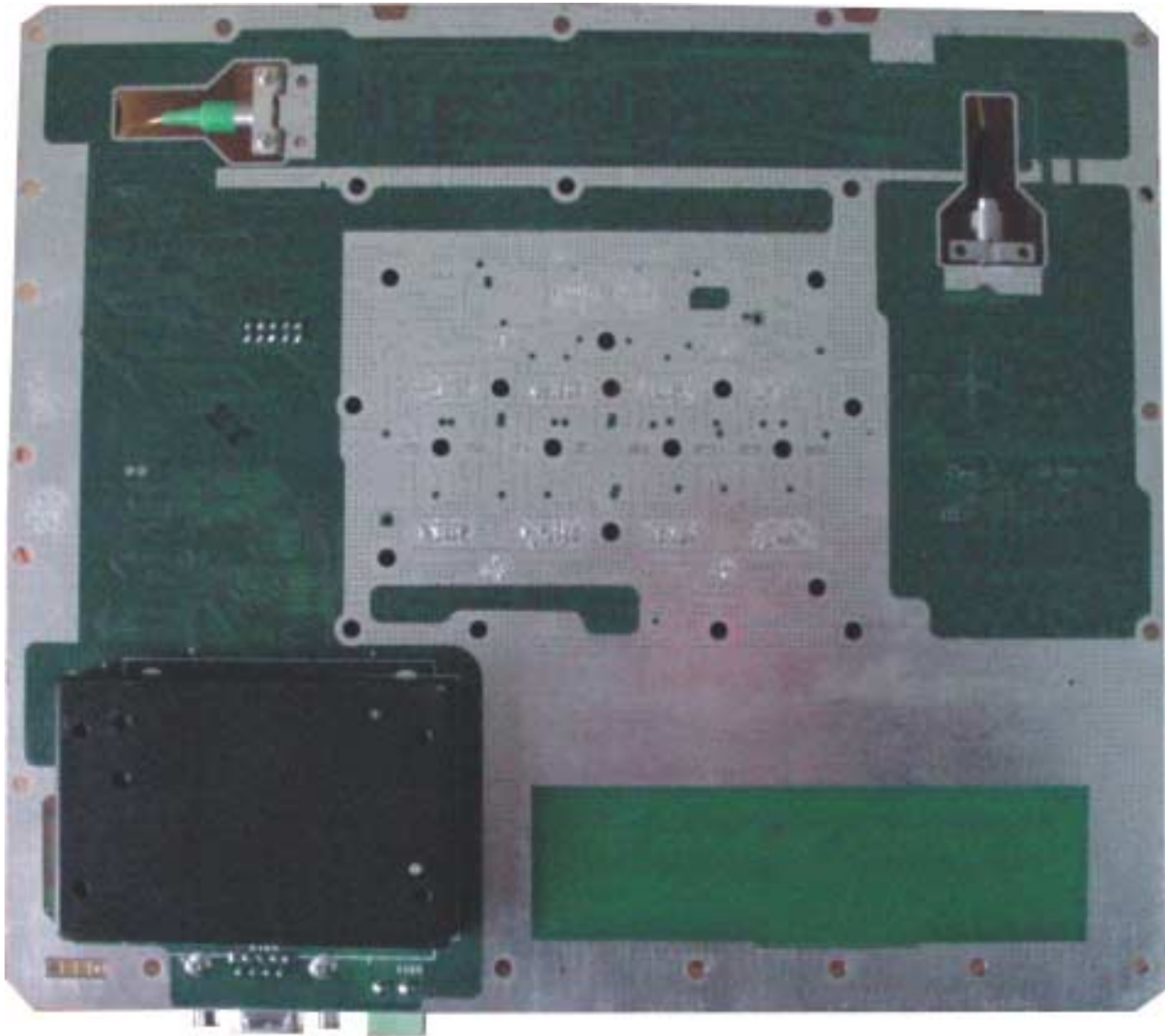
Photograph No.1 Bottom view of the board
