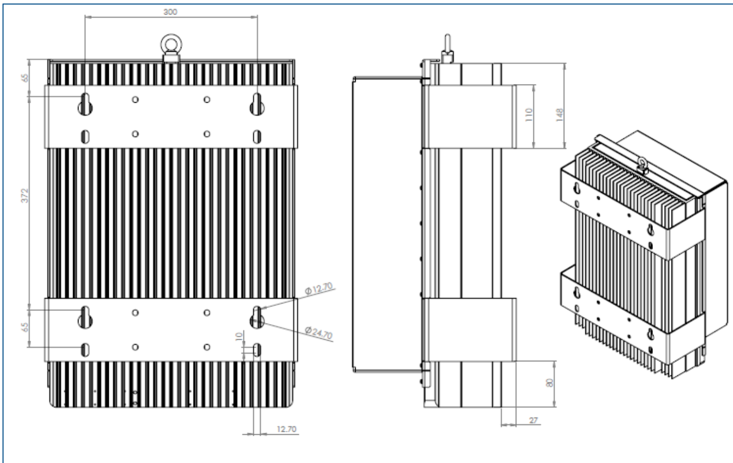
HX Outdoor Bracket Dimensions | Figure 4-2
