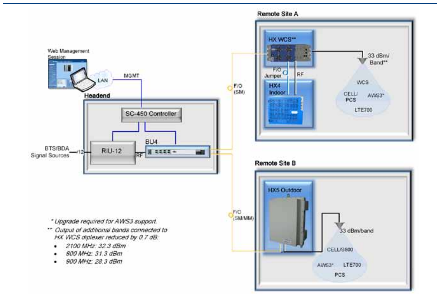
Example of SISO Architecture with HX4 Indoor, HX WCS, and HX5 Outdoor
