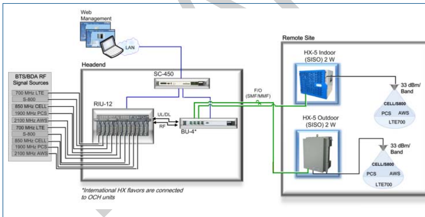
Example of Indoor/ Outdoor SISO Architecture with HX-5
