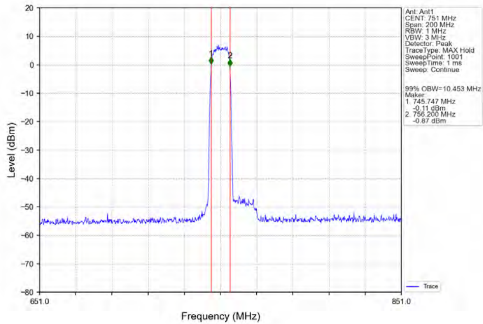
Band13_751MHz_Broad100MHz_SISO_Ant1_NTNV_Output_AGC+3
