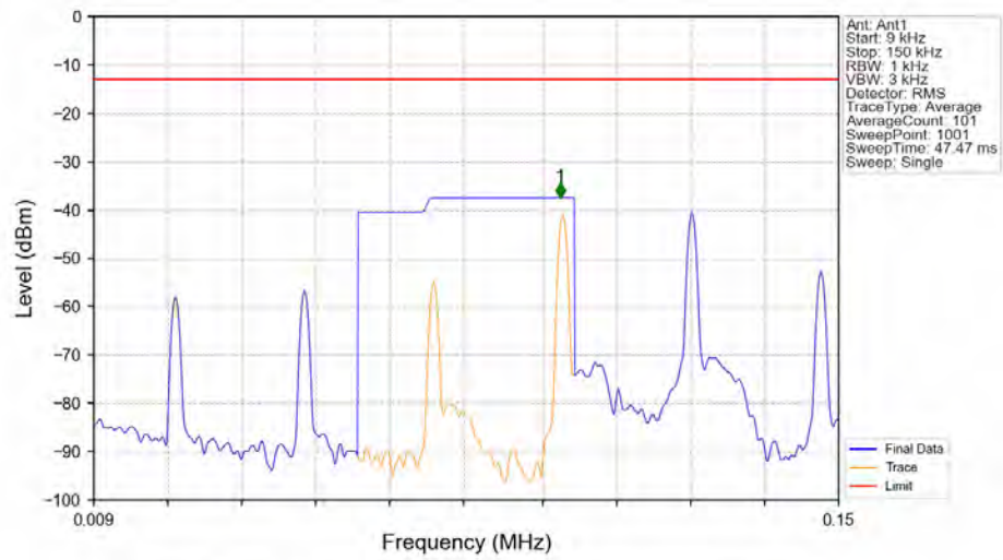
Band13_753.5MHz_AWGN_SISO_Ant1_NTNV
