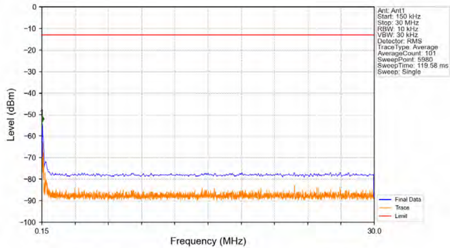
Band13_753.5MHz_AWGN_SISO_Ant1_NTNV
