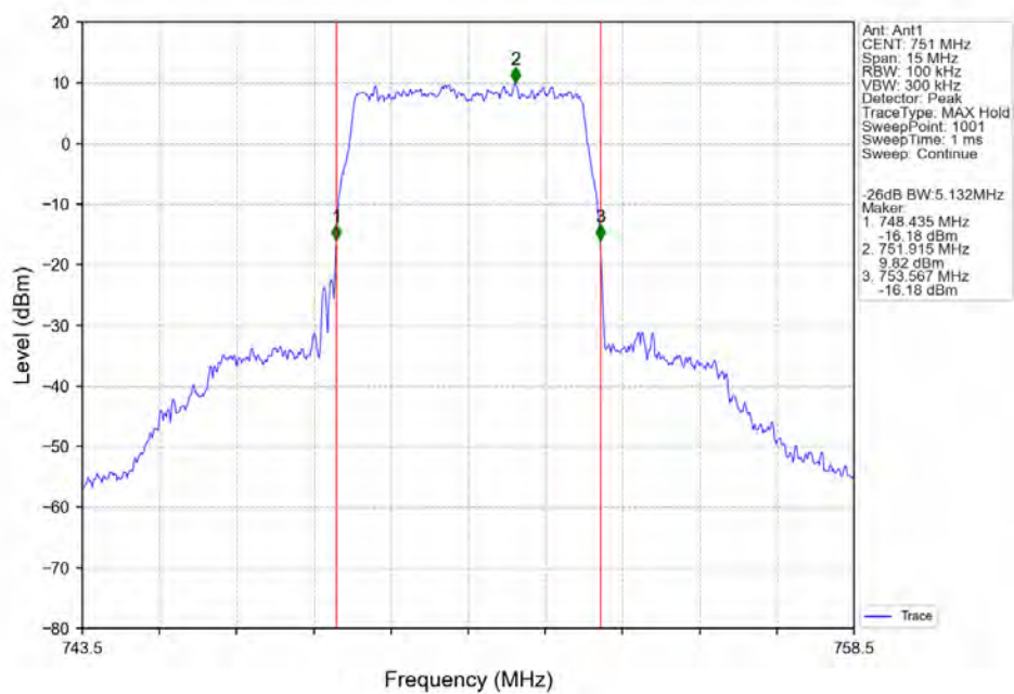
Band13_751MHz_AWGN_SISO_Ant1_NTNV_Output_AGC+3
