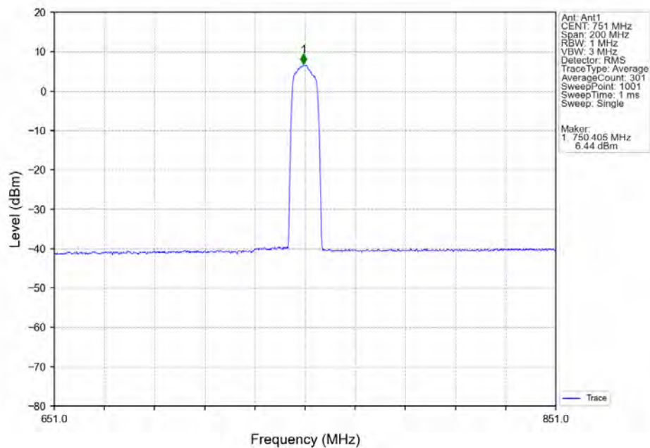
Band13_751MHz_Broad100MHz_SISO_Ant1_NTNV_AGC+3
