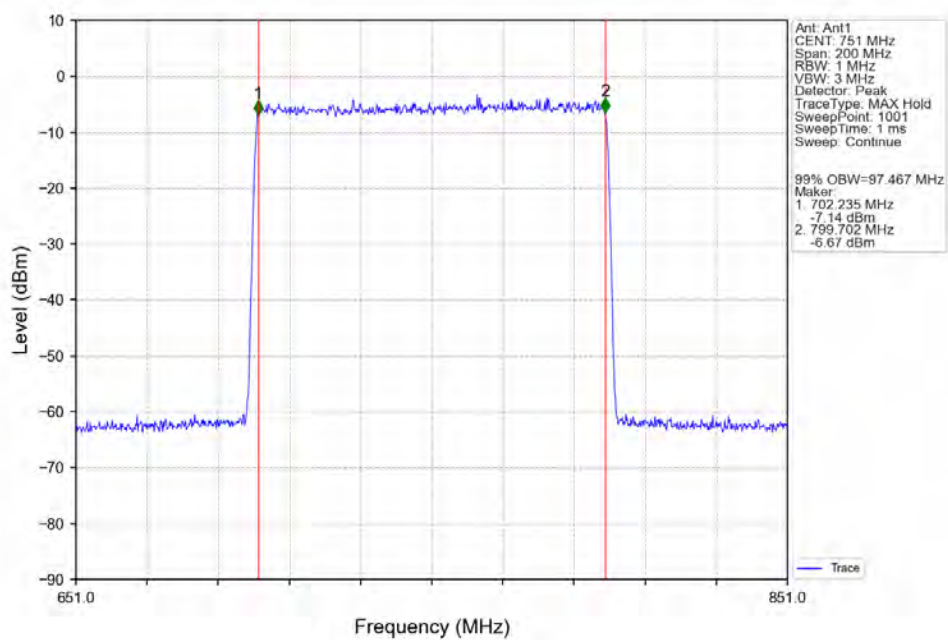
Band13_751MHz_Broad100MHz_SISO_Ant1_NTNV_Input_AGC+3
