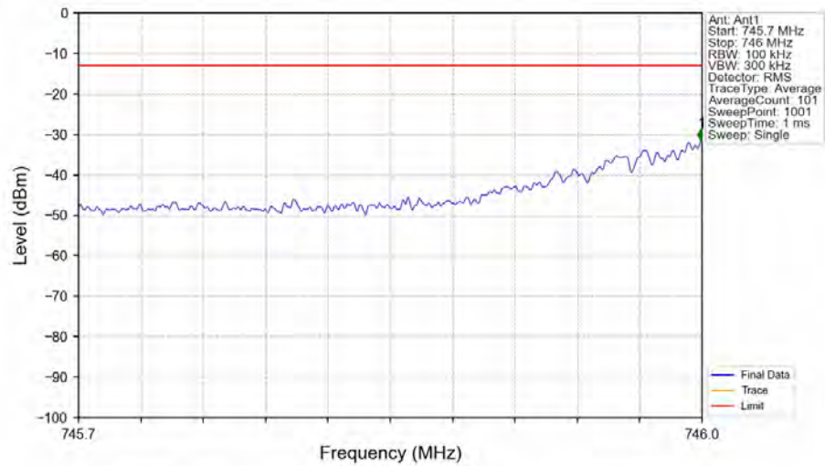
Band13_748.5MHz_AWGN_SISO_Ant1_NTNV_AGC+3
