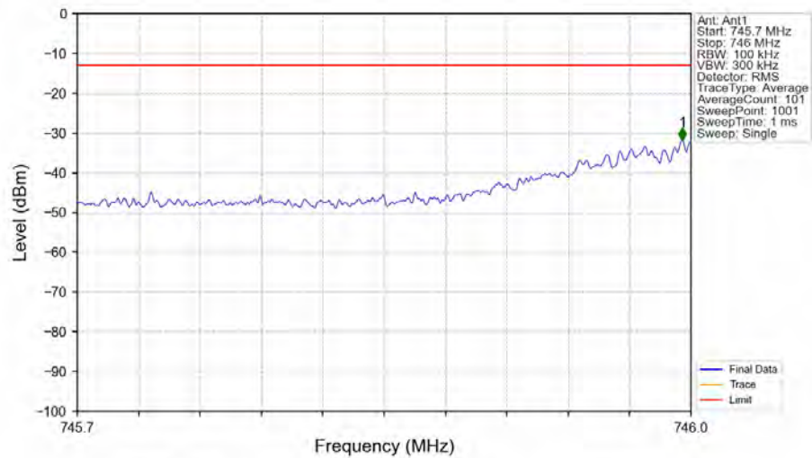
Band13_748.5MHz_AWGN_SISO_Ant1_NTNV_AGC
