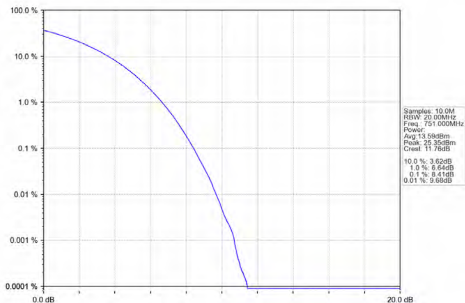
Band13_751MHz_Broad100MHz_SISO_Ant1_NTNV_AGC
